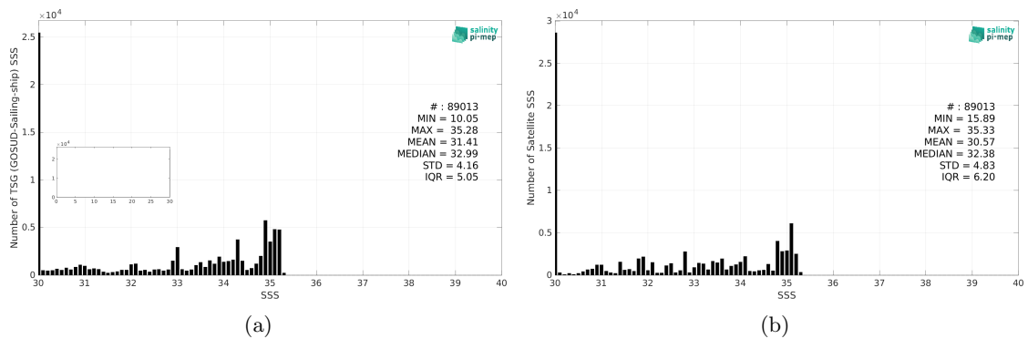
Figure 2: Histograms of SSS from TSG (GOSUD-Sailing-ship) (a) and SMOS SSS L4 v1 - Weekly (CMEMS-CNR) (b) considering all match-up pairs per bins of 0.1 over the Arctic Ocean Pi-MEP region and for the full satellite product period.
