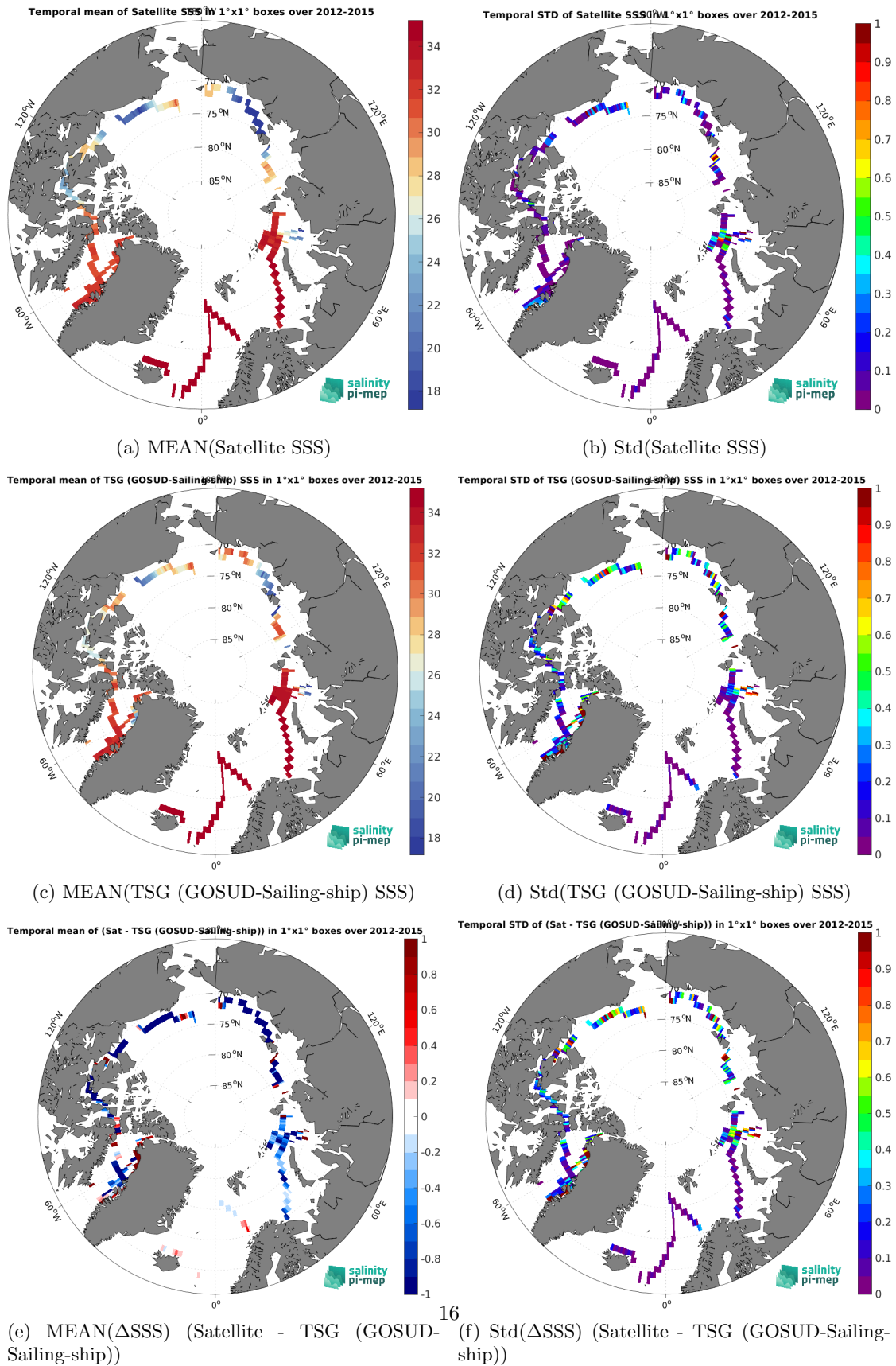
Figure 6: Temporal mean (left) and Std (right) of SSS from SMOS SSS L4 v1 - Weekly (CMEMS-CNR) (top), TSG (GOSUD-Sailing-ship) (middle), and of \Delta SSS (Satellite - TSG (GOSUD-Sailing-ship)). Only match-up pairs are used to generate these maps.
