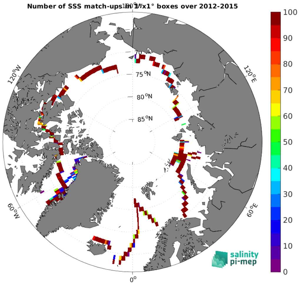
Figure 4: Number of SSS match-ups between TSG (GOSUD-Sailing-ship) SSS and the SMOS SSS L4 v1 - Weekly (CMEMS-CNR) SSS product for the Arctic Ocean Pi-MEP region over 1^\circ \times 1^\circ boxes and for the full satellite product period.
