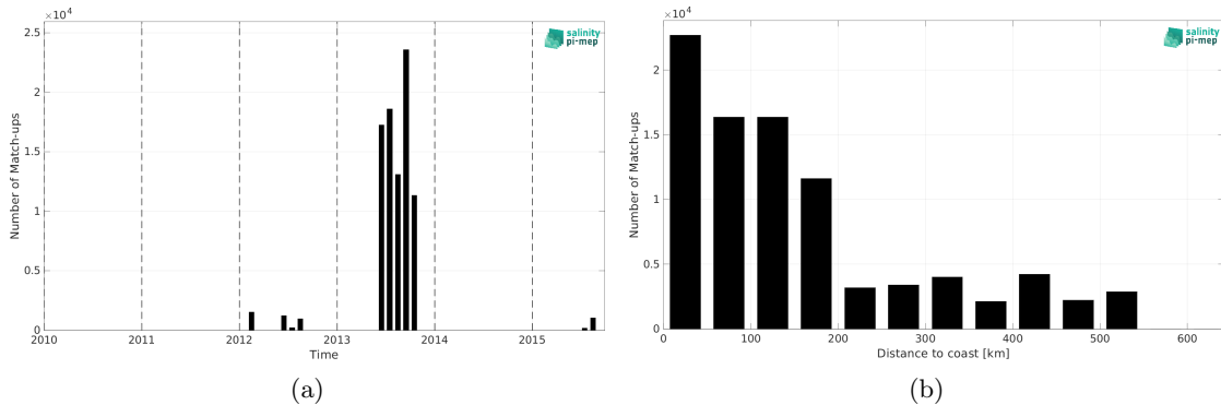
Figure 1: Number of match-ups between TSG (GOSUD-Sailing-ship) and SMOS SSS L4 v1 - Weekly (CMEMS-CNR) SSS as a function of time (a) and as function of the distance to coast (b) over the Arctic Ocean Pi-MEP region and for the full satellite product period.
