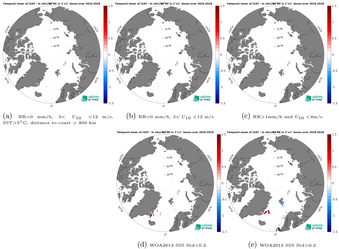
Figure 12: Temporal mean gridded over spatial boxes of size 1^\circ \times 1^\circ of \Delta\text{SSS} (SMOS SSS L4 v1 - Weekly (CMEMS-CNR) - TSG (GOSUD-Research-vessel)) for 5 different subdatasets corresponding to: RR=0 mm/h, 3 < U_{10} < 12 m/s, SST > 5^\circ\text{C} , distance to coast > 800 km (a), RR=0 mm/h, 3 < U_{10} < 12 m/s (b), RR > 1 mm/h and U_{10} < 4 m/s (c), WOA2013 SSS Std < 0.2 (d), WOA2013 SSS Std > 0.2 (e).
