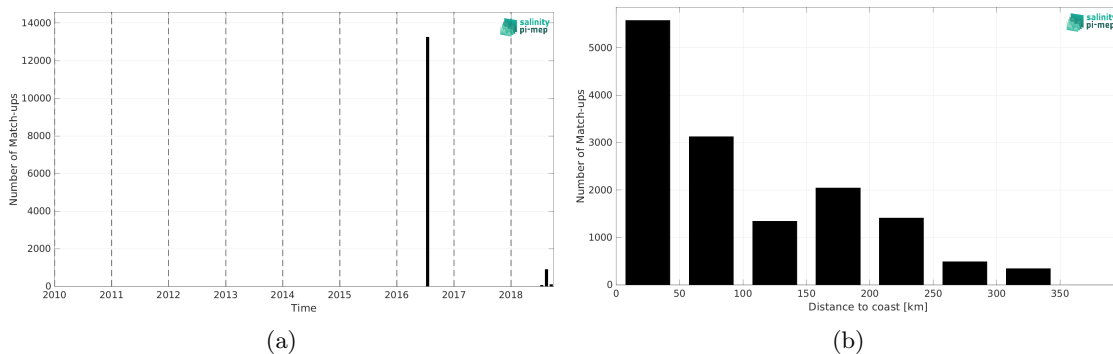
Figure 1: Number of match-ups between TSG (GOSUD-Research-vessel) and SMOS SSS L4 v1 - Weekly (CMEMS-CNR) SSS as a function of time (a) and as function of the distance to coast (b) over the Arctic Ocean Pi-MEP region and for the full satellite product period.
