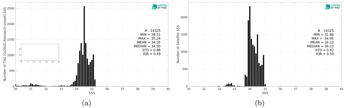
Figure 2: Histograms of SSS from TSG (GOSUD-Research-vessel) (a) and SMOS SSS L4 v1 - Weekly (CMEMS-CNR) (b) considering all match-up pairs per bins of 0.1 over the Arctic Ocean Pi-MEP region and for the full satellite product period.
