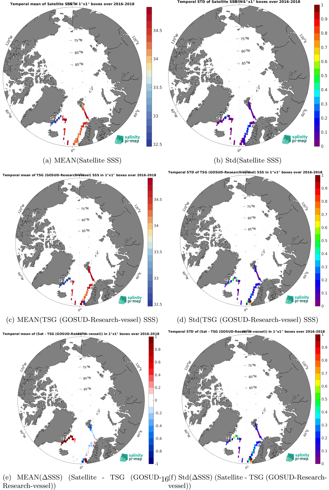
Figure 6: Temporal mean (left) and Std (right) of SSS from SMOS SSS L4 v1 - Weekly (CMEMS-CNR) (top), TSG (GOSUD-Research-vessel) (middle), and of \Delta SSS (Satellite - TSG (GOSUD-Research-vessel)). Only match-up pairs are used to generate these maps.
