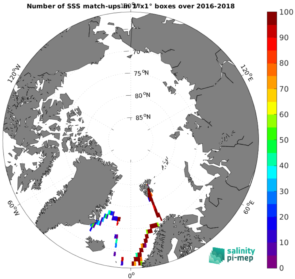
Figure 4: Number of SSS match-ups between TSG (GOSUD-Research-vessel) SSS and the SMOS SSS L4 v1 - Weekly (CMEMS-CNR) SSS product for the Arctic Ocean Pi-MEP region over 1^\circ \times 1^\circ boxes and for the full satellite product period.
