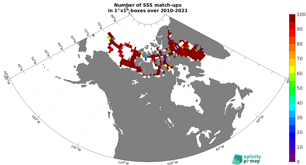
Figure 4: Number of SSS match-ups between TSG (Amundsen) SSS and the SMOS SSS L4 v1 - Weekly (CMEMS-CNR) SSS product for the Arctic Ocean Pi-MEP region over 1^\circ \times 1^\circ boxes and for the full satellite product period.
