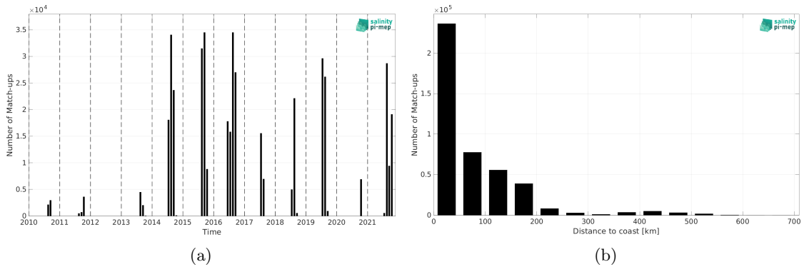
Figure 1: Number of match-ups between TSG (Amundsen) and SMOS SSS L4 v1 - Weekly (CMEMS-CNR) SSS as a function of time (a) and as function of the distance to coast (b) over the Arctic Ocean Pi-MEP region and for the full satellite product period.
