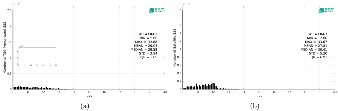
Figure 2: Histograms of SSS from TSG (Amundsen) (a) and SMOS SSS L4 v1 - Weekly (CMEMS-CNR) (b) considering all match-up pairs per bins of 0.1 over the Arctic Ocean Pi-MEP region and for the full satellite product period.
