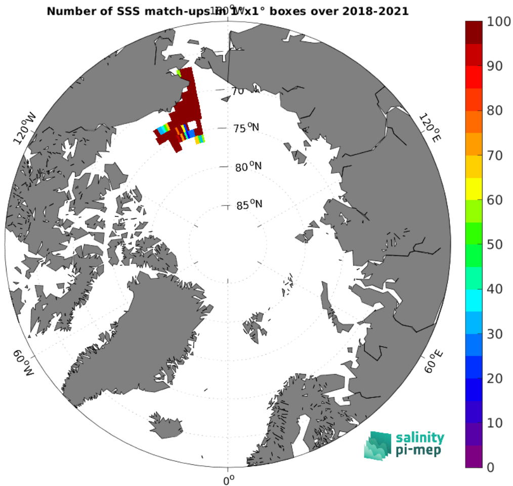
Figure 4: Number of SSS match-ups between Saildrone SSS and the SMOS SSS L4 v1 - Weekly (CMEMS-CNR) SSS product for the Arctic Ocean Pi-MEP region over 1^{\circ} \times 1^{\circ} boxes and for the full satellite product period.
