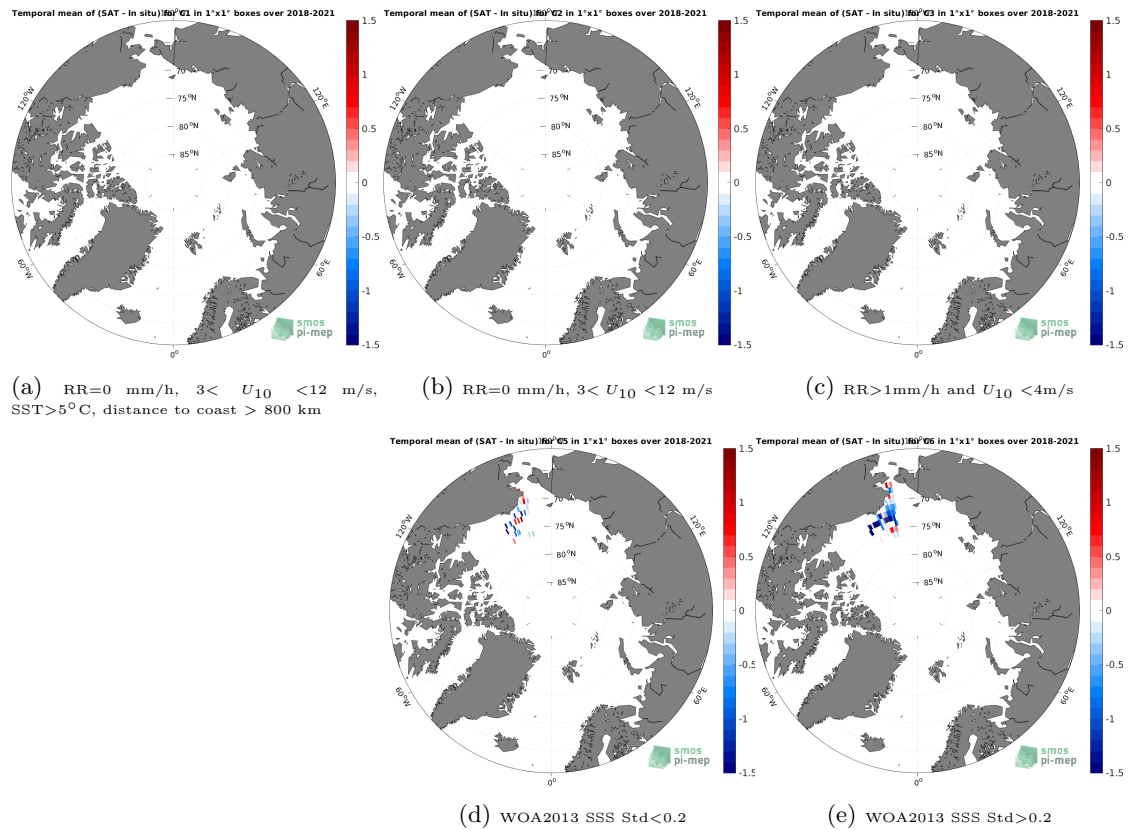
Figure 12: Temporal mean gridded over spatial boxes of size 1^{\circ}\times 1^{\circ} of \Delta\text{SSS} (SMOS SSS L4 v1 - Weekly (CMEMS-CNR) - Saildrone) for 5 different subdatasets corresponding to:RR=0 mm/h, 3 < U_{10} < 12 m/s, SST >5^{\circ}\text{C} , distance to coast > 800 km (a), RR=0 mm/h, 3 < U_{10} < 12 m/s (b), RR >1 mm/h and U_{10} < 4 m/s (c), WOA2013 SSS Std <0.2 (d), WOA2013 SSS Std >0.2 (e).
