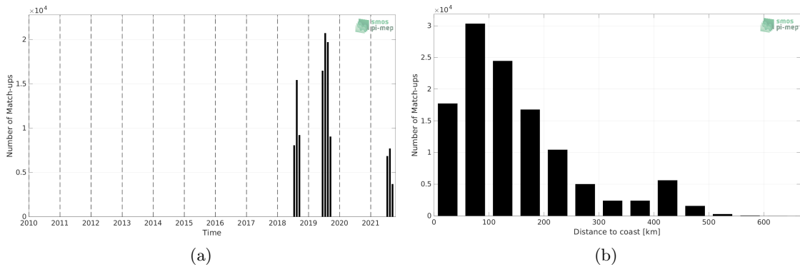
Figure 1: Number of match-ups between Saildrone and SMOS SSS L4 v1 - Weekly (CMEMS-CNR) SSS as a function of time (a) and as function of the distance to coast (b) over the Arctic Ocean Pi-MEP region and for the full satellite product period.
