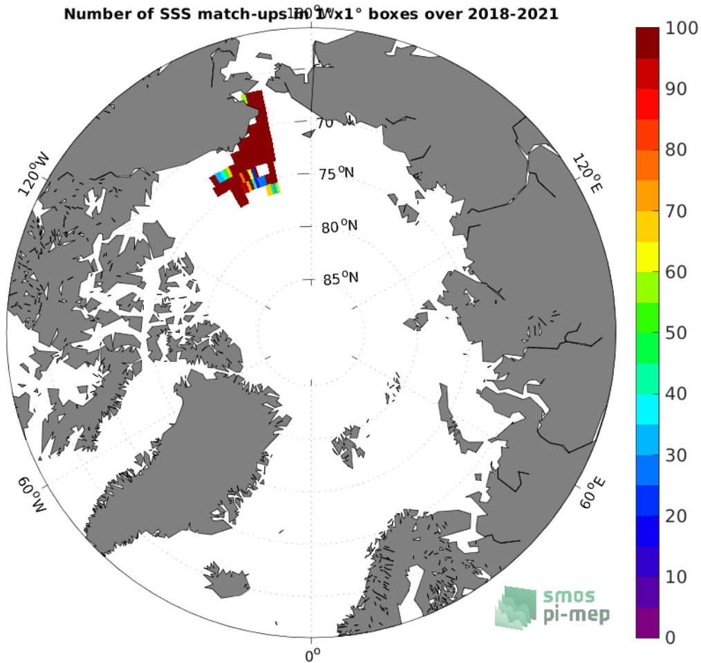
Figure 4: Number of SSS match-ups between Saildrone SSS and the SMOS SSS L4 v1 - Weekly (CMEMS-CNR) SSS product for the Arctic Ocean Pi-MEP region over 1^\circ \times 1^\circ boxes and for the full satellite product period.
