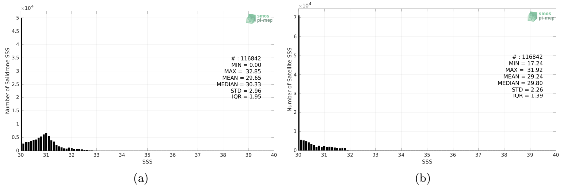
Figure 2: Histograms of SSS from Saildrone (a) and SMOS SSS L4 v1 - Weekly (CMEMS-CNR) (b) considering all match-up pairs per bins of 0.1 over the Arctic Ocean Pi-MEP region and for the full satellite product period.
