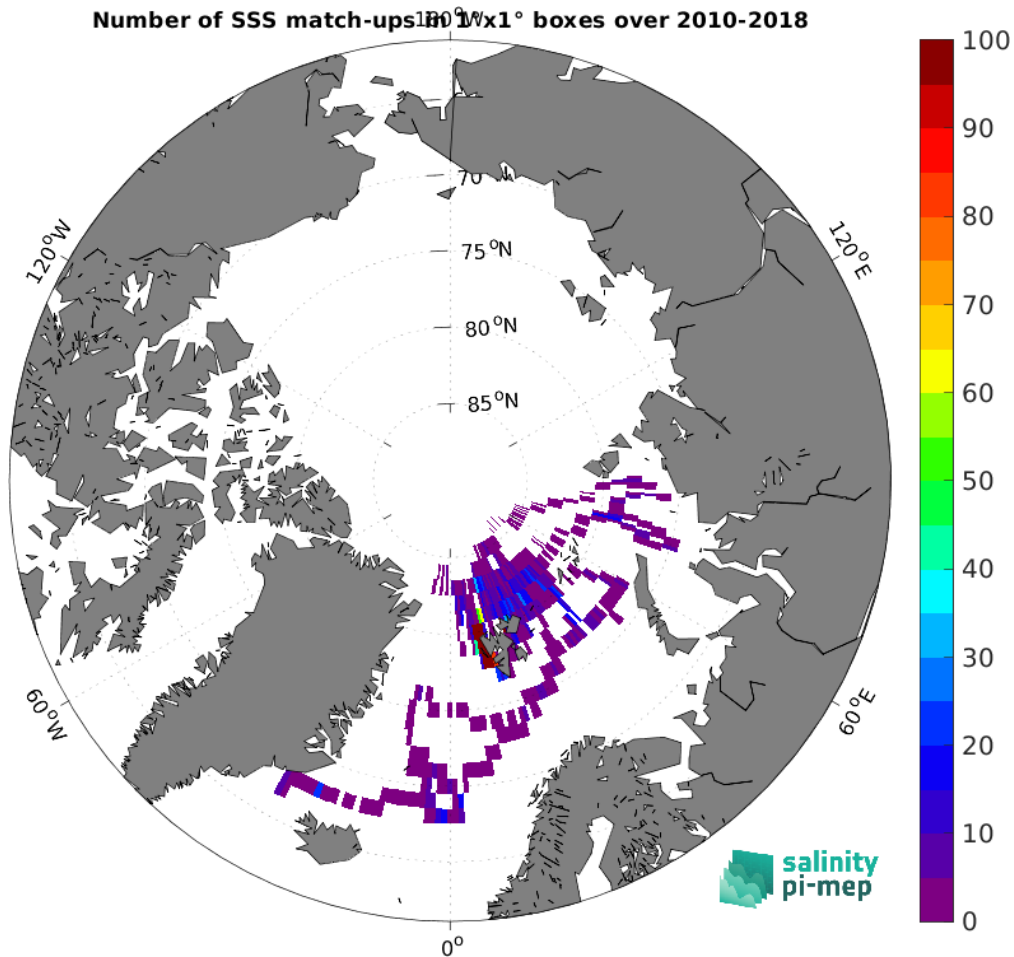
Figure 4: Number of SSS match-ups between Marine mammals SSS and the SMOS SSS L4 v1 - Weekly (CMEMS-CNR) SSS product for the Arctic Ocean Pi-MEP region over 1^\circ \times 1^\circ boxes and for the full satellite product period.
