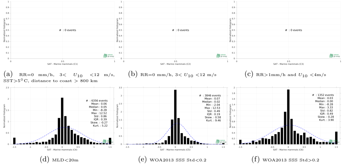
Figure 13: Normalized histogram of \Delta SSS (SMOS SSS L4 v1 - Weekly (CMEMS-CNR) - Marine mammals) for 6 different subdatasets corresponding to: RR=0 mm/h, 3 < U_{10} < 12 m/s, SST > 5°C, distance to coast > 800 km (a), RR=0 mm/h, 3 < U_{10} < 12 m/s (b), RR > 1mm/h and U_{10} < 4 m/s (c), MLD < 20m (d), WOA2013 SSS Std < 0.2 (e), WOA2013 SSS Std > 0.2 (f).
