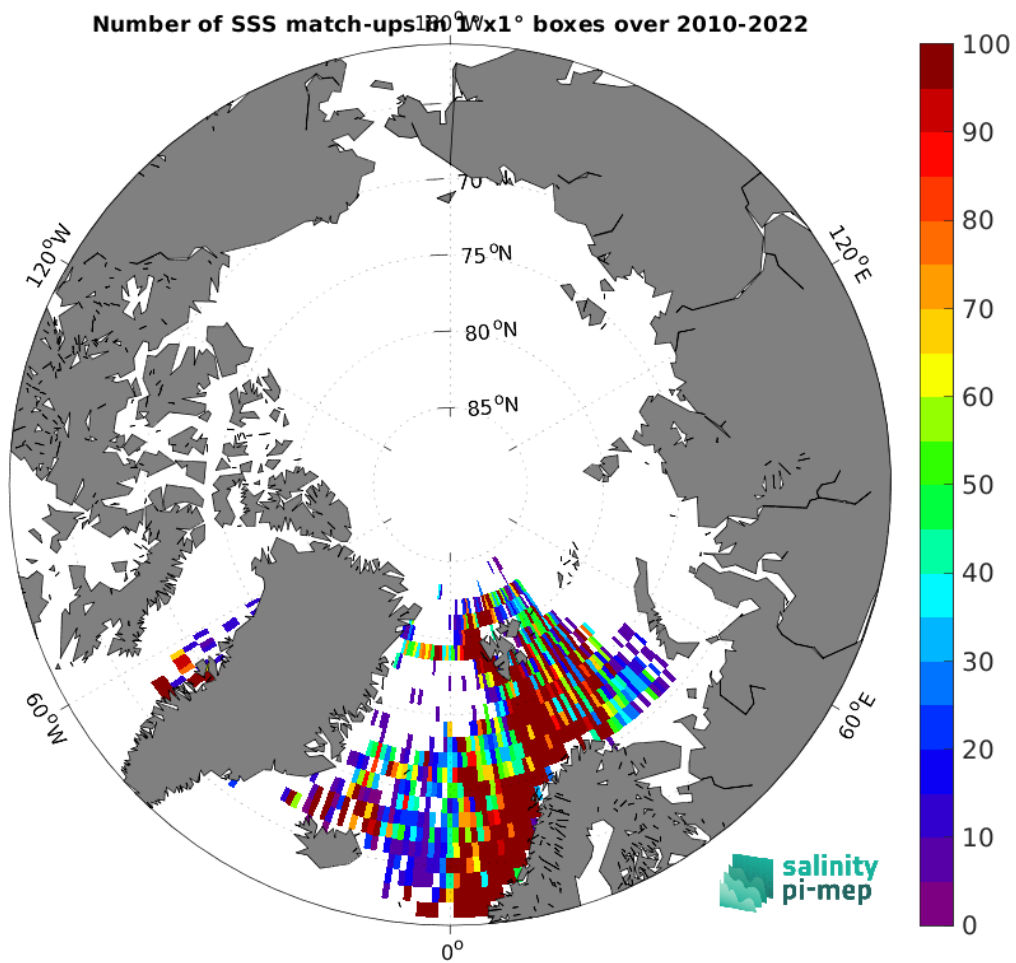
Figure 4: Number of SSS match-ups between ICES SSS and the SMOS SSS L4 v1 - Weekly (CMEMS-CNR) SSS product for the Arctic Ocean Pi-MEP region over 1^\circ \times 1^\circ boxes and for the full satellite product period.
