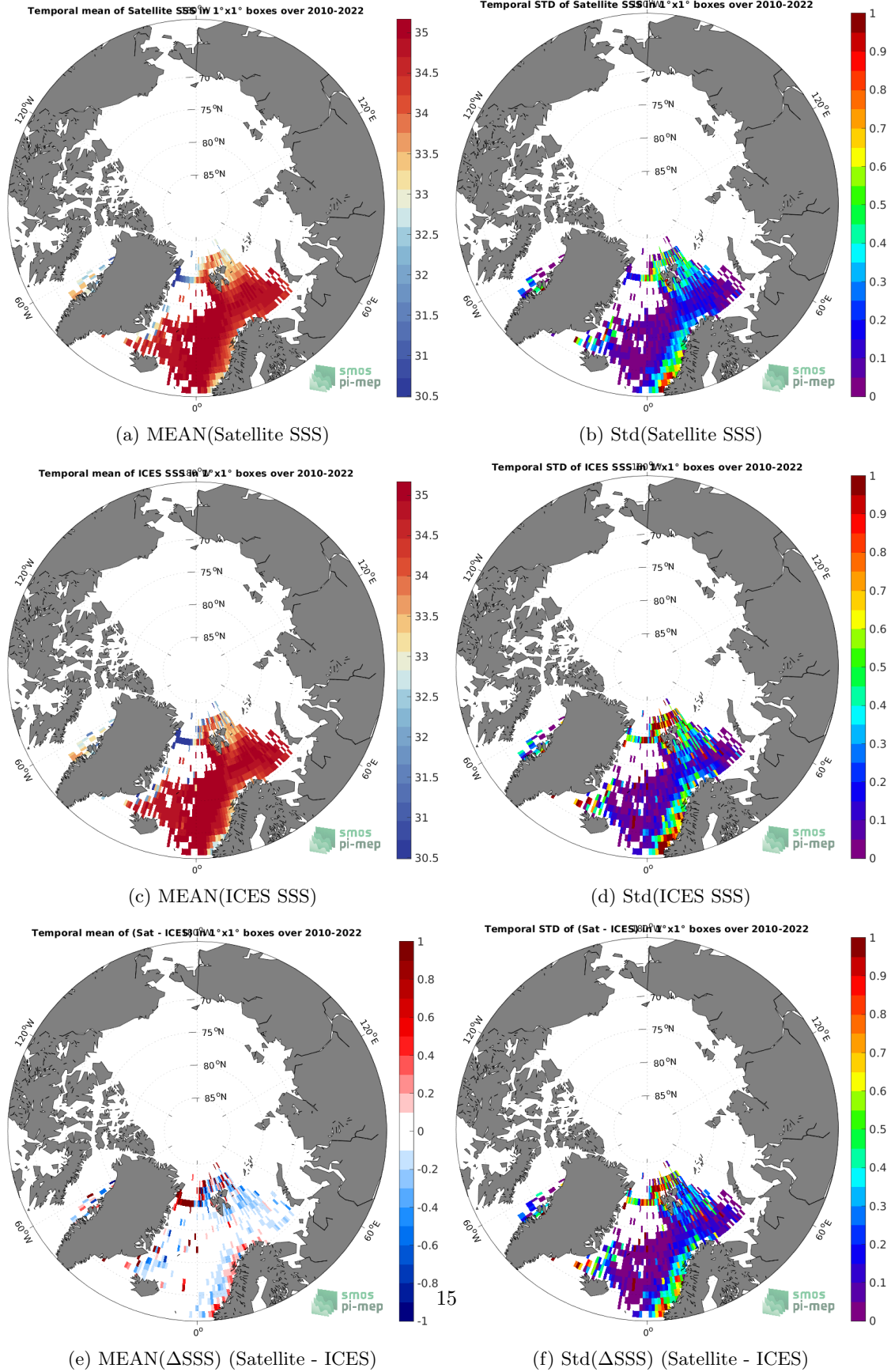
Figure 6: Temporal mean (left) and Std (right) of SSS from SMOS SSS L4 v1 - Weekly (CMEMS-CNR) (top), ICES (middle), and of \Delta SSS (Satellite - ICES). Only match-up pairs are used to generate these maps.
