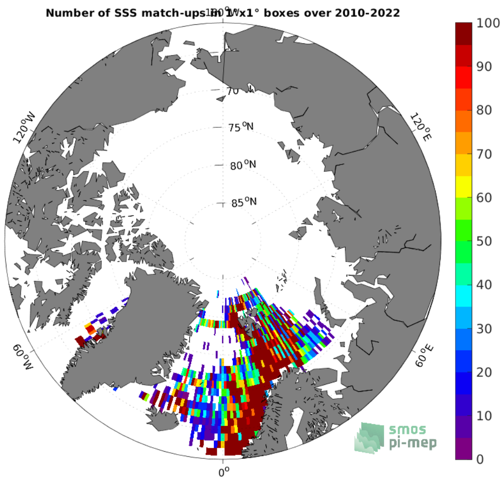
Figure 4: Number of SSS match-ups between ICES SSS and the SMOS SSS L4 v1 - Weekly (CMEMS-CNR) SSS product for the Arctic Ocean Pi-MEP region over 1^{\circ} \times 1^{\circ} boxes and for the full satellite product period.
