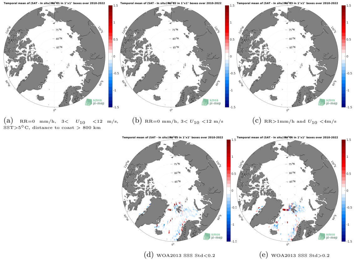
Figure 12: Temporal mean gridded over spatial boxes of size 1^{\circ}\times 1^{\circ} of \Delta\text{SSS} (SMOS SSS L4 v1 - Weekly (CMEMS-CNR) - ICES) for 5 different subdatasets corresponding to:RR=0 mm/h, 3 < U_{10} < 12 m/s, SST > 5^{\circ}\text{C} , distance to coast > 800 km (a), RR=0 mm/h, 3 < U_{10} < 12 m/s (b), RR > 1 mm/h and U_{10} < 4 m/s (c), WOA2013 SSS Std < 0.2 (d), WOA2013 SSS Std > 0.2 (e).
