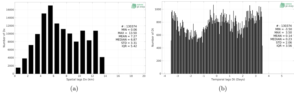
Figure 5: Histograms of the spatial (a) and temporal (b) lags between the location/time of the ICES measurement and the date of the corresponding SMOS SSS L4 v1 - Weekly (CMEMS-CNR) SSS pixel.
