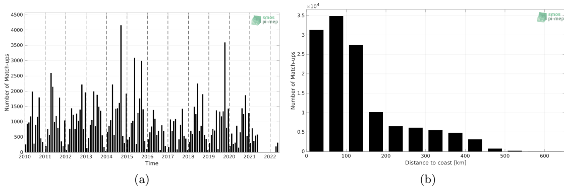
Figure 1: Number of match-ups between ICES and SMOS SSS L4 v1 - Weekly (CMEMS-CNR) SSS as a function of time (a) and as function of the distance to coast (b) over the Arctic Ocean Pi-MEP region and for the full satellite product period.
