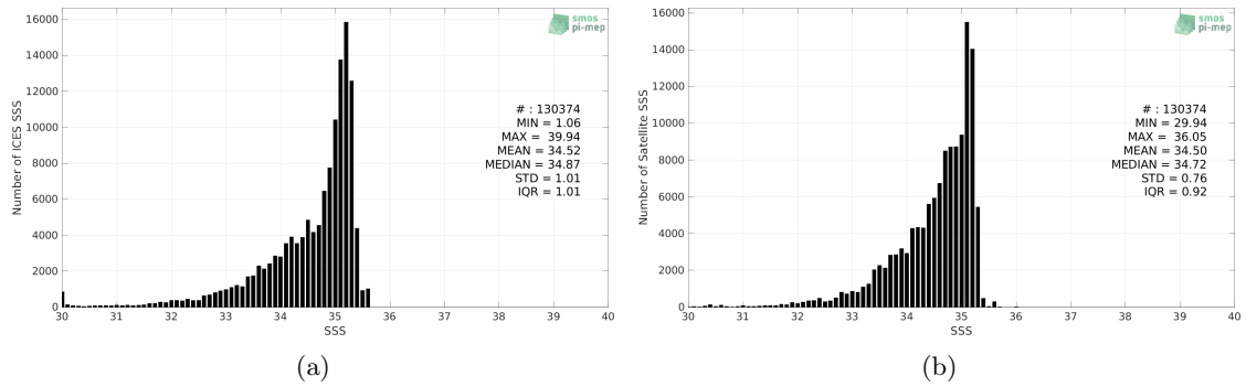
Figure 2: Histograms of SSS from ICES (a) and SMOS SSS L4 v1 - Weekly (CMEMS-CNR) (b) considering all match-up pairs per bins of 0.1 over the Arctic Ocean Pi-MEP region and for the full satellite product period.
