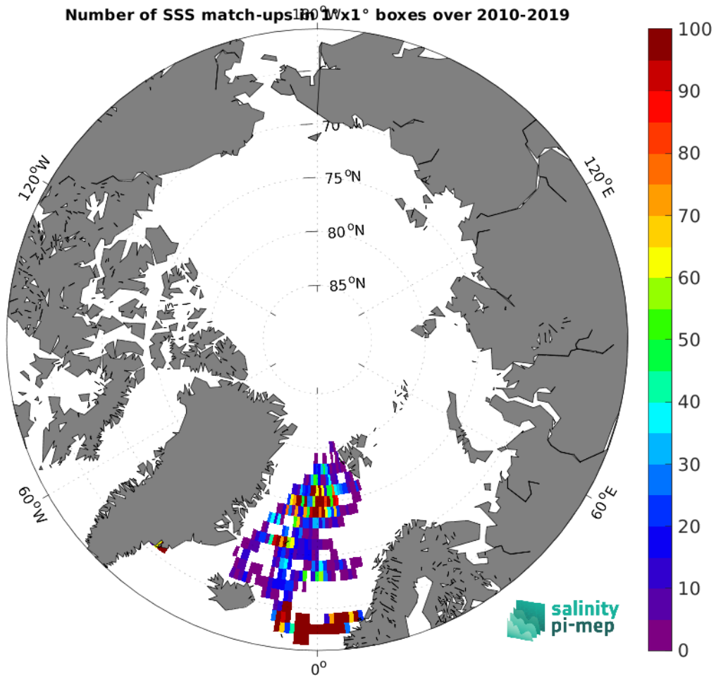
Figure 3: Number of SSS match-ups between Surface drifters SSS and the SMOS SSS L4 v1 - Weekly (CMEMS-CNR) SSS product for the Arctic Ocean Pi-MEP region over 1^{\circ} \times 1^{\circ} boxes and for the full satellite product period.
