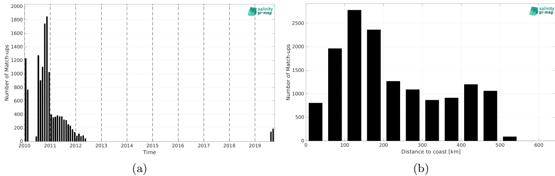
Figure 1: Number of match-ups between Surface drifters and SMOS SSS L4 v1 - Weekly (CMEMS-CNR) SSS as a function of time (a) and as function of the distance to coast (b) over the Arctic Ocean Pi-MEP region and for the full satellite product period.
