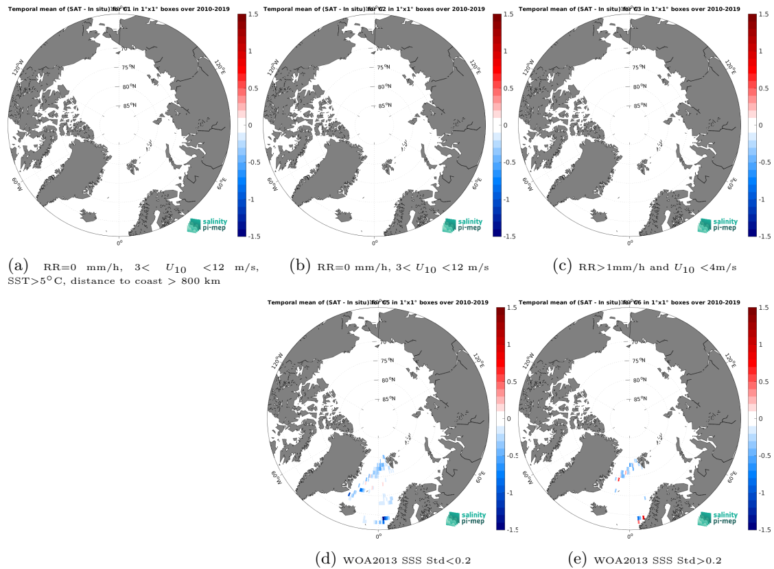
Figure 11: Temporal mean gridded over spatial boxes of size 1^{\circ}\times 1^{\circ} of \Delta\text{SSS} (SMOS SSS L4 v1 - Weekly (CMEMS-CNR) - Surface drifters) for 5 different subdatasets corresponding to:RR=0 mm/h, 3 < U_{10} < 12 m/s, SST >5^{\circ}\text{C} , distance to coast > 800 km (a), RR=0 mm/h, 3 < U_{10} < 12 m/s (b), RR >1 mm/h and U_{10} < 4 m/s (c), WOA2013 SSS Std <0.2 (d), WOA2013 SSS Std >0.2 (e).
