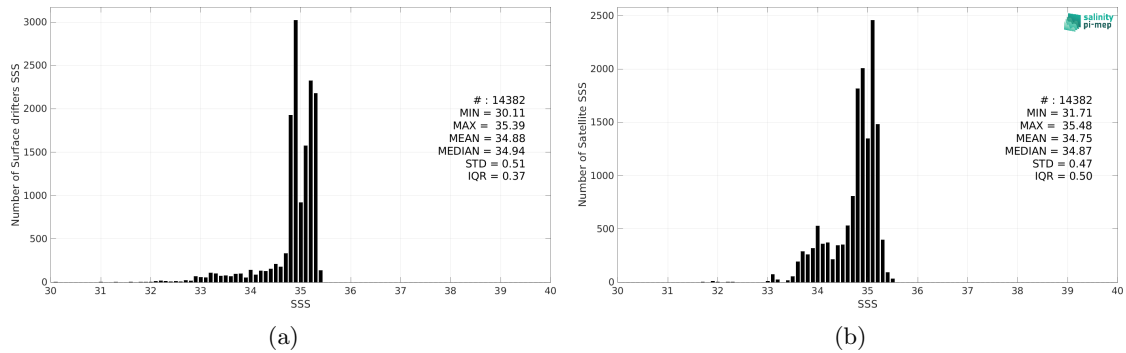
Figure 2: Histograms of SSS from Surface drifters (a) and SMOS SSS L4 v1 - Weekly (CMEMS-CNR) (b) considering all match-up pairs per bins of 0.1 over the Arctic Ocean Pi-MEP region and for the full satellite product period.
