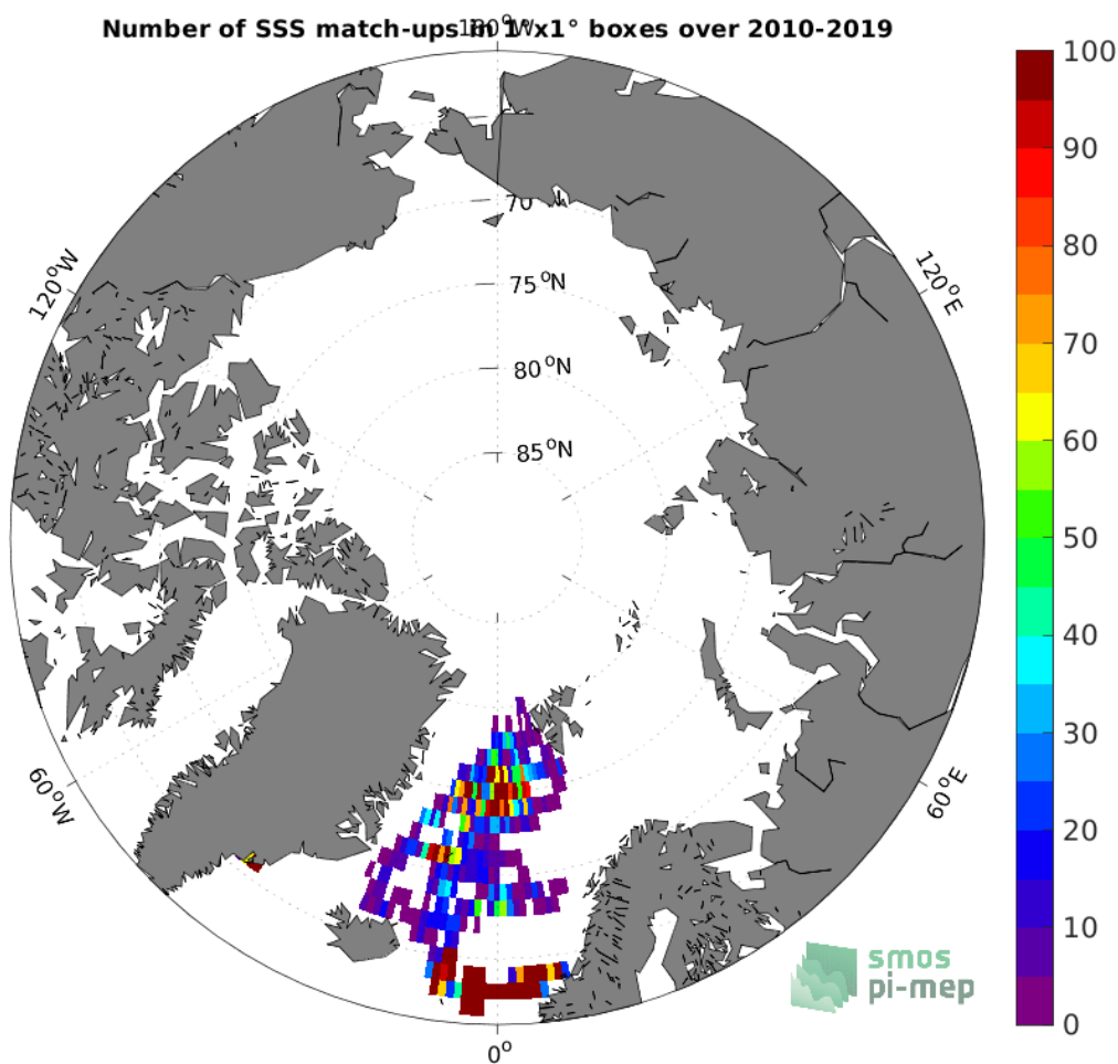
Figure 3: Number of SSS match-ups between Surface drifters SSS and the SMOS SSS L4 v1 - Weekly (CMEMS-CNR) SSS product for the Arctic Ocean Pi-MEP region over 1^\circ \times 1^\circ boxes and for the full satellite product period.
