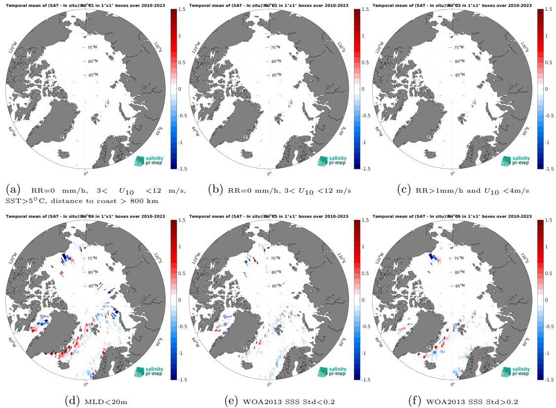
Figure 12: Temporal mean gridded over spatial boxes of size 1^{\circ}\times 1^{\circ} of \Delta\text{SSS} (SMOS SSS L4 v1 - Weekly (CMEMS-CNR) - Argo) for 6 different subdatasets corresponding to: RR=0 mm/h, 3 < U_{10} < 12 m/s, SST > 5^{\circ}\text{C} , distance to coast > 800 km (a), RR=0 mm/h, 3 < U_{10} < 12 m/s (b), RR > 1 mm/h and U_{10} < 4 m/s (c), MLD < 20 m (d), WOA2013 SSS Std < 0.2 (e), WOA2013 SSS Std > 0.2 (f).
