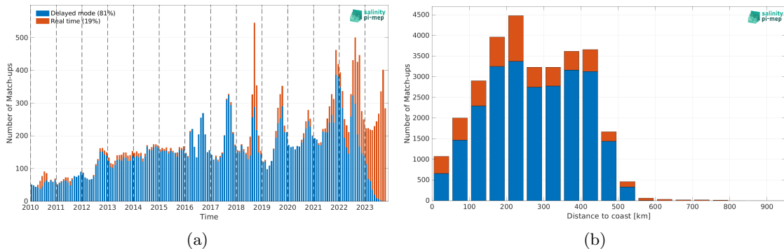
Figure 1: Number of match-ups between Argo and SMOS SSS L4 v1 - Weekly (CMEMS-CNR) SSS as a function of time (a) and as function of the distance to coast (b) over the Arctic Ocean Pi-MEP region and for the full satellite product period.
