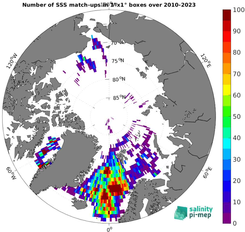
Figure 4: Number of SSS match-ups between Argo SSS and the SMOS SSS L4 v1 - Weekly (CMEMS-CNR) SSS product for the Arctic Ocean Pi-MEP region over 1^\circ \times 1^\circ boxes and for the full satellite product period.
