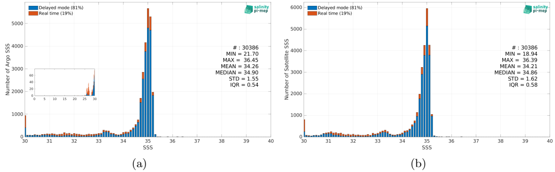
Figure 2: Histograms of SSS from Argo (a) and SMOS SSS L4 v1 - Weekly (CMEMS-CNR) (b) considering all match-up pairs per bins of 0.1 over the Arctic Ocean Pi-MEP region and for the full satellite product period.
