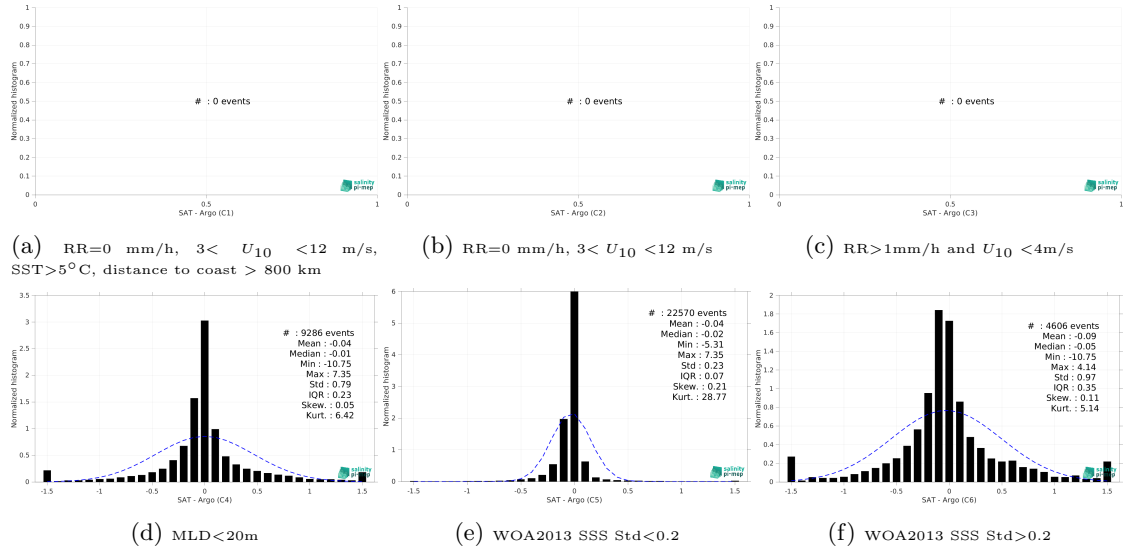
Figure 13: Normalized histogram of \Delta\text{SSS} (SMOS SSS L4 v1 - Weekly (CMEMS-CNR) - Argo) for 6 different subdatasets corresponding to: RR=0 mm/h, 3 < U_{10} < 12 m/s, SST > 5^\circ\text{C} , distance to coast > 800 km (a), RR=0 mm/h, 3 < U_{10} < 12 m/s (b), RR > 1\text{mm/h} and U_{10} < 4\text{m/s} (c), MLD < 20\text{m} (d), WOA2013 SSS Std < 0.2 (e), WOA2013 SSS Std > 0.2 (f).
