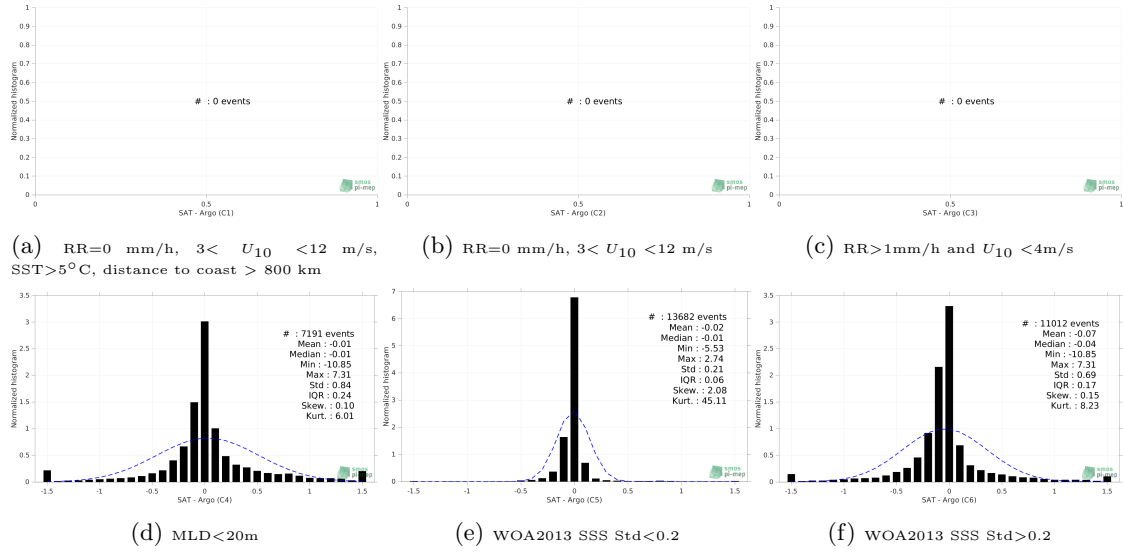
Figure 13: Normalized histogram of \Delta SSS (SMOS SSS L4 v1 - Weekly (CMEMS-CNR) - Argo) for 6 different subdatasets corresponding to: RR=0 mm/h, 3 < U_{10} < 12 m/s, SST > 5°C, distance to coast > 800 km (a), RR=0 mm/h, 3 < U_{10} < 12 m/s (b), RR > 1mm/h and U_{10} < 4 m/s (c), MLD < 20m (d), WOA2013 SSS Std < 0.2 (e), WOA2013 SSS Std > 0.2 (f).
