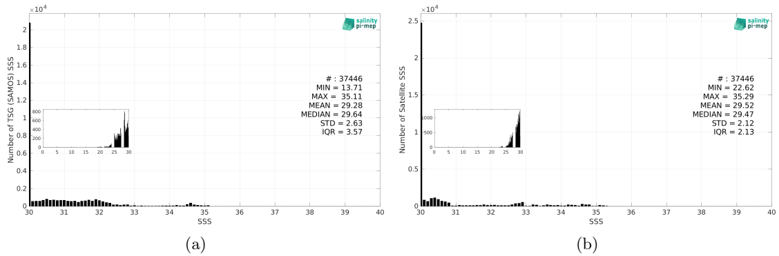
Figure 3: Histograms of SSS from TSG (SAMOS) (a) and SMOS SSS L4 v1 - Monthly (CMEMS-CNR) (b) considering all match-up pairs per bins of 0.1 over the Arctic Ocean Pi-MEP region and for the full satellite product period.
