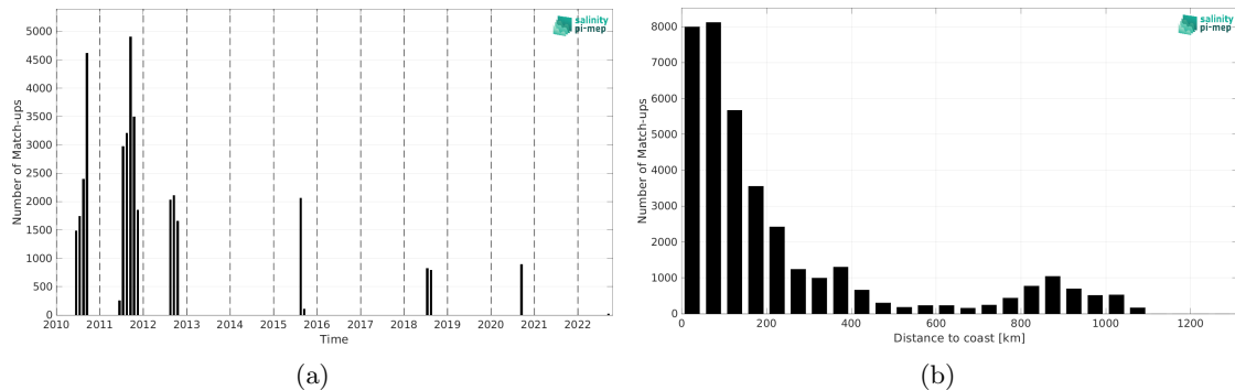
Figure 2: Number of match-ups between TSG (SAMOS) and SMOS SSS L4 v1 - Monthly (CMEMS-CNR) SSS as a function of time (a) and as function of the distance to coast (b) over the Arctic Ocean Pi-MEP region and for the full satellite product period.
