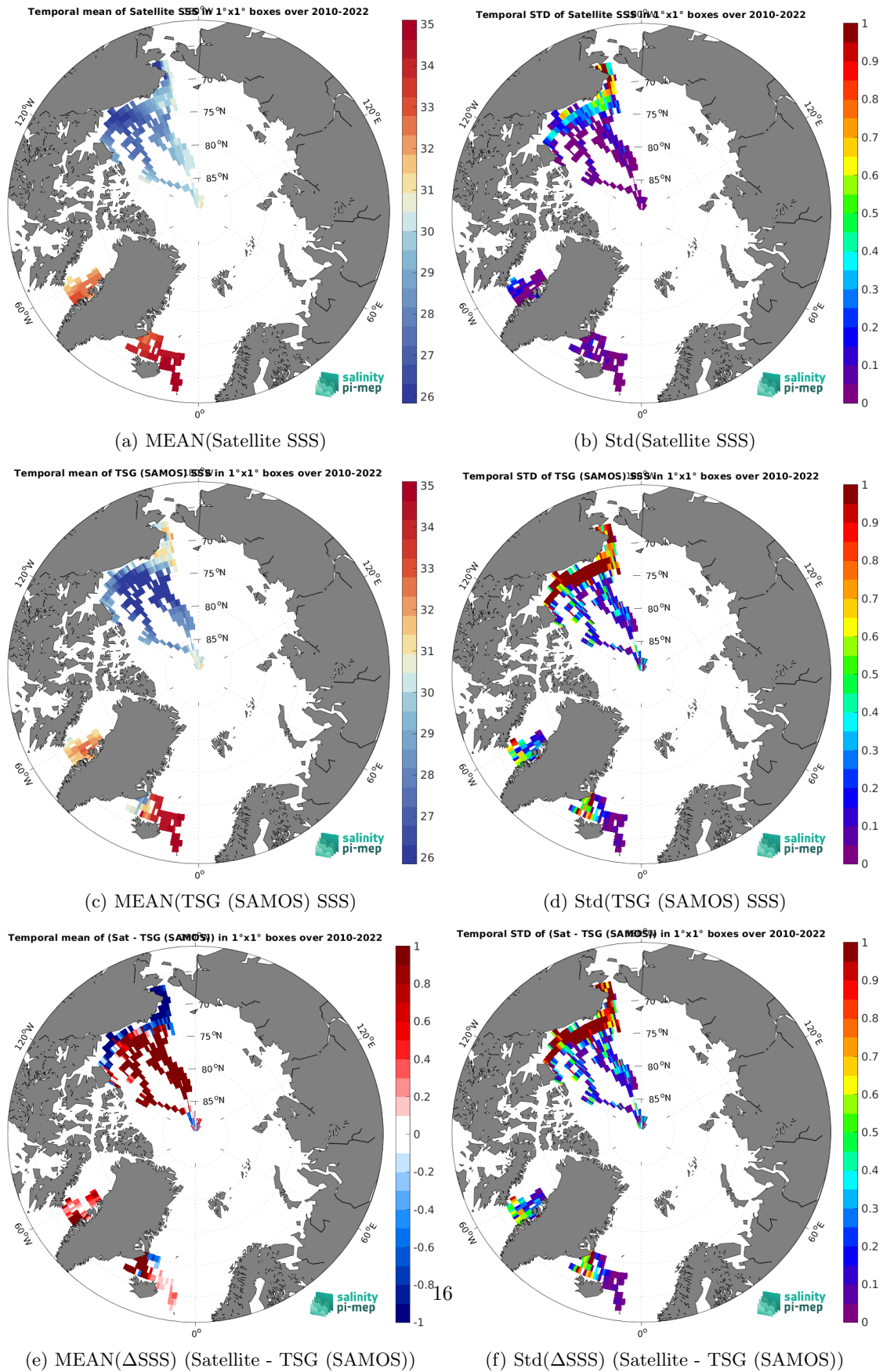
Figure 7: Temporal mean (left) and Std (right) of SSS from SMOS SSS L4 v1 - Monthly (CMEMS-CNR) (top), TSG (SAMOS) (middle), and of \Delta SSS (Satellite - TSG (SAMOS)). Only match-up pairs are used to generate these maps.
