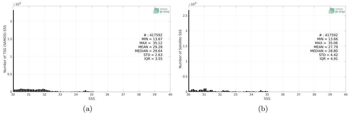
Figure 2: Histograms of SSS from TSG (SAMOS) (a) and SMOS SSS L4 v1 - Monthly (CMEMS-CNR) (b) considering all match-up pairs per bins of 0.1 over the Arctic Ocean Pi-MEP region and for the full satellite product period.
