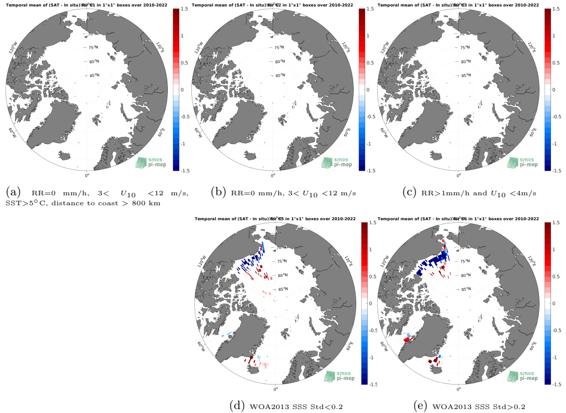
Figure 12: Temporal mean gridded over spatial boxes of size 1^{\circ}\times 1^{\circ} of \Delta\text{SSS} (SMOS SSS L4 v1 - Monthly (CMEMS-CNR) - TSG (SAMOS)) for 5 different subdatasets corresponding to:RR=0 mm/h, 3 < U_{10} < 12 m/s, SST >5^{\circ}\text{C} , distance to coast > 800 km (a), RR=0 mm/h, 3 < U_{10} < 12 m/s (b), RR >1 mm/h and U_{10} < 4 m/s (c), WOA2013 SSS Std <0.2 (d), WOA2013 SSS Std >0.2 (e).
