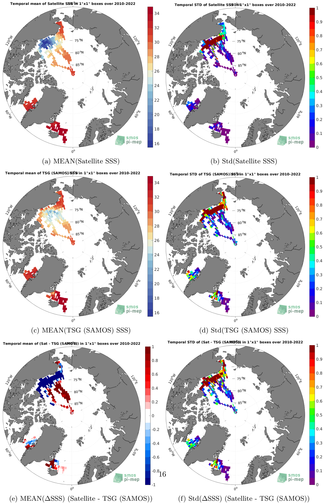
Figure 6: Temporal mean (left) and Std (right) of SSS from SMOS SSS L4 v1 - Monthly (CMEMS-CNR) (top), TSG (SAMOS) (middle), and of \Delta SSS (Satellite - TSG (SAMOS)). Only match-up pairs are used to generate these maps.
