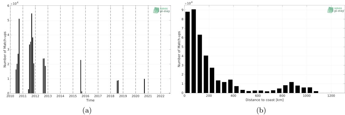
Figure 1: Number of match-ups between TSG (SAMOS) and SMOS SSS L4 v1 - Monthly (CMEMS-CNR) SSS as a function of time (a) and as function of the distance to coast (b) over the Arctic Ocean Pi-MEP region and for the full satellite product period.
