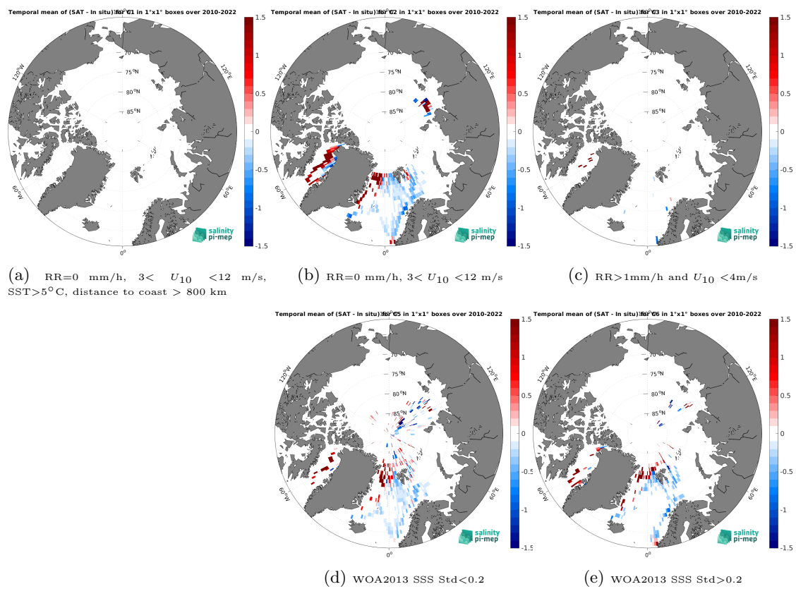
Figure 14: Temporal mean gridded over spatial boxes of size 1^\circ \times 1^\circ of \Delta SSS (SMOS SSS L4 v1 - Monthly (CMEMS-CNR) - TSG (Polarstern)) for 5 different subdatasets corresponding to:RR=0 mm/h, 3 < U_{10} < 12 m/s, SST > 5°C, distance to coast > 800 km (a), RR=0 mm/h, 3 < U_{10} < 12 m/s (b), RR > 1mm/h and U_{10} < 4 m/s (c), WOA2013 SSS Std < 0.2 (d), WOA2013 SSS Std > 0.2 (e).
