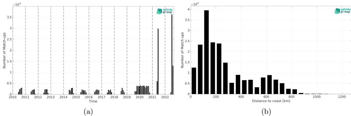
Figure 2: Number of match-ups between TSG (Polarstern) and SMOS SSS L4 v1 - Monthly (CMEMS-CNR) SSS as a function of time (a) and as function of the distance to coast (b) over the Arctic Ocean Pi-MEP region and for the full satellite product period.
