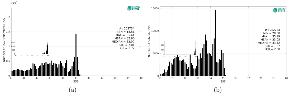
Figure 3: Histograms of SSS from TSG (Polarstern) (a) and SMOS SSS L4 v1 - Monthly (CMEMS-CNR) (b) considering all match-up pairs per bins of 0.1 over the Arctic Ocean Pi-MEP region and for the full satellite product period.
