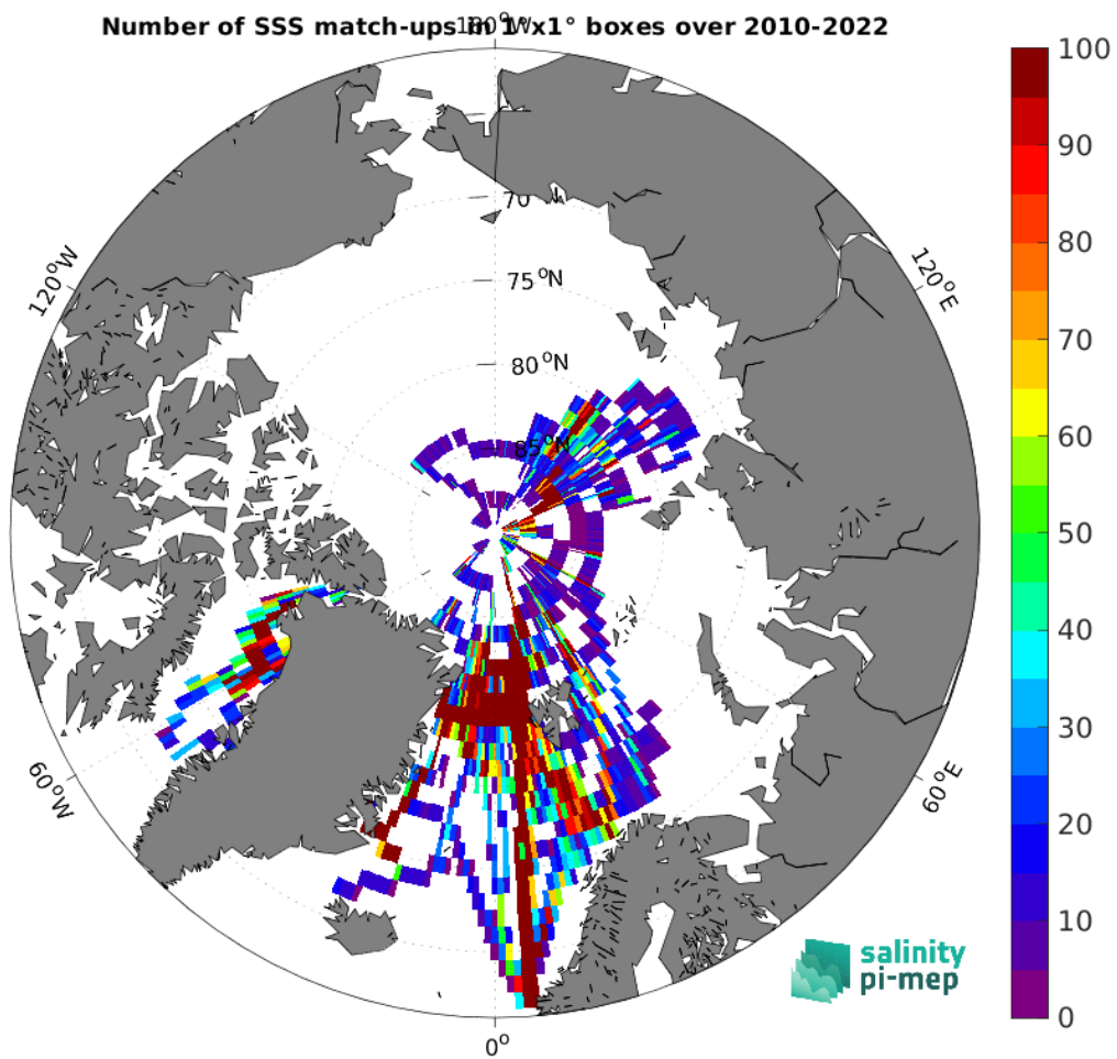
Figure 5: Number of SSS match-ups between TSG (Polarstern) SSS and the SMOS SSS L4 v1 - Monthly (CMEMS-CNR) SSS product for the Arctic Ocean Pi-MEP region over 1^\circ \times 1^\circ boxes and for the full satellite product period.
