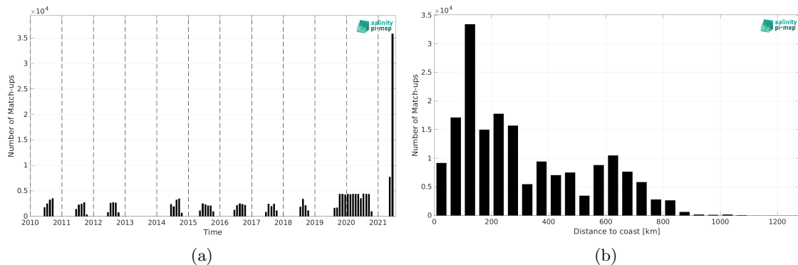
Figure 1: Number of match-ups between TSG (Polarstern) and SMOS SSS L4 v1 - Monthly (CMEMS-CNR) SSS as a function of time (a) and as function of the distance to coast (b) over the Arctic Ocean Pi-MEP region and for the full satellite product period.
