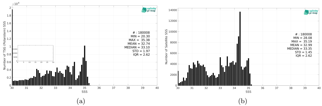
Figure 2: Histograms of SSS from TSG (Polarstern) (a) and SMOS SSS L4 v1 - Monthly (CMEMS-CNR) (b) considering all match-up pairs per bins of 0.1 over the Arctic Ocean Pi-MEP region and for the full satellite product period.
