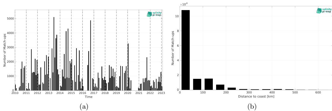
Figure 2: Number of match-ups between TSG (LEGOS-DM) and SMOS SSS L4 v1 - Monthly (CMEMS-CNR) SSS as a function of time (a) and as function of the distance to coast (b) over the Arctic Ocean Pi-MEP region and for the full satellite product period.
