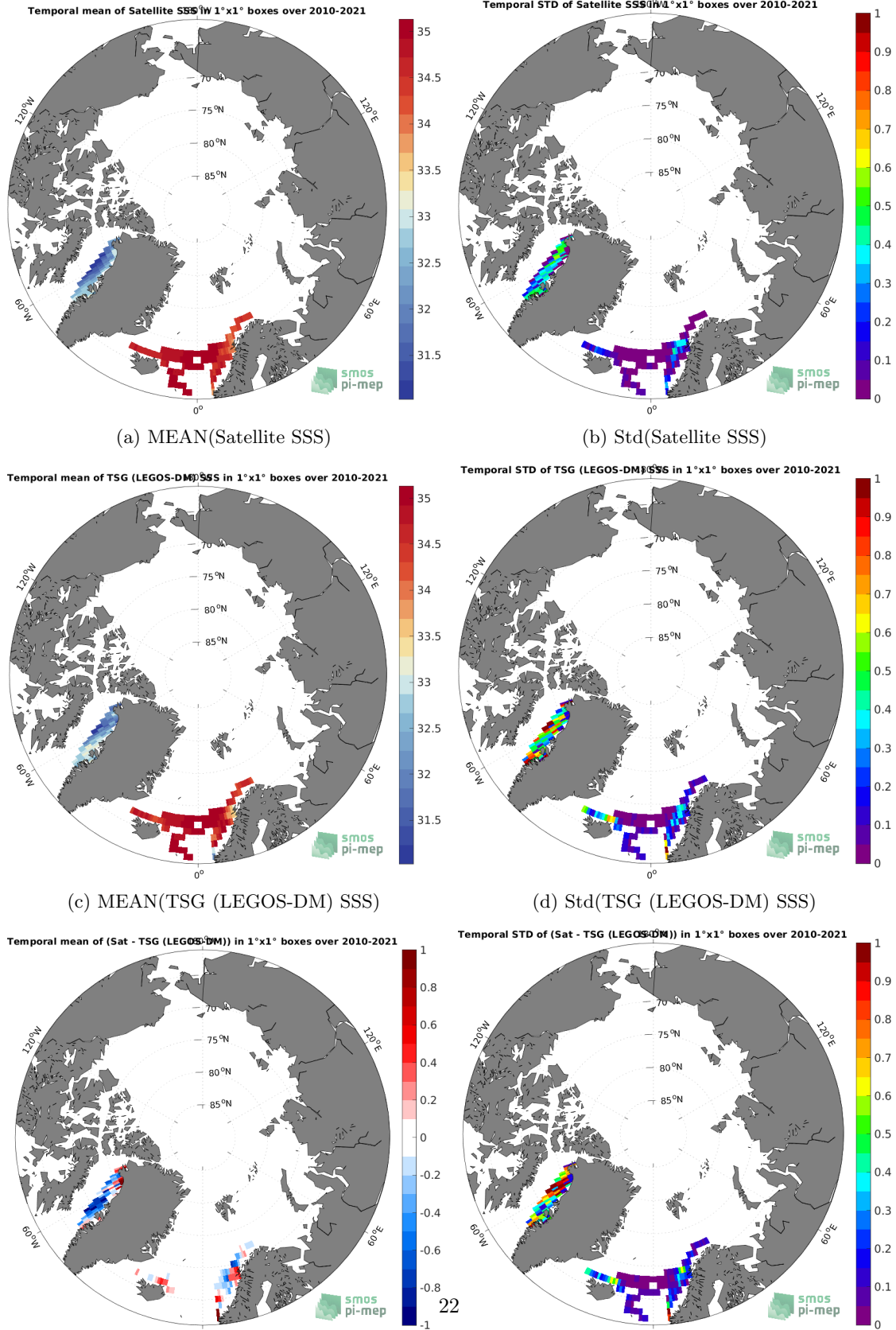
(e) MEAN( \Delta SSS) (Satellite - TSG (LEGOS-DM)) (f) Std( \Delta SSS) (Satellite - TSG (LEGOS-DM)) Figure 6: Temporal mean (left) and Std (right) of SSS from SMOS SSS L4 v1 - Monthly (CMEMS-CNR) (top), TSG (LEGOS-DM) (middle), and of \Delta SSS (Satellite - TSG (LEGOS-DM)). Only match-up pairs are used to generate these maps.
