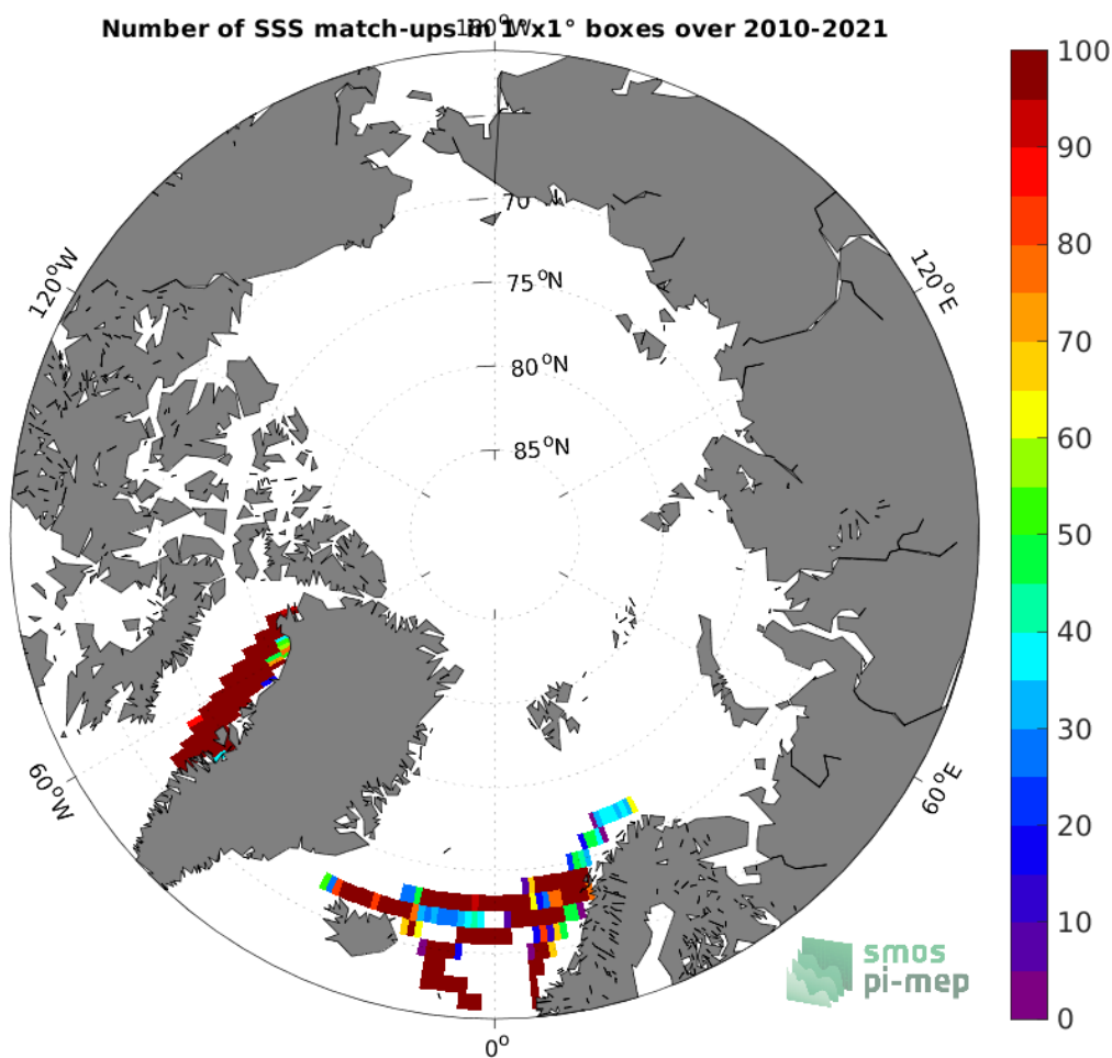
Figure 4: Number of SSS match-ups between TSG (LEGOS-DM) SSS and the SMOS SSS L4 v1 - Monthly (CMEMS-CNR) SSS product for the Arctic Ocean Pi-MEP region over 1^\circ \times 1^\circ boxes and for the full satellite product period.
