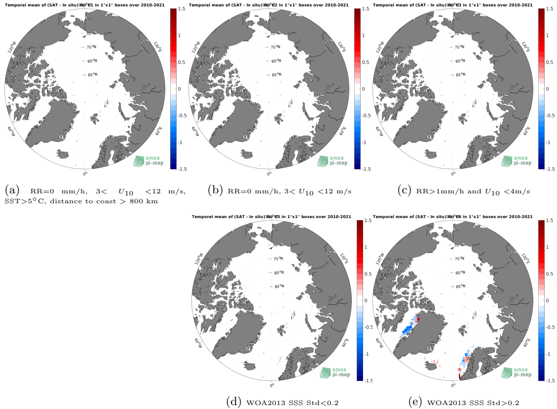
Figure 12: Temporal mean gridded over spatial boxes of size 1^{\circ}\times 1^{\circ} of \Delta\text{SSS} (SMOS SSS L4 v1 - Monthly (CMEMS-CNR) - TSG (LEGOS-DM)) for 5 different subdatasets corresponding to:RR=0 mm/h, 3 < U_{10} < 12 m/s, SST >5^{\circ}\text{C} , distance to coast > 800 km (a), RR=0 mm/h, 3 < U_{10} < 12 m/s (b), RR >1 mm/h and U_{10} < 4 m/s (c), WOA2013 SSS Std <0.2 (d), WOA2013 SSS Std >0.2 (e).
