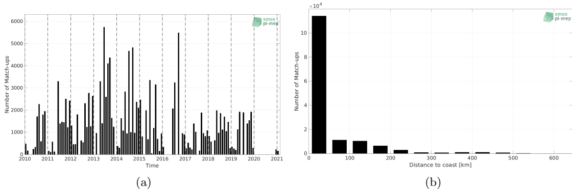
Figure 1: Number of match-ups between TSG (LEGOS-DM) and SMOS SSS L4 v1 - Monthly (CMEMS-CNR) SSS as a function of time (a) and as function of the distance to coast (b) over the Arctic Ocean Pi-MEP region and for the full satellite product period.
