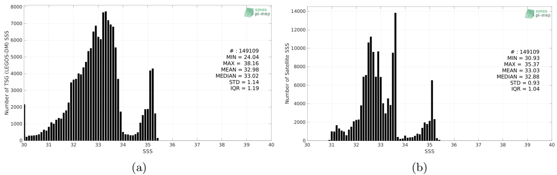
Figure 2: Histograms of SSS from TSG (LEGOS-DM) (a) and SMOS SSS L4 v1 - Monthly (CMEMS-CNR) (b) considering all match-up pairs per bins of 0.1 over the Arctic Ocean Pi-MEP region and for the full satellite product period.
