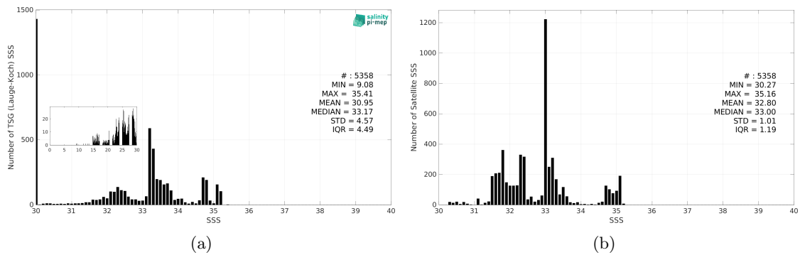
Figure 3: Histograms of SSS from TSG (Lauge-Koch) (a) and SMOS SSS L4 v1 - Monthly (CMEMS-CNR) (b) considering all match-up pairs per bins of 0.1 over the Arctic Ocean Pi-MEP region and for the full satellite product period.
