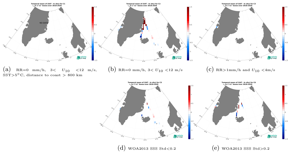
Figure 14: Temporal mean gridded over spatial boxes of size 1^\circ \times 1^\circ of \Delta SSS (SMOS SSS L4 v1 - Monthly (CMEMS-CNR) - TSG (Laugel-Koch)) for 5 different subdatasets corresponding to: RR=0 mm/h, 3 < U_{10} < 12 m/s, SST > 5^\circ C, distance to coast > 800 km (a), RR=0 mm/h, 3 < U_{10} < 12 m/s (b), RR > 1 mm/h and U_{10} < 4 m/s (c), WOA2013 SSS Std < 0.2 (d), WOA2013 SSS Std > 0.2 (e).
