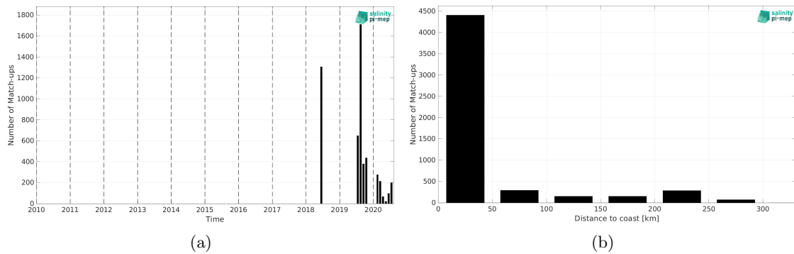
Figure 2: Number of match-ups between TSG (Lauge-Koch) and SMOS SSS L4 v1 - Monthly (CMEMS-CNR) SSS as a function of time (a) and as function of the distance to coast (b) over the Arctic Ocean Pi-MEP region and for the full satellite product period.
