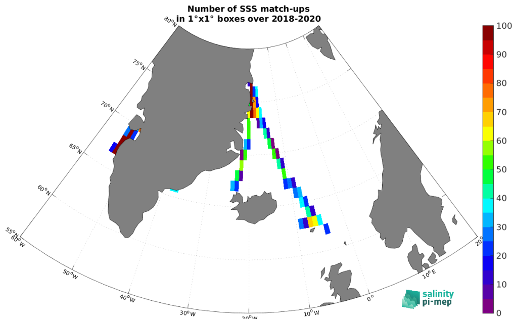
Figure 5: Number of SSS match-ups between TSG (Lauge-Koch) SSS and the SMOS SSS L4 v1 - Monthly (CMEMS-CNR) SSS product for the Arctic Ocean Pi-MEP region over 1^\circ \times 1^\circ boxes and for the full satellite product period.
