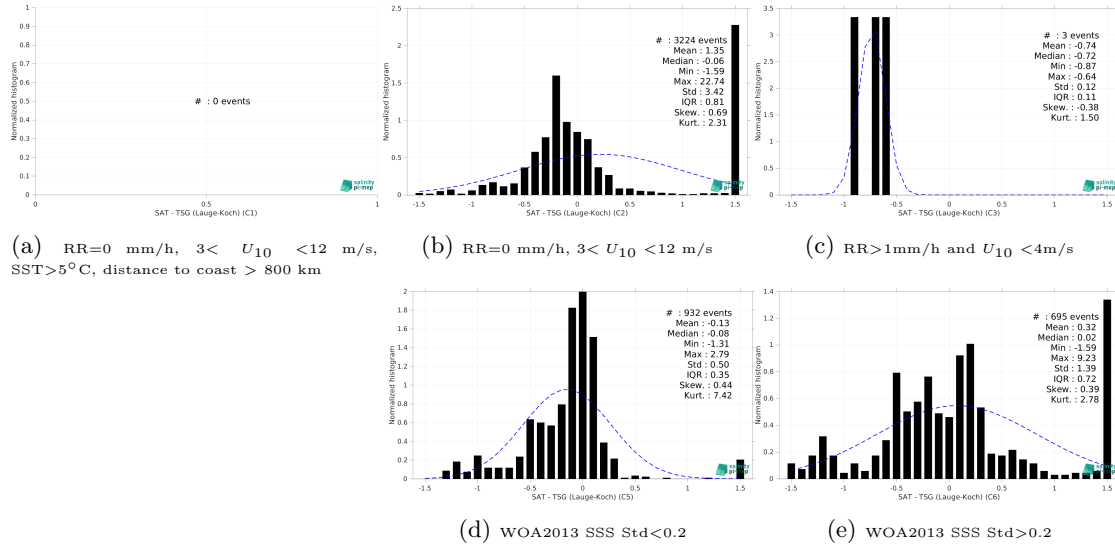
Figure 15: Normalized histogram of \Delta SSS (SMOS SSS L4 v1 - Monthly (CMEMS-CNR) - TSG (Laue-Koch)) for 5 different subdatasets corresponding to: RR=0 mm/h, 3 < U_{10} < 12 m/s, SST > 5°C, distance to coast > 800 km (a), RR=0 mm/h, 3 < U_{10} < 12 m/s (b), RR > 1mm/h and U_{10} < 4 m/s (c), WOA2013 SSS Std < 0.2 (d), WOA2013 SSS Std > 0.2 (e).
