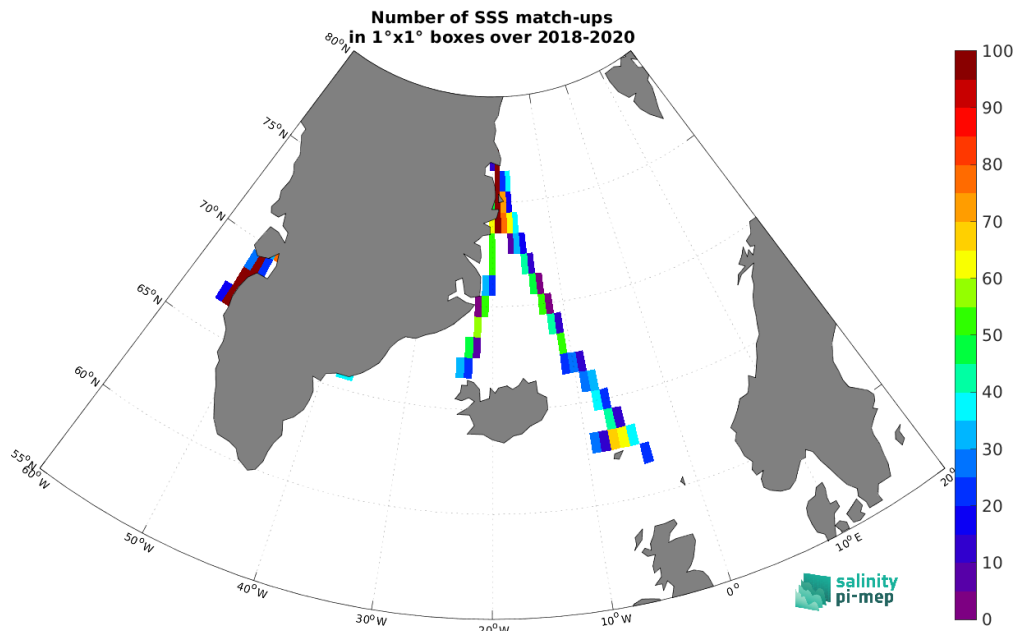
Figure 5: Number of SSS match-ups between TSG (Lauge-Koch) SSS and the SMOS SSS L4 v1 - Monthly (CMEMS-CNR) SSS product for the Arctic Ocean Pi-MEP region over 1°x1° boxes and for the full satellite product period.
