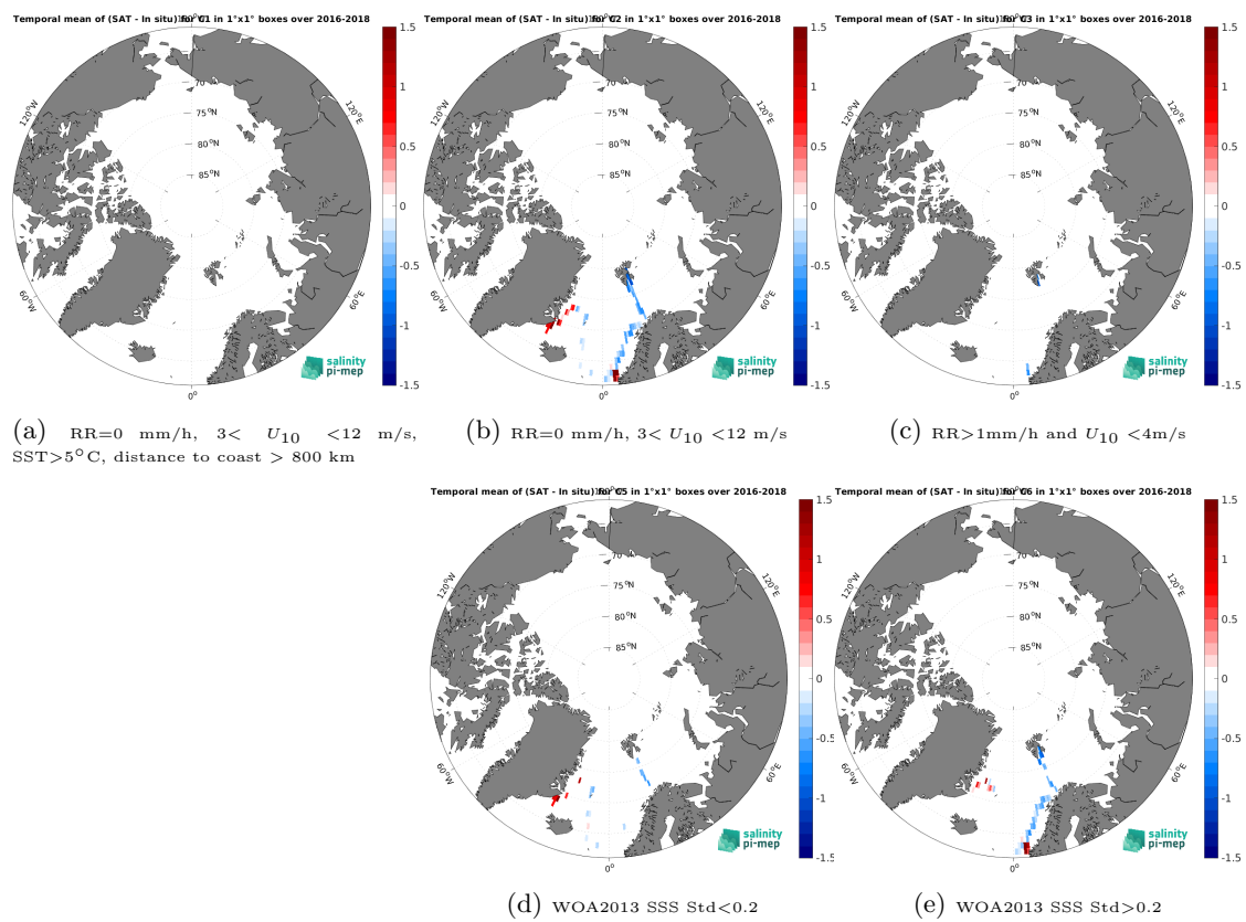
Figure 14: Temporal mean gridded over spatial boxes of size 1^\circ \times 1^\circ of \Delta\text{SSS} (SMOS SSS L4 v1 - Monthly (CMEMS-CNR) - TSG (GOSUD-Research-vessel)) for 5 different subdatasets corresponding to: RR=0 mm/h, 3 < U_{10} < 12 m/s, SST > 5°C, distance to coast > 800 km (a), RR=0 mm/h, 3 < U_{10} < 12 m/s (b), RR > 1mm/h and U_{10} < 4 m/s (c), WOA2013 SSS Std < 0.2 (d), WOA2013 SSS Std > 0.2 (e).
