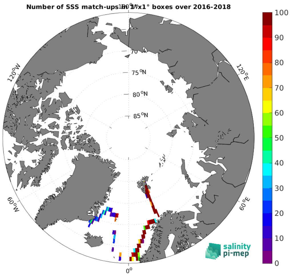
Figure 5: Number of SSS match-ups between TSG (GOSUD-Research-vessel) SSS and the SMOS SSS L4 v1 - Monthly (CMEMS-CNR) SSS product for the Arctic Ocean Pi-MEP region over 1^\circ \times 1^\circ boxes and for the full satellite product period.
