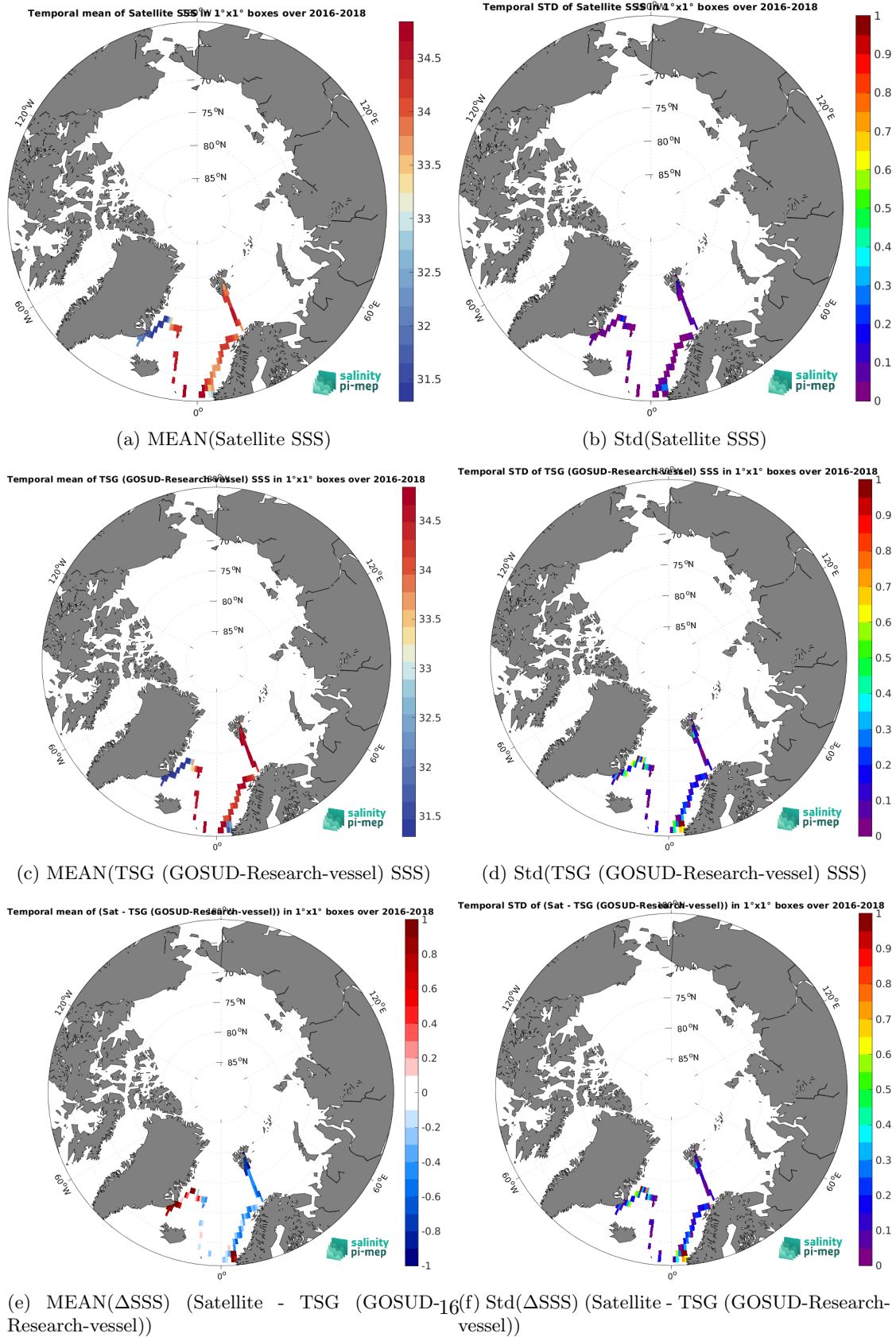
Figure 7: Temporal mean (left) and Std (right) of SSS from SMOS SSS L4 v1 - Monthly (CMEMS-CNR) (top), TSG (GOSUD-Research-vessel) (middle), and of \Delta SSS (Satellite - TSG (GOSUD-Research-vessel)). Only match-up pairs are used to generate these maps.
