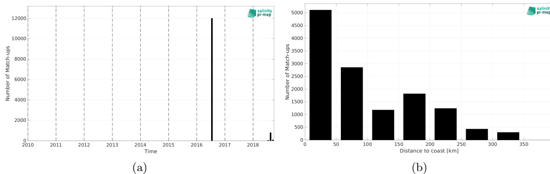
Figure 2: Number of match-ups between TSG (GOSUD-Research-vessel) and SMOS SSS L4 v1 - Monthly (CMEMS-CNR) SSS as a function of time (a) and as function of the distance to coast (b) over the Arctic Ocean Pi-MEP region and for the full satellite product period.
