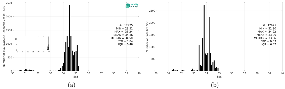
Figure 3: Histograms of SSS from TSG (GOSUD-Research-vessel) (a) and SMOS SSS L4 v1 - Monthly (CMEMS-CNR) (b) considering all match-up pairs per bins of 0.1 over the Arctic Ocean Pi-MEP region and for the full satellite product period.
