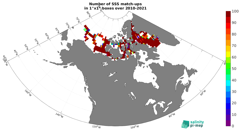
Figure 5: Number of SSS match-ups between TSG (Amundsen) SSS and the SMOS SSS L4 v1 - Monthly (CMEMS-CNR) SSS product for the Arctic Ocean Pi-MEP region over 1^\circ \times 1^\circ boxes and for the full satellite product period.
