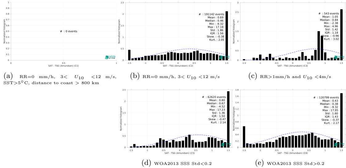
Figure 15: Normalized histogram of \Delta SSS (SMOS SSS L4 v1 - Monthly (CMEMS-CNR) - TSG (Amundsen)) for 5 different subdatasets corresponding to: RR=0 mm/h, 3 < U_{10} < 12 m/s, SST > 5°C, distance to coast > 800 km (a), RR=0 mm/h, 3 < U_{10} < 12 m/s (b), RR > 1mm/h and U_{10} < 4 m/s (c), WOA2013 SSS Std < 0.2 (d), WOA2013 SSS Std > 0.2 (e).
