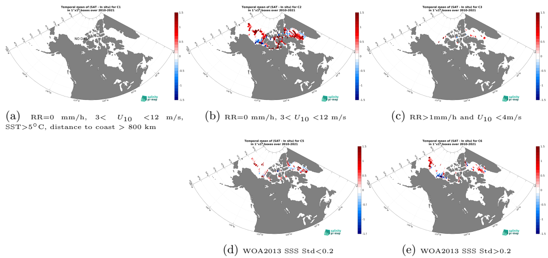
Figure 14: Temporal mean gridded over spatial boxes of size 1^\circ \times 1^\circ of \Delta SSS (SMOS SSS L4 v1 - Monthly (CMEMS-CNR) - TSG (Amundsen)) for 5 different subdatasets corresponding to: RR=0 mm/h, 3 < U_{10} < 12 m/s, SST > 5°C, distance to coast > 800 km (a), RR=0 mm/h, 3 < U_{10} < 12 m/s (b), RR > 1mm/h and U_{10} < 4 m/s (c), WOA2013 SSS Std < 0.2 (d), WOA2013 SSS Std > 0.2 (e).
