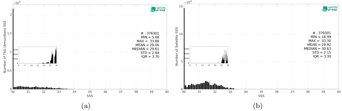
Figure 3: Histograms of SSS from TSG (Amundsen) (a) and SMOS SSS L4 v1 - Monthly (CMEMS-CNR) (b) considering all match-up pairs per bins of 0.1 over the Arctic Ocean Pi-MEP region and for the full satellite product period.
