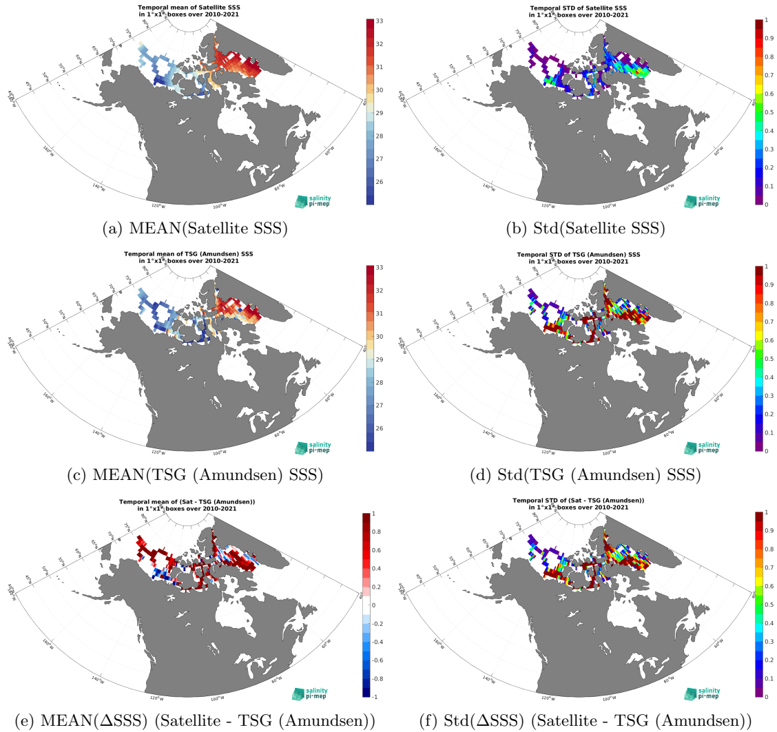
Figure 7: Temporal mean (left) and Std (right) of SSS from SMOS SSS L4 v1 - Monthly (CMEMS-CNR) (top), TSG (Amundsen) ( in situ ) (middle), and of \Delta SSS (Satellite - TSG (Amundsen)). Only match-up pairs are used to generate these maps.
