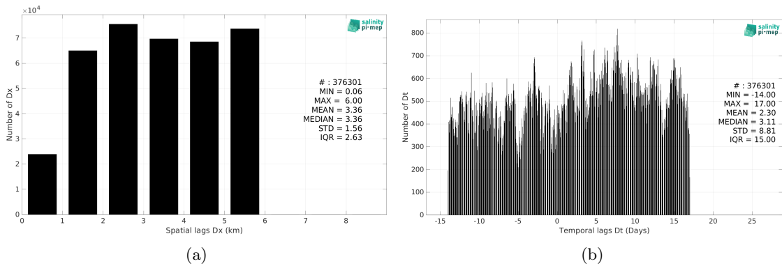
Figure 6: Histograms of the spatial (a) and temporal (b) lags between the location/time of the TSG (Amundsen) measurement and the date of the corresponding SMOS SSS L4 v1 - Monthly (CMEMS-CNR) SSS pixel.
