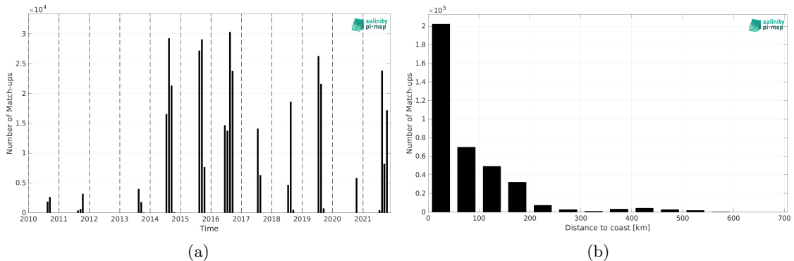
Figure 2: Number of match-ups between TSG (Amundsen) and SMOS SSS L4 v1 - Monthly (CMEMS-CNR) SSS as a function of time (a) and as function of the distance to coast (b) over the Arctic Ocean Pi-MEP region and for the full satellite product period.
