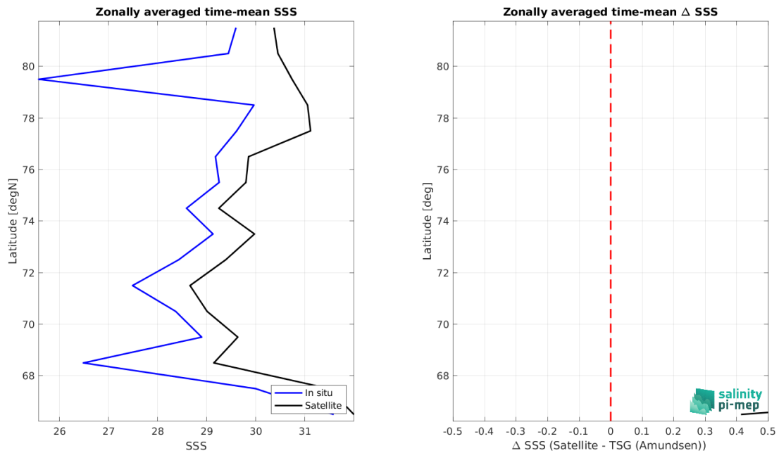
Figure 9: Left panel: Zonal mean SSS from SMOS SSS L4 v1 - Monthly (CMEMS-CNR) satellite product (black) and from TSG (Amundsen) (blue). Right panel: Zonal mean of \Delta SSS (Satellite - TSG (Amundsen)) for all the collected Pi-MEP match-up pairs estimated over the full satellite product period.
