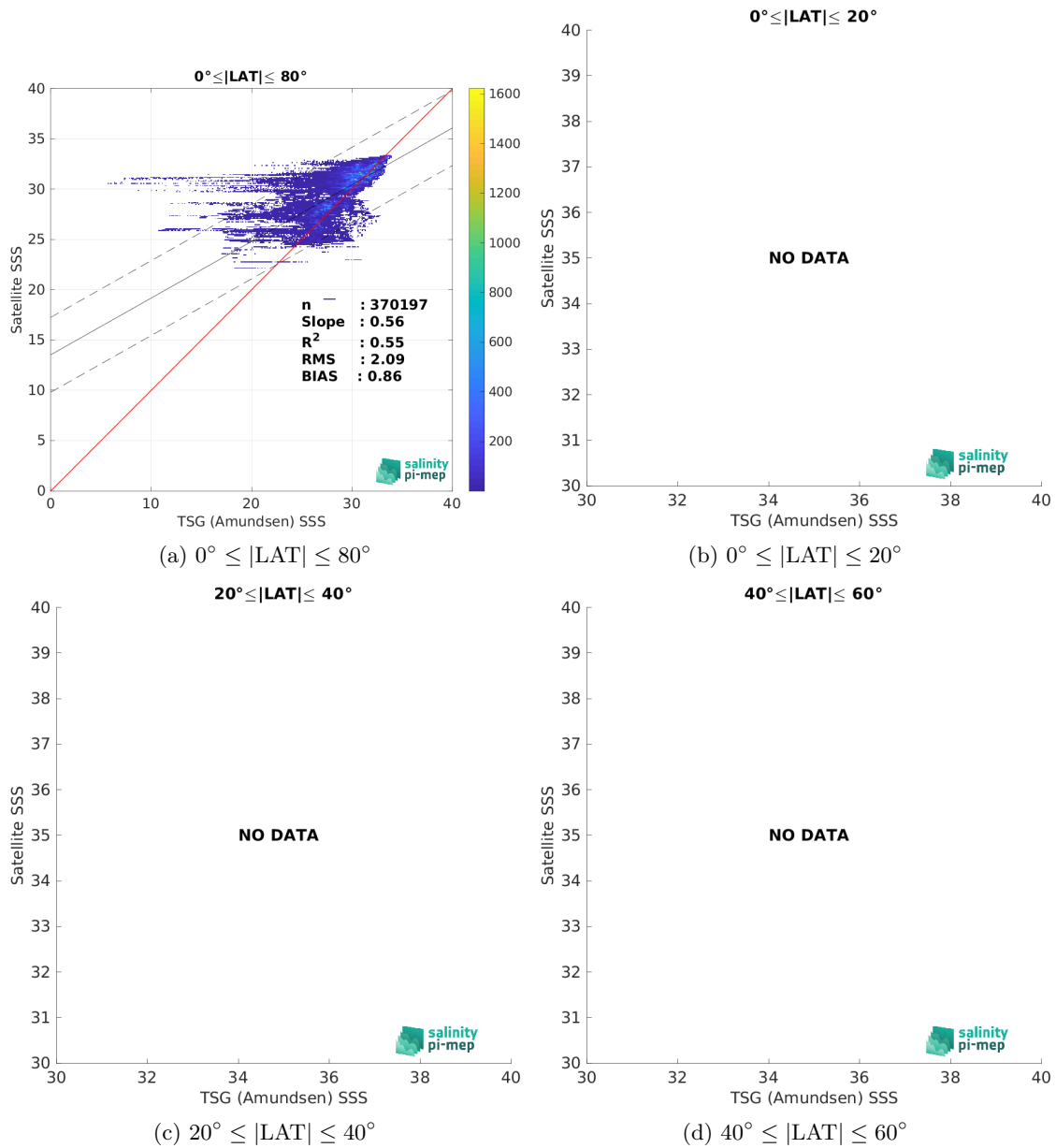
Figure 10: Contour maps of the concentration of SMOS SSS L4 v1 - Monthly (CMEMS-CNR) SSS (y-axis) versus TSG (Amundsen) SSS (x-axis) at match-up pairs for different latitude bands. For each plot, the red line shows x=y . The black thin and dashed lines indicate a linear fit through the data cloud and the \pm 95\% confidence levels, respectively. The number match-up pairs n , the slope and R^2 coefficient of the linear fit, the root mean square (RMS) and the mean bias between satellite and in situ data are indicated for each latitude band in each plots.
