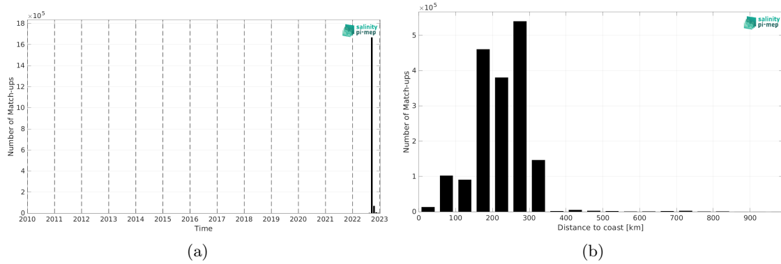
Figure 2: Number of match-ups between SASSIE and SMOS SSS L4 v1 - Monthly (CMEMS-CNR) SSS as a function of time (a) and as function of the distance to coast (b) over the Arctic Ocean Pi-MEP region and for the full satellite product period.
