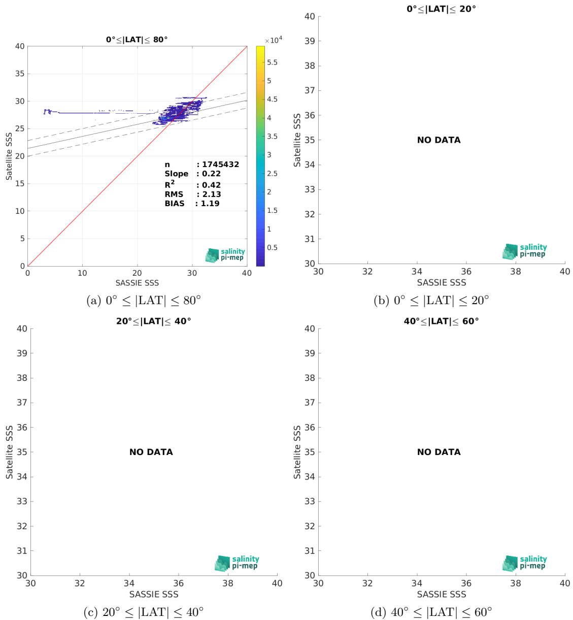
Figure 10: Contour maps of the concentration of SMOS SSS L4 v1 - Monthly (CMEMS-CNR) SSS (y-axis) versus SASSIE SSS (x-axis) at match-up pairs for different latitude bands. For each plot, the red line shows x=y . The black thin and dashed lines indicate a linear fit through the data cloud and the \pm 95\% confidence levels, respectively. The number match-up pairs n , the slope and R^2 coefficient of the linear fit, the root mean square (RMS) and the mean bias between satellite and in situ data are indicated for each latitude band in each plots.
