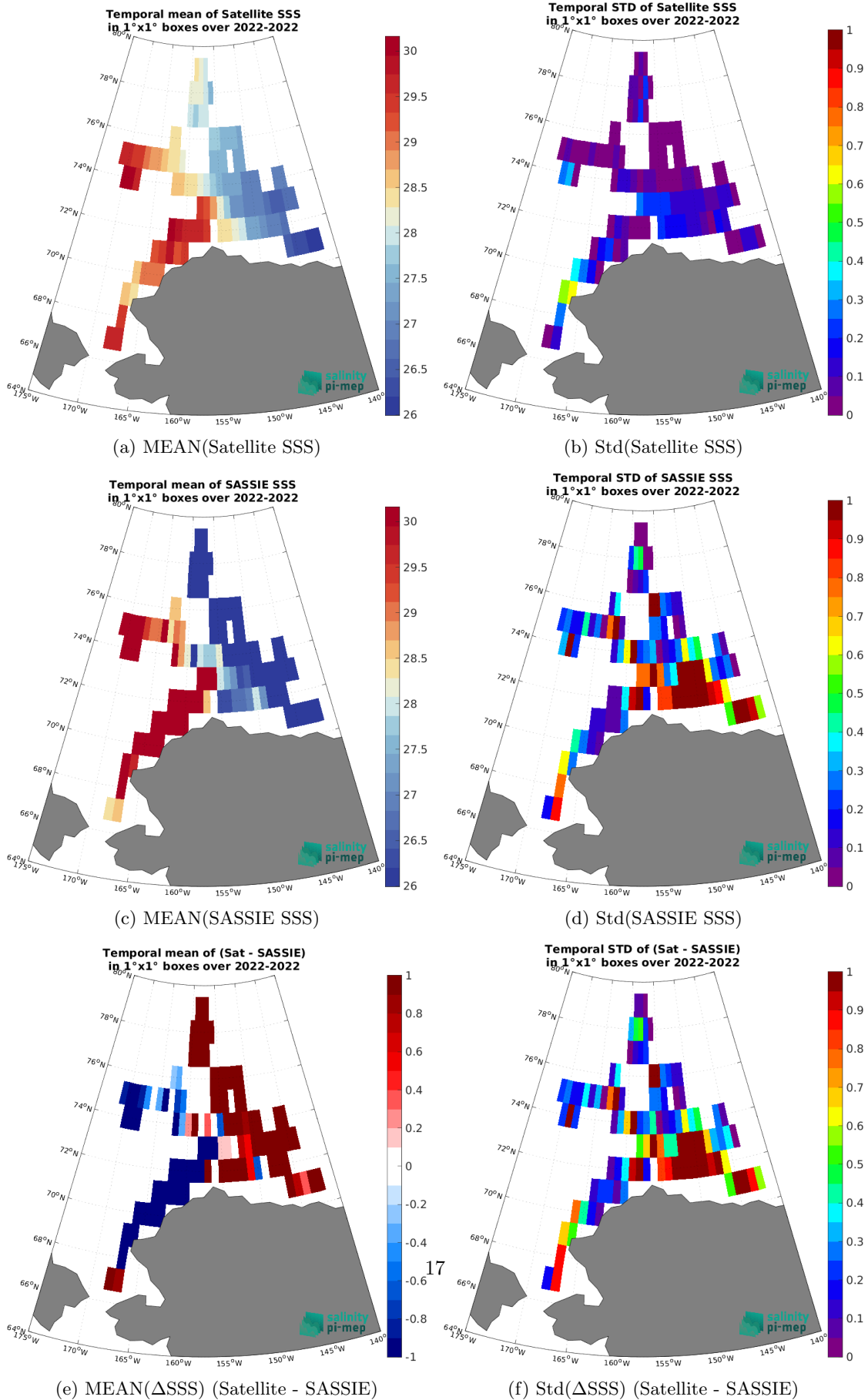
Figure 7: Temporal mean (left) and Std (right) of SSS from SMOS SSS L4 v1 - Monthly (CMEMS-CNR) (top), SASSIE (middle), and of \Delta SSS (Satellite - SASSIE). Only match-up pairs are used to generate these maps.
