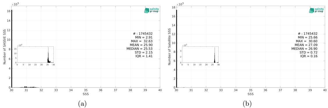
Figure 3: Histograms of SSS from SASSIE (a) and SMOS SSS L4 v1 - Monthly (CMEMS-CNR) (b) considering all match-up pairs per bins of 0.1 over the Arctic Ocean Pi-MEP region and for the full satellite product period.
