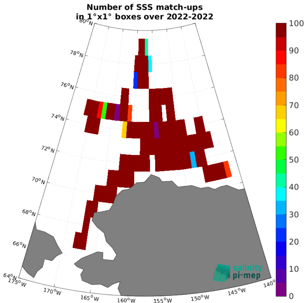
Figure 5: Number of SSS match-ups between SASSIE SSS and the SMOS SSS L4 v1 - Monthly (CMEMS-CNR) SSS product for the Arctic Ocean Pi-MEP region over 1^\circ \times 1^\circ boxes and for the full satellite product period.
