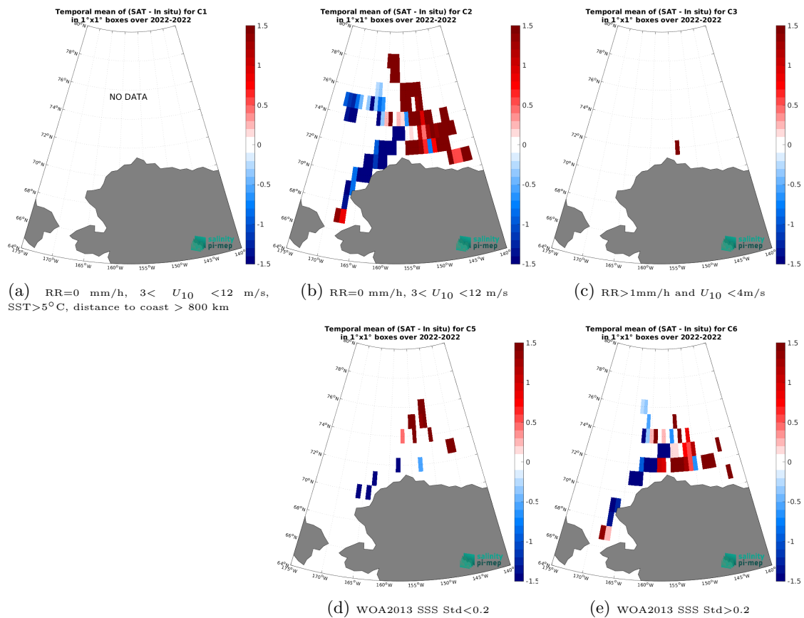
Figure 14: Temporal mean gridded over spatial boxes of size 1^\circ \times 1^\circ of \Delta SSS (SMOS SSS L4 v1 - Monthly (CMEMS-CNR) - SASSIE) for 5 different subdatasets corresponding to:RR=0 mm/h, 3 < U_{10} < 12 m/s, SST >5^\circ\text{C} , distance to coast > 800 km (a), RR=0 mm/h, 3 < U_{10} < 12 m/s (b), RR >1 mm/h and U_{10} < 4 m/s (c), WOA2013 SSS Std <0.2 (d), WOA2013 SSS Std >0.2 (e).
