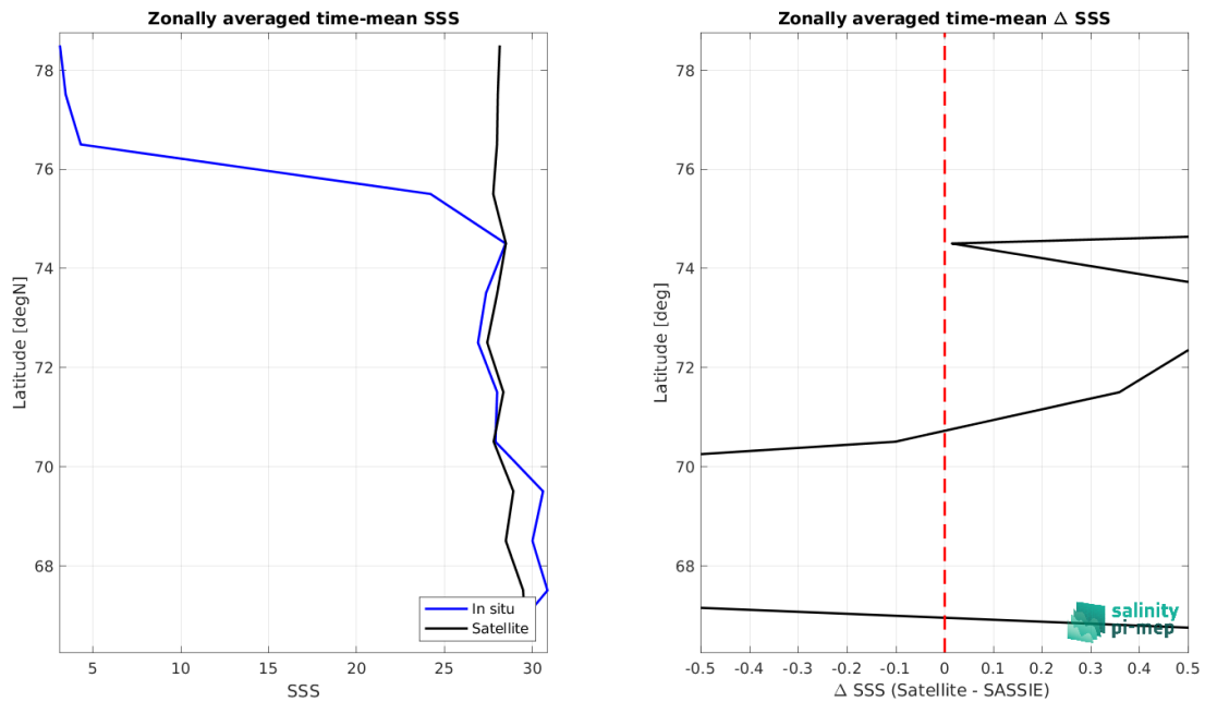
Figure 9: Left panel: Zonal mean SSS from SMOS SSS L4 v1 - Monthly (CMEMS-CNR) satellite product (black) and from SASSIE (blue). Right panel: Zonal mean of \Delta SSS (Satellite - SASSIE) for all the collected Pi-MEP match-up pairs estimated over the full satellite product period.
