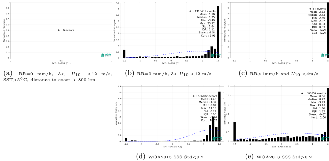
Figure 15: Normalized histogram of \Delta SSS (SMOS SSS L4 v1 - Monthly (CMEMS-CNR) - SASSIE) for 5 different subdatasets corresponding to: RR=0 mm/h, 3 < U_{10} < 12 m/s, SST > 5°C, distance to coast > 800 km (a), RR=0 mm/h, 3 < U_{10} < 12 m/s (b), RR > 1mm/h and U_{10} < 4 m/s (c), WOA2013 SSS Std < 0.2 (d), WOA2013 SSS Std > 0.2 (e).
