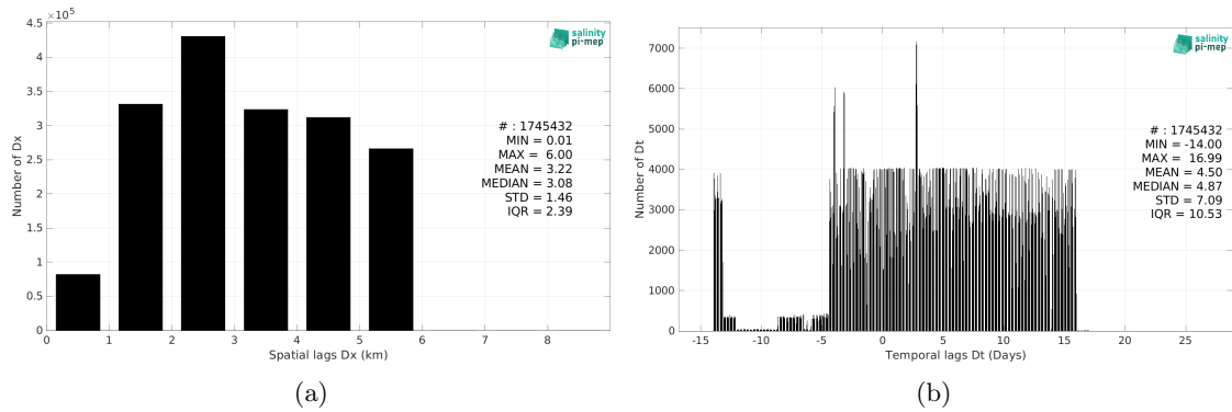
Figure 6: Histograms of the spatial (a) and temporal (b) lags between the location/time of the SASSIE measurement and the date of the corresponding SMOS SSS L4 v1 - Monthly (CMEMS-CNR) SSS pixel.
