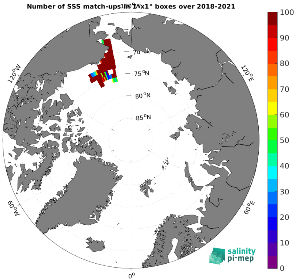
Figure 5: Number of SSS match-ups between Saildrone SSS and the SMOS SSS L4 v1 - Monthly (CMEMS-CNR) SSS product for the Arctic Ocean Pi-MEP region over 1^{\circ} \times 1^{\circ} boxes and for the full satellite product period.
