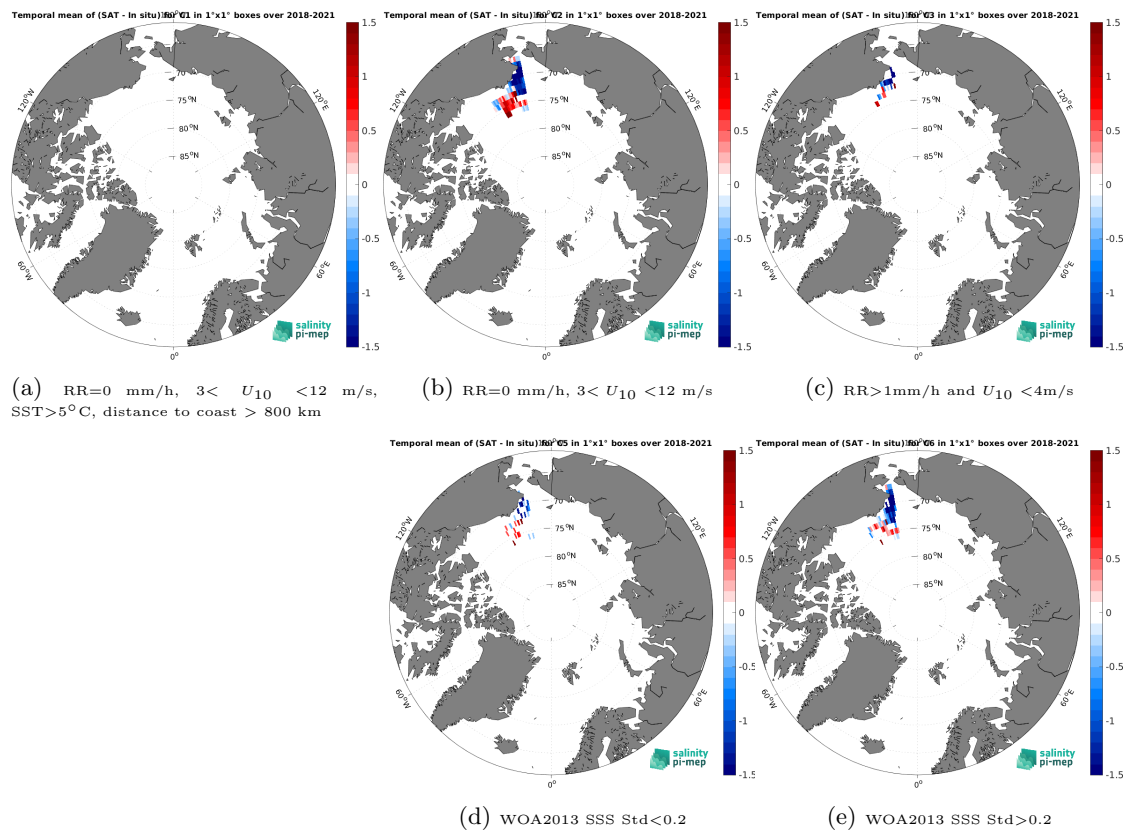
Figure 14: Temporal mean gridded over spatial boxes of size 1^\circ \times 1^\circ of \Delta\text{SSS} (SMOS SSS L4 v1 - Monthly (CMEMS-CNR) - Saildrone) for 5 different subdatasets corresponding to:RR=0 mm/h, 3 < U_{10} < 12 m/s, SST >5^\circ\text{C} , distance to coast > 800 km (a), RR=0 mm/h, 3 < U_{10} < 12 m/s (b), RR >1 mm/h and U_{10} < 4 m/s (c), WOA2013 SSS Std <0.2 (d), WOA2013 SSS Std >0.2 (e).
