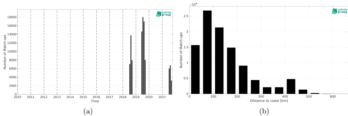
Figure 2: Number of match-ups between Saildrone and SMOS SSS L4 v1 - Monthly (CMEMS-CNR) SSS as a function of time (a) and as function of the distance to coast (b) over the Arctic Ocean Pi-MEP region and for the full satellite product period.
