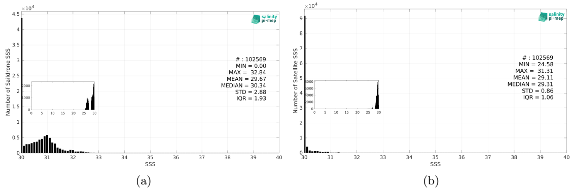
Figure 3: Histograms of SSS from Saïdrone (a) and SMOS SSS L4 v1 - Monthly (CMEMS-CNR) (b) considering all match-up pairs per bins of 0.1 over the Arctic Ocean Pi-MEP region and for the full satellite product period.
