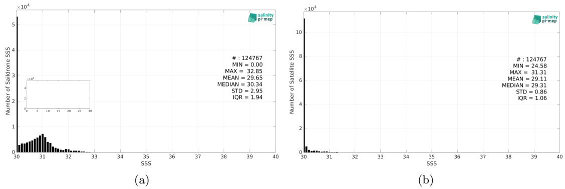
Figure 2: Histograms of SSS from Saildrone (a) and SMOS SSS L4 v1 - Monthly (CMEMS-CNR) (b) considering all match-up pairs per bins of 0.1 over the Arctic Ocean Pi-MEP region and for the full satellite product period.
