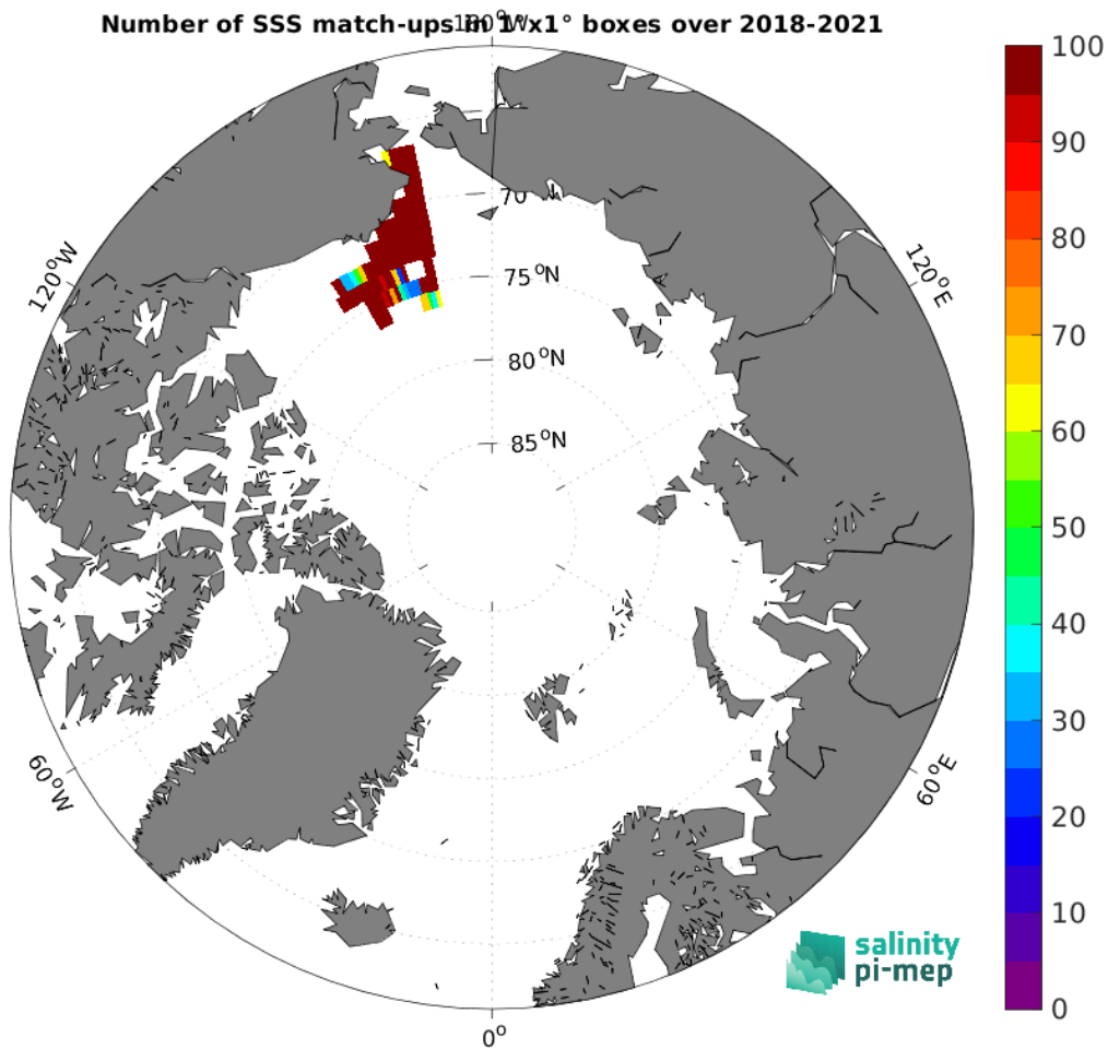
Figure 4: Number of SSS match-ups between Saildrone SSS and the SMOS SSS L4 v1 - Monthly (CMEMS-CNR) SSS product for the Arctic Ocean Pi-MEP region over 1^{\circ} \times 1^{\circ} boxes and for the full satellite product period.
