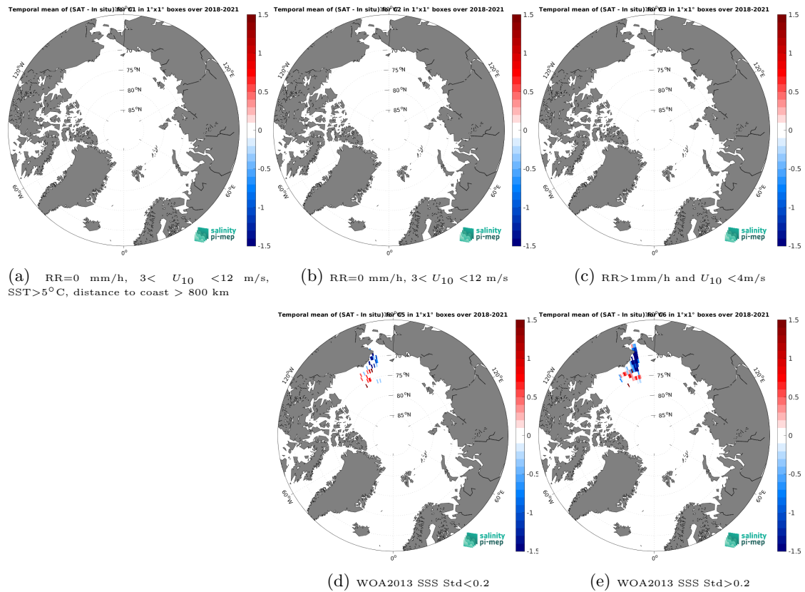
Figure 12: Temporal mean gridded over spatial boxes of size 1^{\circ}\times 1^{\circ} of \Delta\text{SSS} (SMOS SSS L4 v1 - Monthly (CMEMS-CNR) - Saifdrone) for 5 different subdatasets corresponding to:RR=0 mm/h, 3 < U_{10} < 12 m/s, SST > 5^{\circ}\text{C} , distance to coast > 800 km (a), RR=0 mm/h, 3 < U_{10} < 12 m/s (b), RR > 1 mm/h and U_{10} < 4 m/s (c), WOA2013 SSS Std < 0.2 (d), WOA2013 SSS Std > 0.2 (e).
