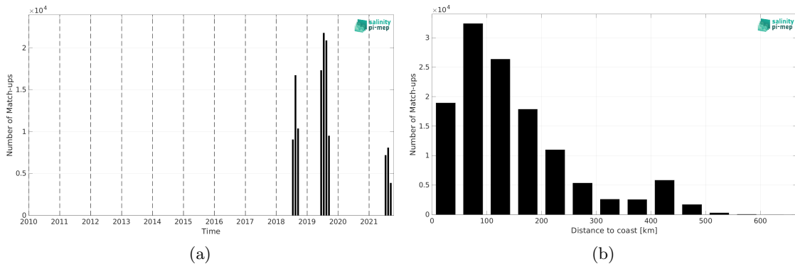
Figure 1: Number of match-ups between Saildrone and SMOS SSS L4 v1 - Monthly (CMEMS-CNR) SSS as a function of time (a) and as function of the distance to coast (b) over the Arctic Ocean Pi-MEP region and for the full satellite product period.
