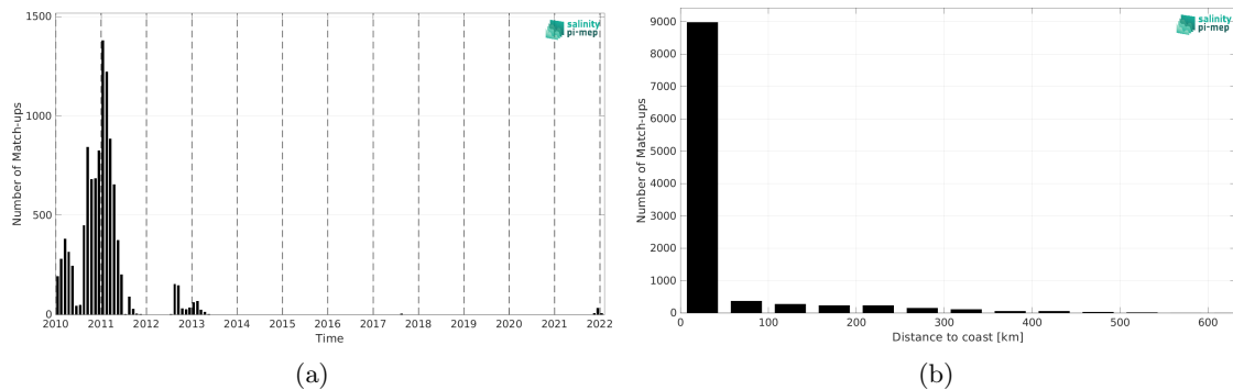
Figure 2: Number of match-ups between Marine mammals and SMOS SSS L4 v1 - Monthly (CMEMS-CNR) SSS as a function of time (a) and as function of the distance to coast (b) over the Arctic Ocean Pi-MEP region and for the full satellite product period.
