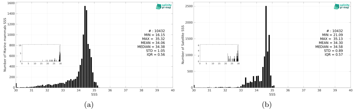
Figure 3: Histograms of SSS from Marine mammals (a) and SMOS SSS L4 v1 - Monthly (CMEMS-CNR) (b) considering all match-up pairs per bins of 0.1 over the Arctic Ocean Pi-MEP region and for the full satellite product period.
