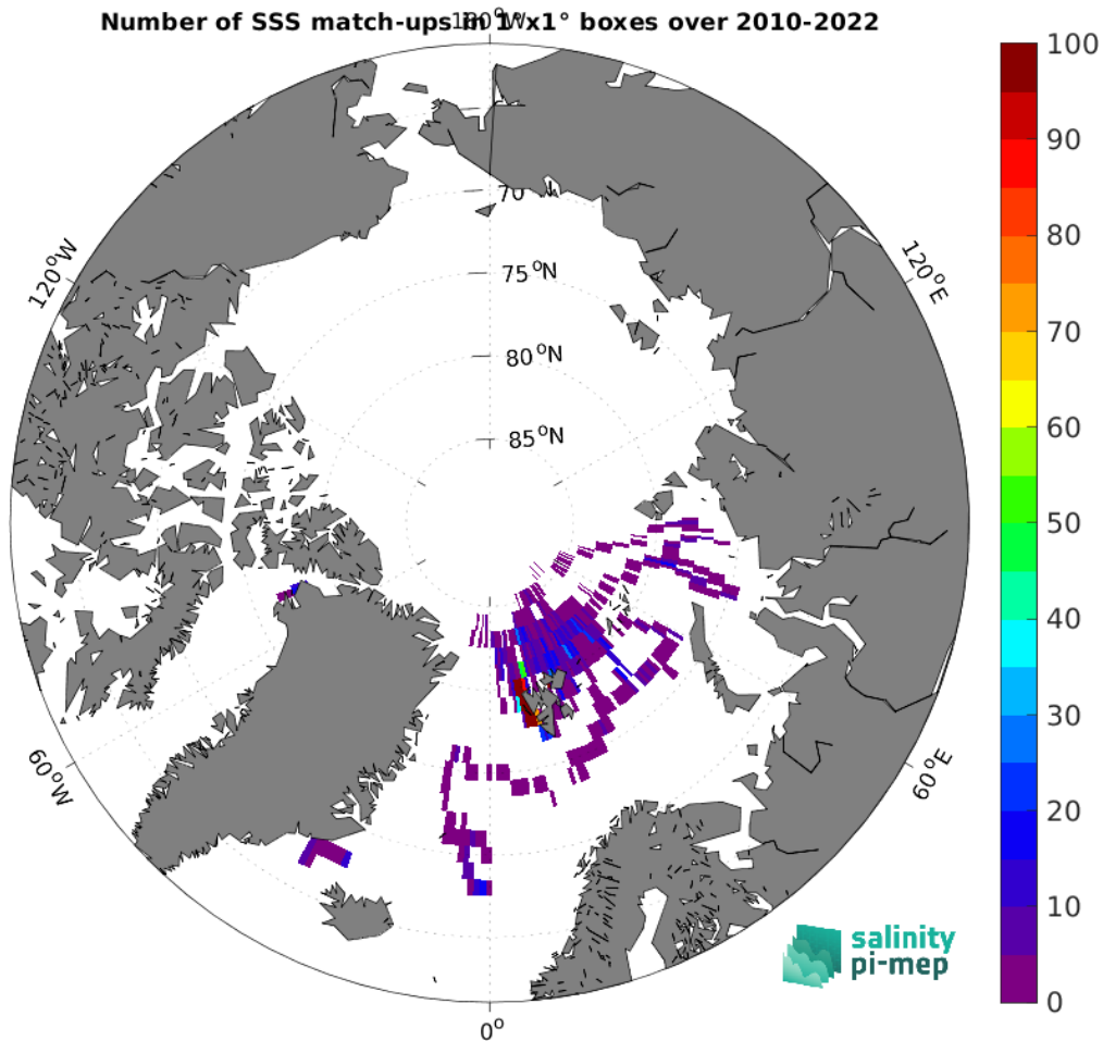
Figure 5: Number of SSS match-ups between Marine mammals SSS and the SMOS SSS L4 v1 - Monthly (CMEMS-CNR) SSS product for the Arctic Ocean Pi-MEP region over 1^\circ \times 1^\circ boxes and for the full satellite product period.
