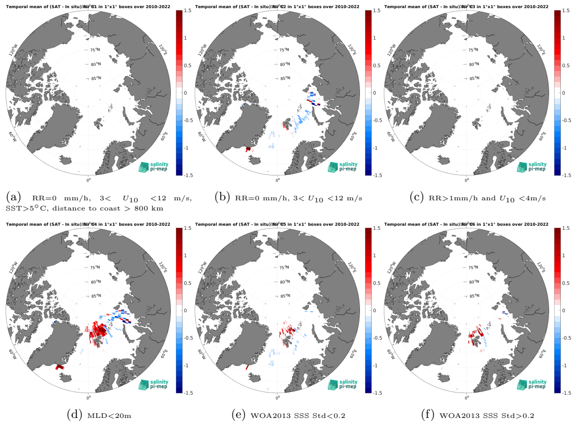
Figure 14: Temporal mean gridded over spatial boxes of size 1^\circ \times 1^\circ of \Delta SSS (SMOS SSS L4 v1 - Monthly (CMEMS-CNR) - Marine mammals) for 6 different subdatasets corresponding to:RR=0 mm/h, 3 < U_{10} < 12 m/s, SST > 5°C, distance to coast > 800 km (a), RR=0 mm/h, 3 < U_{10} < 12 m/s (b), RR > 1mm/h and U_{10} < 4 m/s (c),MLD < 20m (d),WOA2013 SSS Std < 0.2 (e),WOA2013 SSS Std > 0.2 (f).
