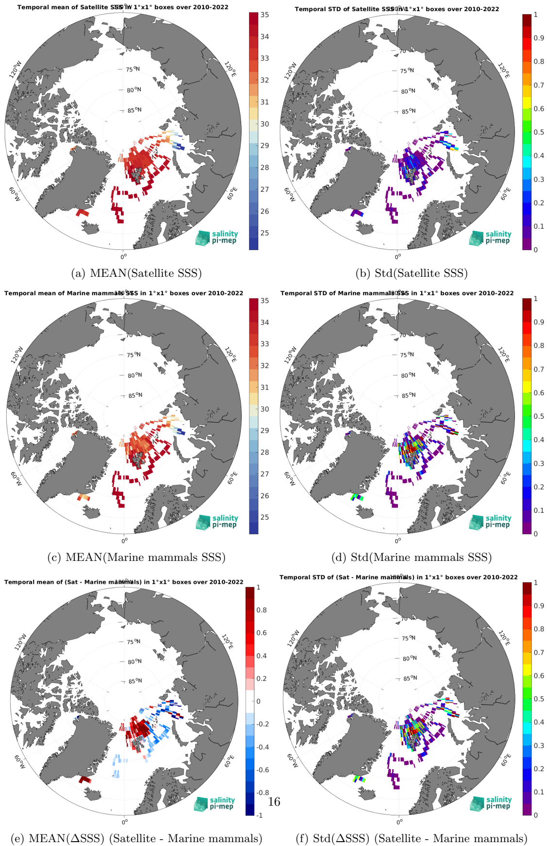
Figure 7: Temporal mean (left) and Std (right) of SSS from SMOS SSS L4 v1 - Monthly (CMEMS-CNR) (top), Marine mammals (middle), and of \Delta SSS (Satellite - Marine mammals). Only match-up pairs are used to generate these maps.
