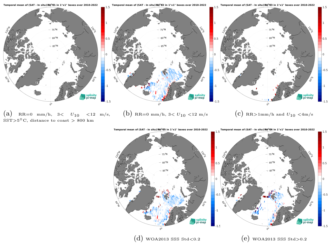
Figure 14: Temporal mean gridded over spatial boxes of size 1^\circ \times 1^\circ of \Delta SSS (SMOS SSS L4 v1 - Monthly (CMEMS-CNR) - ICES) for 5 different subdatasets corresponding to:RR=0 mm/h, 3 < U_{10} < 12 m/s, SST > 5^\circ\text{C} , distance to coast > 800 km (a), RR=0 mm/h, 3 < U_{10} < 12 m/s (b), RR > 1 mm/h and U_{10} < 4 m/s (c), WOA2013 SSS Std < 0.2 (d), WOA2013 SSS Std > 0.2 (e).
