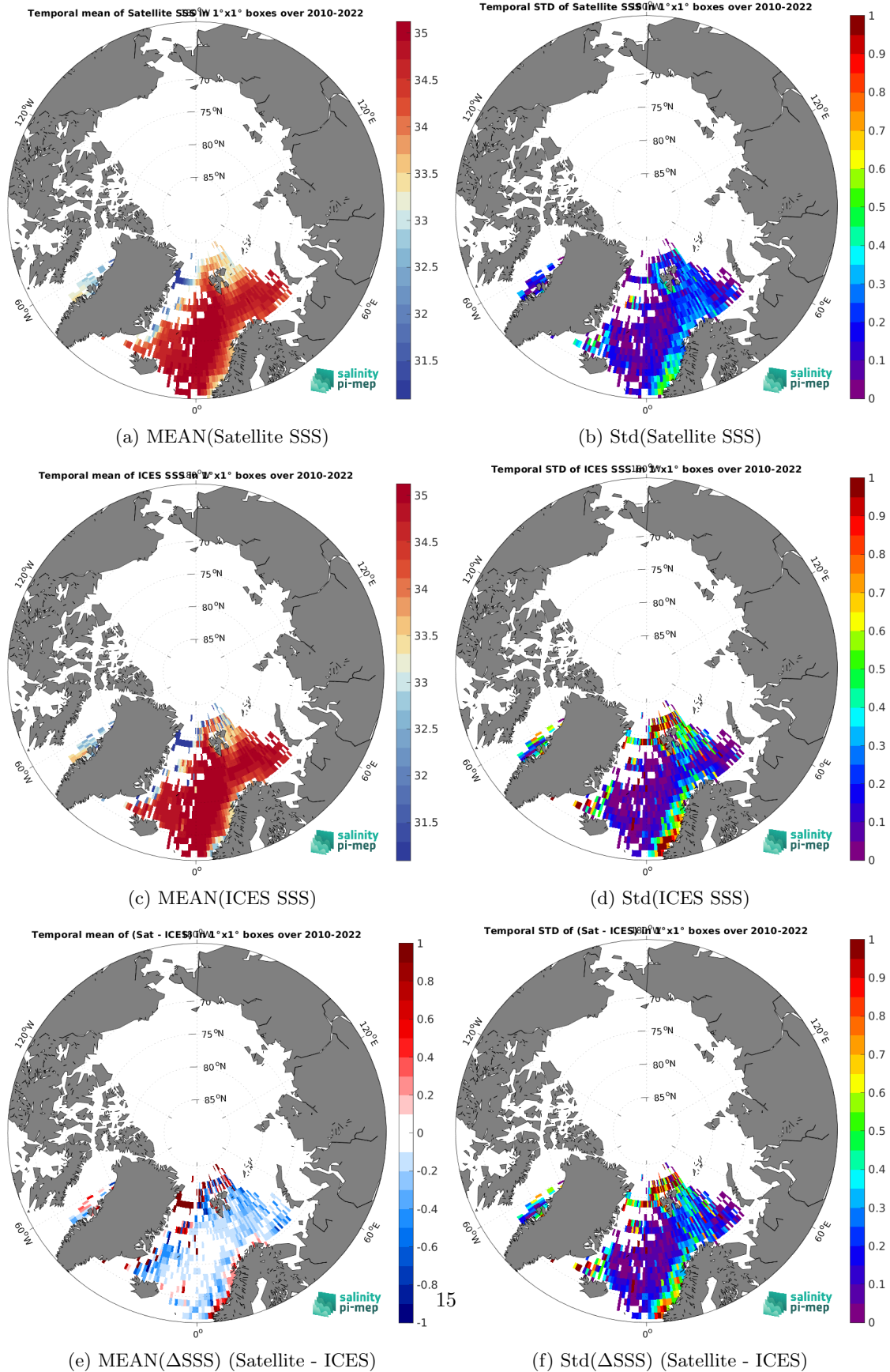
Figure 6: Temporal mean (left) and Std (right) of SSS from SMOS SSS L4 v1 - Monthly (CMEMS-CNR) (top), ICES (middle), and of \Delta SSS (Satellite - ICES). Only match-up pairs are used to generate these maps.
