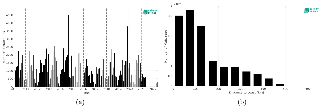
Figure 1: Number of match-ups between ICES and SMOS SSS L4 v1 - Monthly (CMEMS-CNR) SSS as a function of time (a) and as function of the distance to coast (b) over the Arctic Ocean Pi-MEP region and for the full satellite product period.
