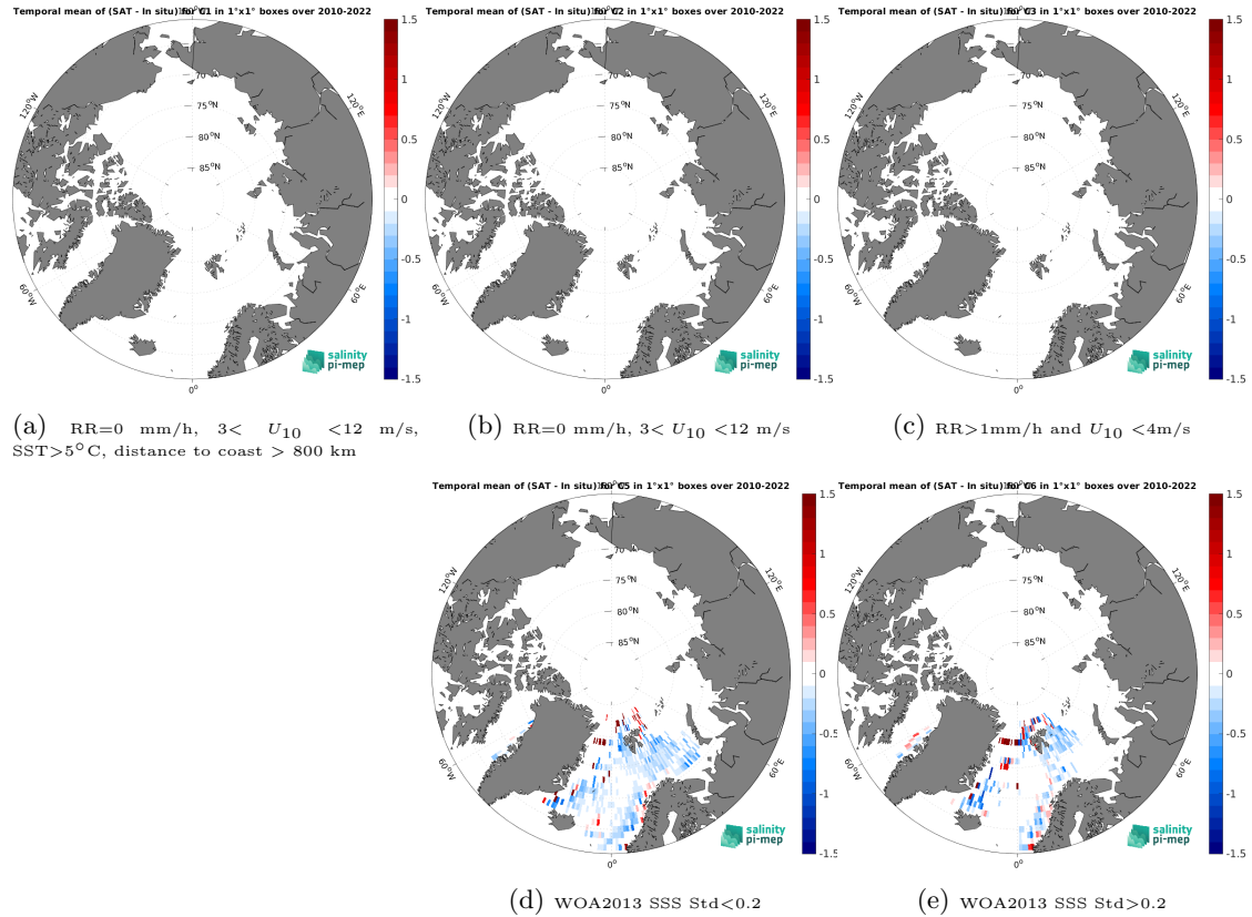
Figure 12: Temporal mean gridded over spatial boxes of size 1^{\circ}\times 1^{\circ} of \Delta\text{SSS} (SMOS SSS L4 v1 - Monthly (CMEMS-CNR) - ICES) for 5 different subdatasets corresponding to:RR=0 mm/h, 3 < U_{10} < 12 m/s, SST >5^{\circ}\text{C} , distance to coast > 800 km (a), RR=0 mm/h, 3 < U_{10} < 12 m/s (b), RR >1 mm/h and U_{10} < 4 m/s (c), WOA2013 SSS Std <0.2 (d), WOA2013 SSS Std >0.2 (e).
