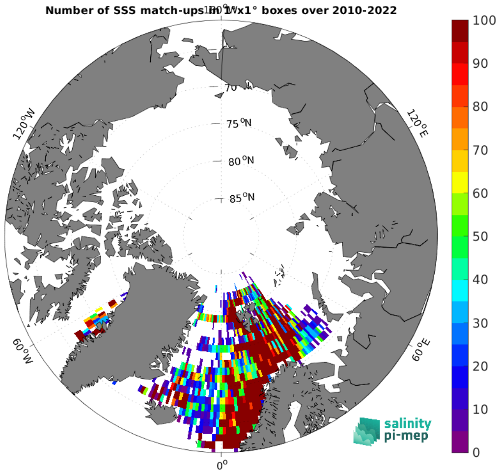
Figure 4: Number of SSS match-ups between ICES SSS and the SMOS SSS L4 v1 - Monthly (CMEMS-CNR) SSS product for the Arctic Ocean Pi-MEP region over 1^\circ \times 1^\circ boxes and for the full satellite product period.
