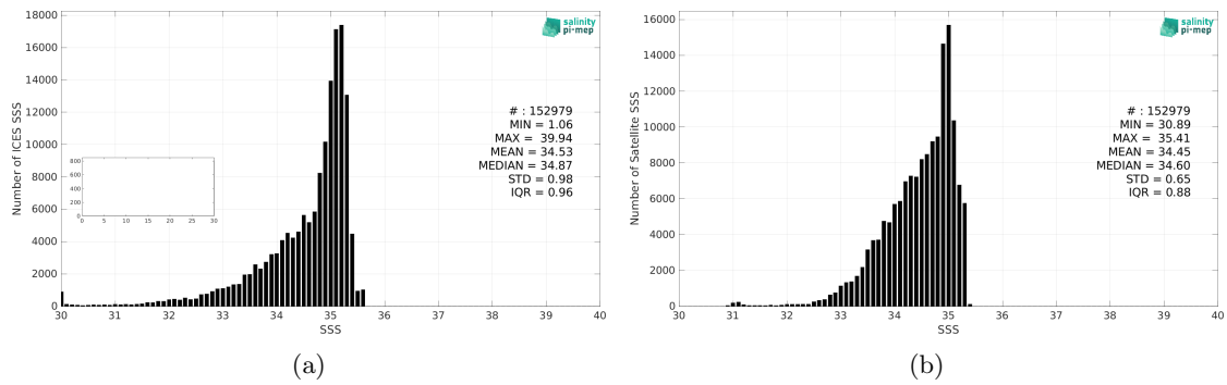
Figure 2: Histograms of SSS from ICES (a) and SMOS SSS L4 v1 - Monthly (CMEMS-CNR) (b) considering all match-up pairs per bins of 0.1 over the Arctic Ocean Pi-MEP region and for the full satellite product period.
