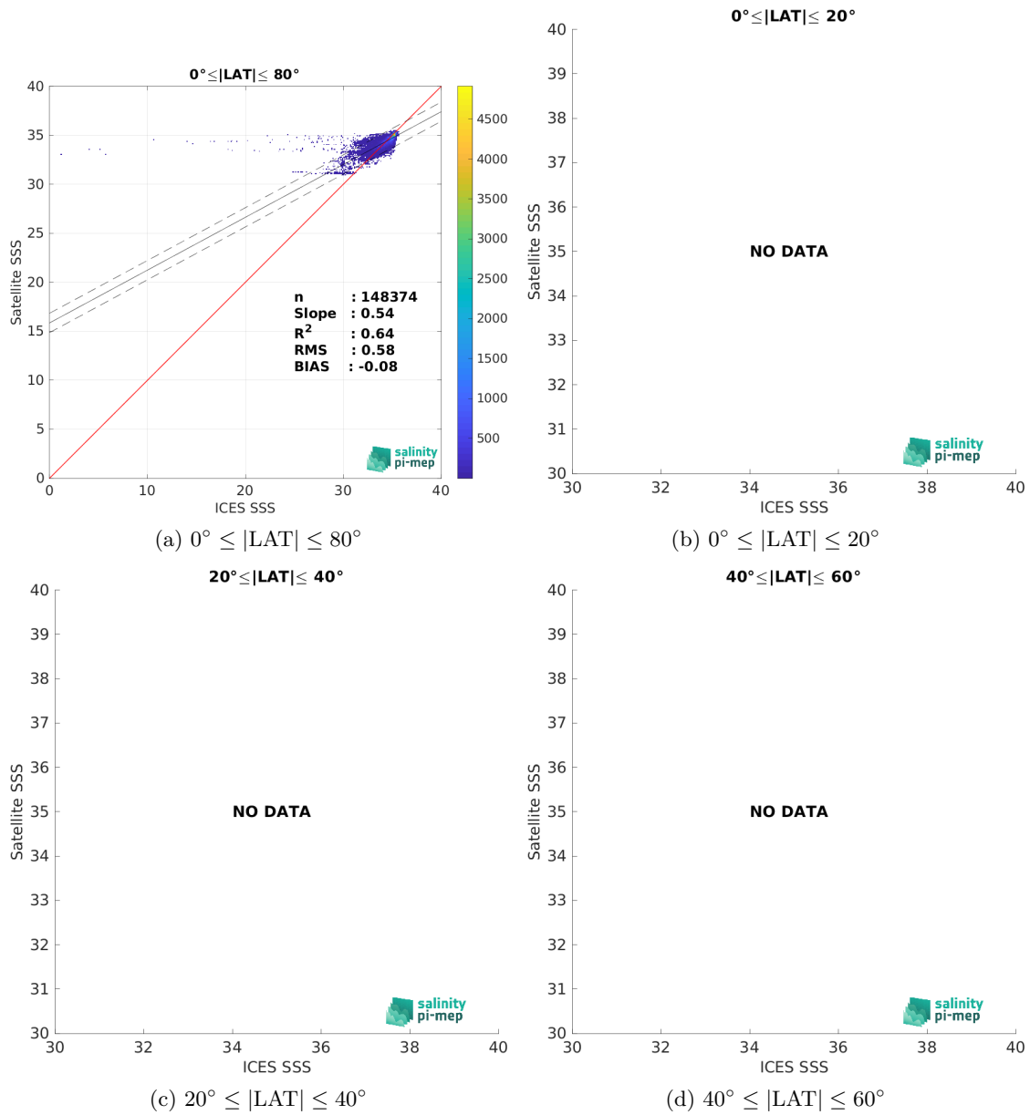
Figure 9: Contour maps of the concentration of SMOS SSS L4 v1 - Monthly (CMEMS-CNR) SSS (y-axis) versus ICES SSS (x-axis) at match-up pairs for different latitude bands. For each plot, the red line shows x=y . The black thin and dashed lines indicate a linear fit through the data cloud and the \pm 95\% confidence levels, respectively. The number match-up pairs n , the slope and R^2 coefficient of the linear fit, the root mean square (RMS) and the mean bias between satellite and in situ data are indicated for each latitude band in each plots.
