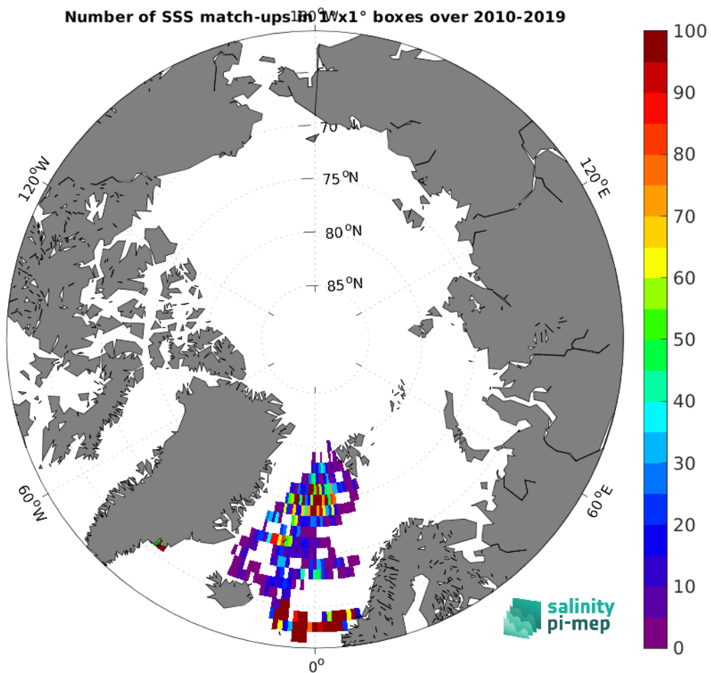
Figure 4: Number of SSS match-ups between Surface drifters SSS and the SMOS SSS L4 v1 - Monthly (CMEMS-CNR) SSS product for the Arctic Ocean Pi-MEP region over 1^\circ \times 1^\circ boxes and for the full satellite product period.
