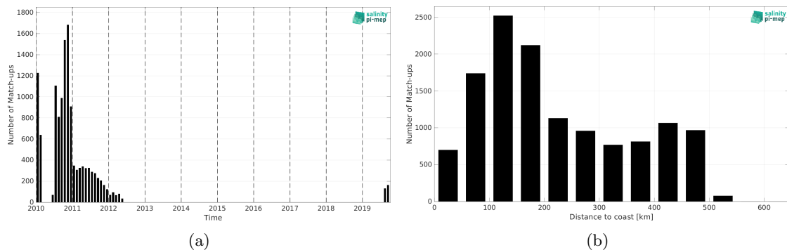
Figure 2: Number of match-ups between Surface drifters and SMOS SSS L4 v1 - Monthly (CMEMS-CNR) SSS as a function of time (a) and as function of the distance to coast (b) over the Arctic Ocean Pi-MEP region and for the full satellite product period.
