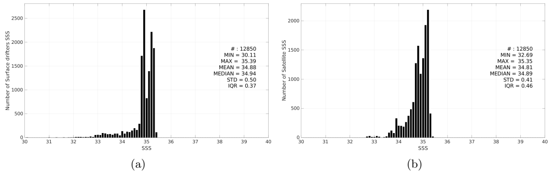
Figure 3: Histograms of SSS from Surface drifters (a) and SMOS SSS L4 v1 - Monthly (CMEMS-CNR) (b) considering all match-up pairs per bins of 0.1 over the Arctic Ocean Pi-MEP region and for the full satellite product period.
