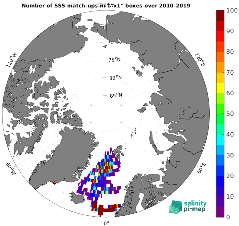
Figure 3: Number of SSS match-ups between Surface drifters SSS and the SMOS SSS L4 v1 - Monthly (CMEMS-CNR) SSS product for the Arctic Ocean Pi-MEP region over 1^{\circ} \times 1^{\circ} boxes and for the full satellite product period.
