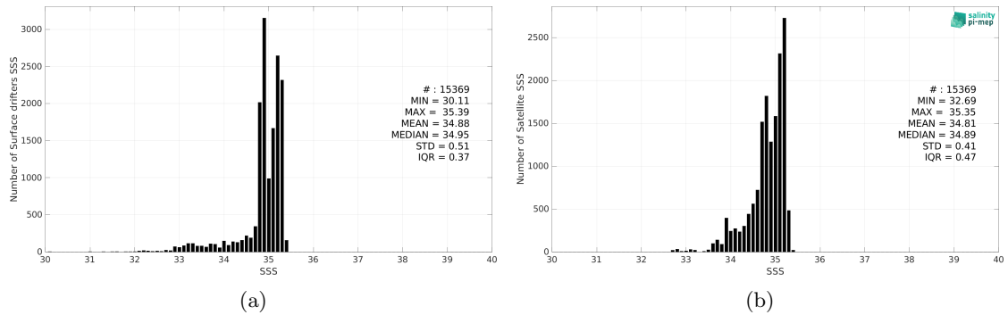
Figure 2: Histograms of SSS from Surface drifters (a) and SMOS SSS L4 v1 - Monthly (CMEMS-CNR) (b) considering all match-up pairs per bins of 0.1 over the Arctic Ocean Pi-MEP region and for the full satellite product period.
