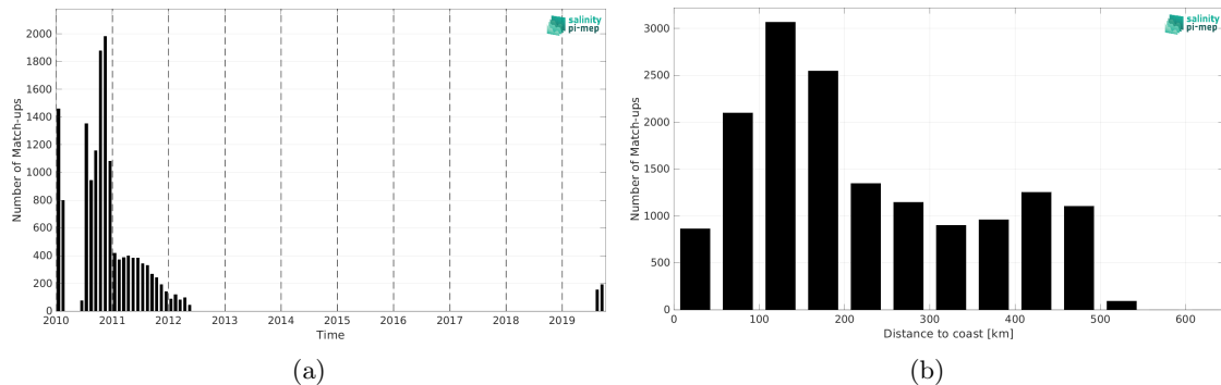
Figure 1: Number of match-ups between Surface drifters and SMOS SSS L4 v1 - Monthly (CMEMS-CNR) SSS as a function of time (a) and as function of the distance to coast (b) over the Arctic Ocean Pi-MEP region and for the full satellite product period.
