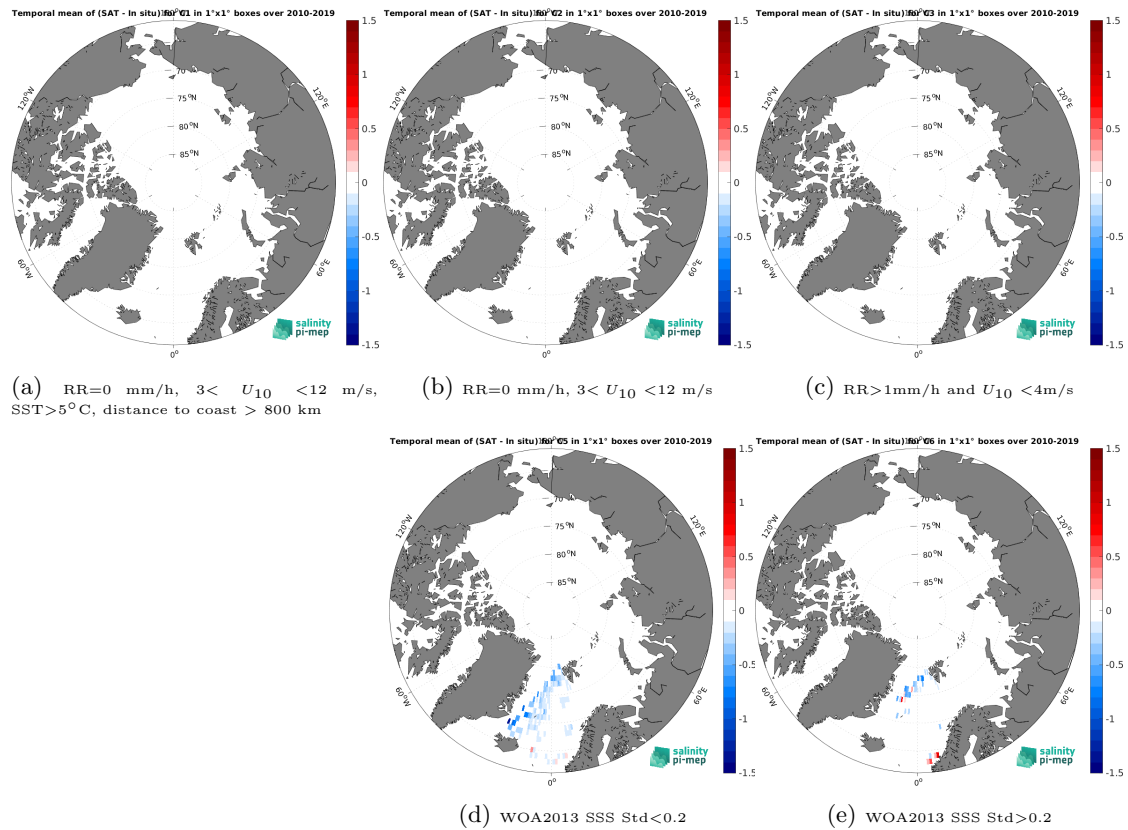
Figure 11: Temporal mean gridded over spatial boxes of size 1^{\circ}\times 1^{\circ} of \Delta\text{SSS} (SMOS SSS L4 v1 - Monthly (CMEMS-CNR) - Surface drifters) for 5 different subdatasets corresponding to:RR=0 mm/h, 3 < U_{10} < 12 m/s, SST >5^{\circ}\text{C} , distance to coast > 800 km (a), RR=0 mm/h, 3 < U_{10} < 12 m/s (b), RR >1 mm/h and U_{10} < 4 m/s (c), WOA2013 SSS Std <0.2 (d), WOA2013 SSS Std >0.2 (e).
