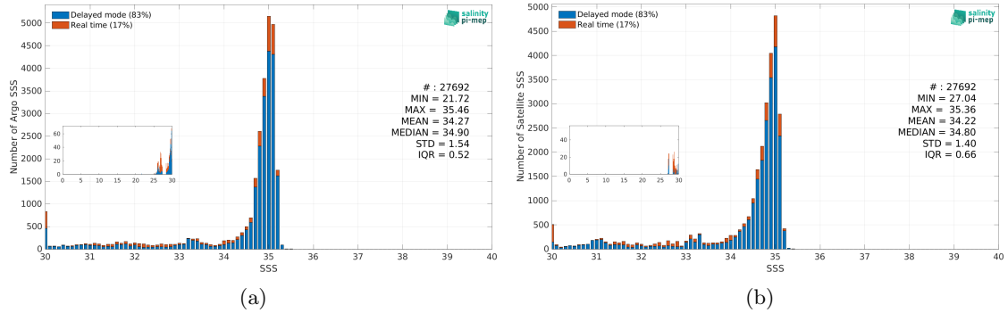
Figure 3: Histograms of SSS from Argo (a) and SMOS SSS L4 v1 - Monthly (CMEMS-CNR) (b) considering all match-up pairs per bins of 0.1 over the Arctic Ocean Pi-MEP region and for the full satellite product period.
