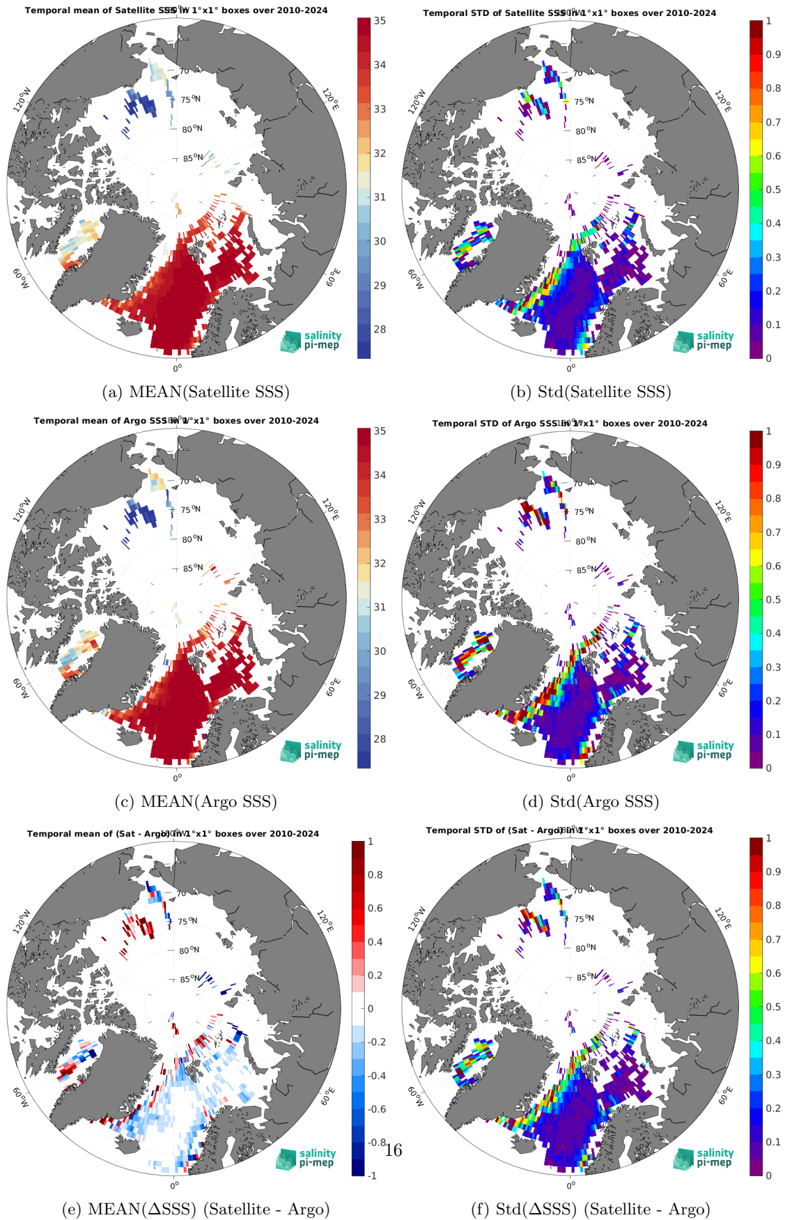
Figure 7: Temporal mean (left) and Std (right) of SSS from SMOS SSS L4 v1 - Monthly (CMEMS-CNR) (top), Argo (middle), and of \Delta SSS (Satellite - Argo). Only match-up pairs are used to generate these maps.
