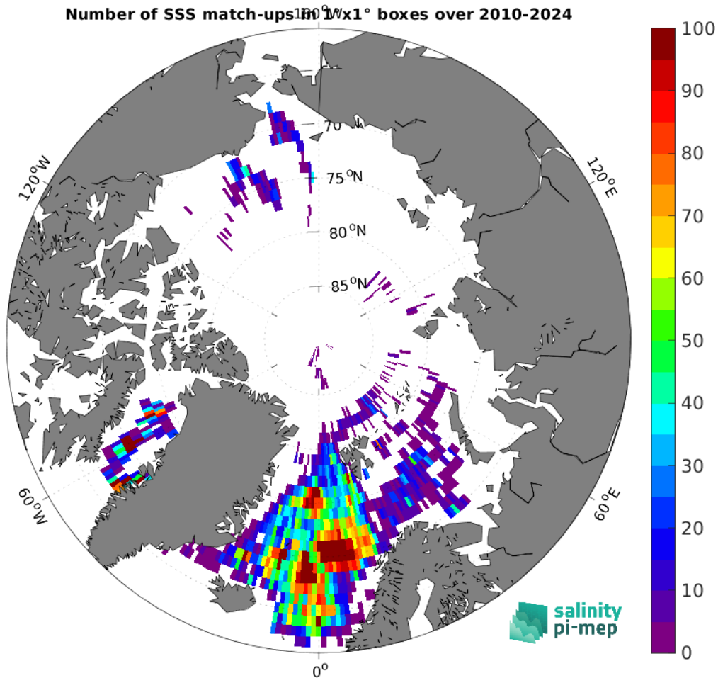
Figure 5: Number of SSS match-ups between Argo SSS and the SMOS SSS L4 v1 - Monthly (CMEMS-CNR) SSS product for the Arctic Ocean Pi-MEP region over 1^\circ \times 1^\circ boxes and for the full satellite product period.
