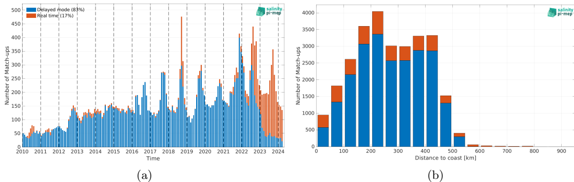
Figure 2: Number of match-ups between Argo and SMOS SSS L4 v1 - Monthly (CMEMS-CNR) SSS as a function of time (a) and as function of the distance to coast (b) over the Arctic Ocean Pi-MEP region and for the full satellite product period.
