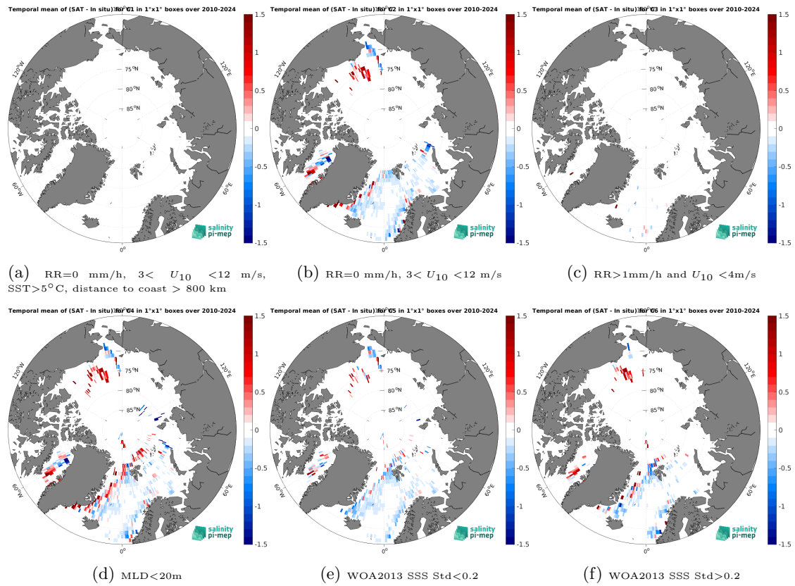
Figure 14: Temporal mean gridded over spatial boxes of size 1^\circ \times 1^\circ of \Delta SSS (SMOS SSS L4 v1 - Monthly (CMEMS-CNR) - Argo) for 6 different subdatasets corresponding to:RR=0 mm/h, 3 < U_{10} < 12 m/s, SST>5°C, distance to coast > 800 km (a), RR=0 mm/h, 3 < U_{10} < 12 m/s (b), RR>1mm/h and U_{10} < 4 m/s (c),MLD<20m (d),WOA2013 SSS Std<0.2 (e),WOA2013 SSS Std>0.2 (f).
