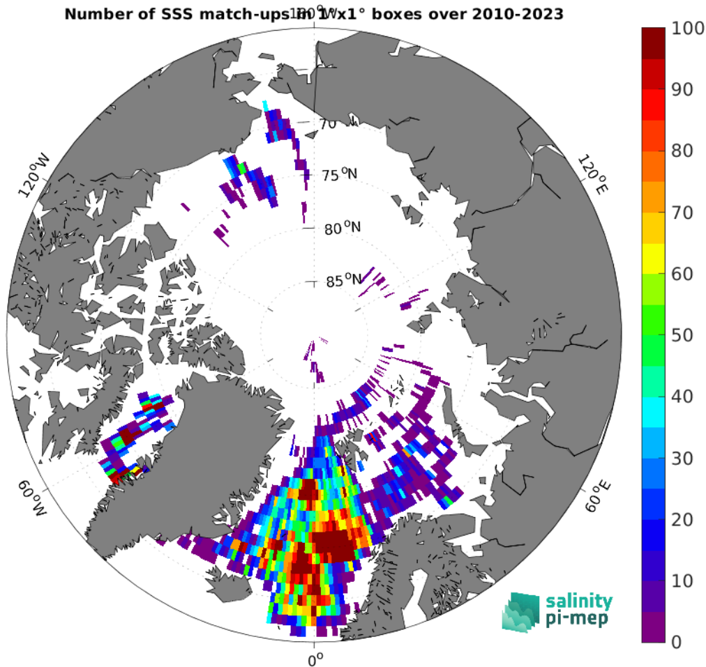
Figure 4: Number of SSS match-ups between Argo SSS and the SMOS SSS L4 v1 - Monthly (CMEMS-CNR) SSS product for the Arctic Ocean Pi-MEP region over 1^\circ \times 1^\circ boxes and for the full satellite product period.
