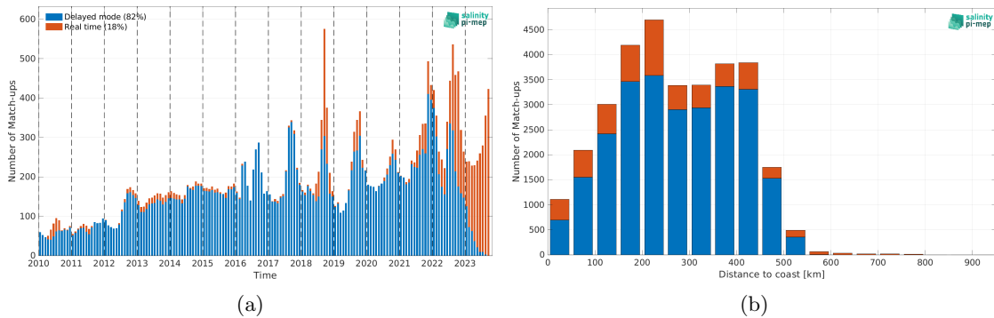
Figure 1: Number of match-ups between Argo and SMOS SSS L4 v1 - Monthly (CMEMS-CNR) SSS as a function of time (a) and as function of the distance to coast (b) over the Arctic Ocean Pi-MEP region and for the full satellite product period.
