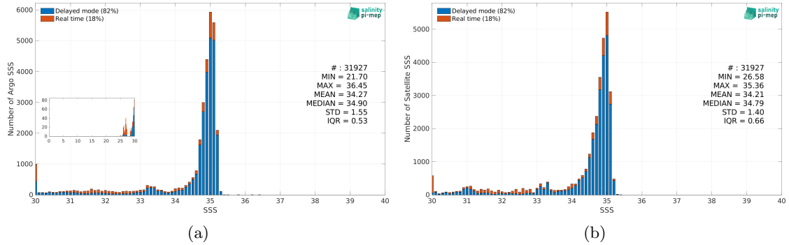
Figure 2: Histograms of SSS from Argo (a) and SMOS SSS L4 v1 - Monthly (CMEMS-CNR) (b) considering all match-up pairs per bins of 0.1 over the Arctic Ocean Pi-MEP region and for the full satellite product period.
