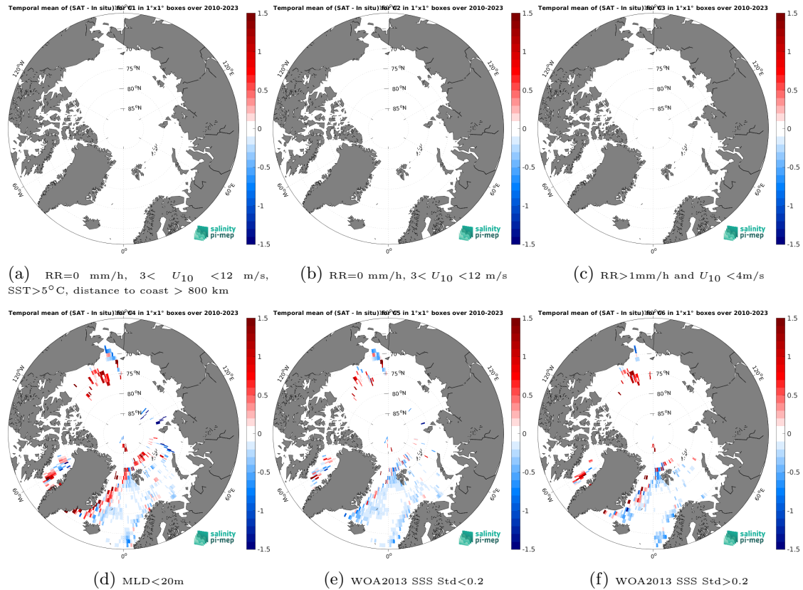
Figure 12: Temporal mean gridded over spatial boxes of size 1^{\circ}\times 1^{\circ} of \Delta\text{SSS} (SMOS SSS L4 v1 - Monthly (CMEMS-CNR) - Argo) for 6 different subdatasets corresponding to:RR=0 mm/h, 3 < U_{10} < 12 m/s, SST > 5^{\circ}\text{C} , distance to coast > 800 km (a), RR=0 mm/h, 3 < U_{10} < 12 m/s (b), RR > 1\text{mm/h} and U_{10} < 4\text{m/s} (c),MLD < 20\text{m} (d),WOA2013 SSS Std < 0.2 (e),WOA2013 SSS Std > 0.2 (f).
