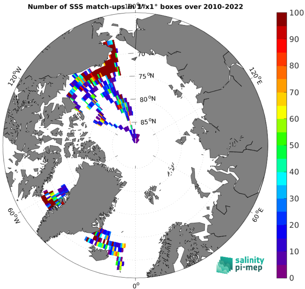
Figure 5: Number of SSS match-ups between TSG (SAMOS) SSS and the SMOS SSS L4 v1 - Daily (CMEMS-CNR) SSS product for the Arctic Ocean Pi-MEP region over 1^\circ \times 1^\circ boxes and for the full satellite product period.
