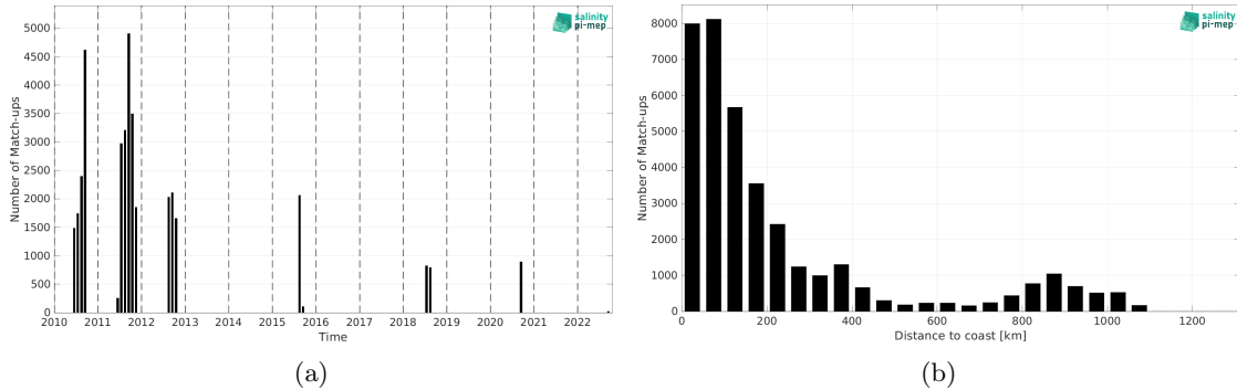
Figure 2: Number of match-ups between TSG (SAMOS) and SMOS SSS L4 v1 - Daily (CMEMS-CNR) SSS as a function of time (a) and as function of the distance to coast (b) over the Arctic Ocean Pi-MEP region and for the full satellite product period.
