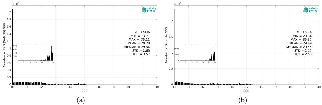
Figure 3: Histograms of SSS from TSG (SAMOS) (a) and SMOS SSS L4 v1 - Daily (CMEMS-CNR) (b) considering all match-up pairs per bins of 0.1 over the Arctic Ocean Pi-MEP region and for the full satellite product period.
