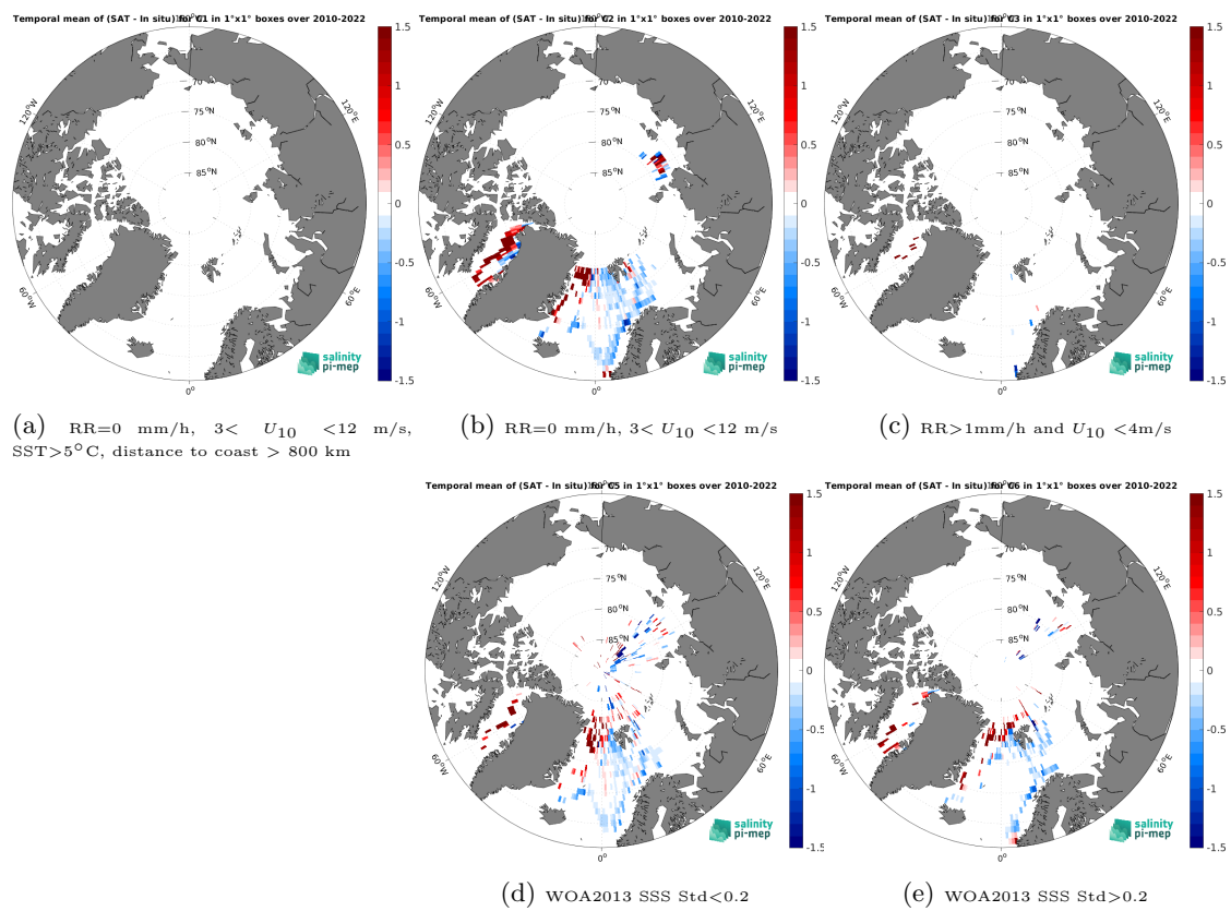
Figure 14: Temporal mean gridded over spatial boxes of size 1^\circ \times 1^\circ of \Delta SSS (SMOS SSS L4 v1 - Daily (CMEMS-CNR) - TSG (Polarstern)) for 5 different subdatasets corresponding to:RR=0 mm/h, 3 < U_{10} < 12 m/s, SST > 5°C, distance to coast > 800 km (a), RR=0 mm/h, 3 < U_{10} < 12 m/s (b), RR > 1mm/h and U_{10} < 4 m/s (c), WOA2013 SSS Std < 0.2 (d), WOA2013 SSS Std > 0.2 (e).
