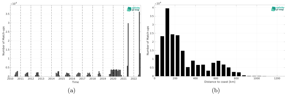
Figure 2: Number of match-ups between TSG (Polarstern) and SMOS SSS L4 v1 - Daily (CMEMS-CNR) SSS as a function of time (a) and as function of the distance to coast (b) over the Arctic Ocean Pi-MEP region and for the full satellite product period.
