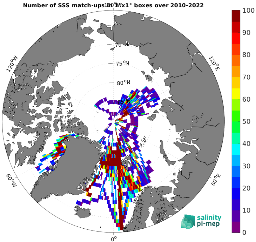
Figure 5: Number of SSS match-ups between TSG (Polarstern) SSS and the SMOS SSS L4 v1 - Daily (CMEMS-CNR) SSS product for the Arctic Ocean Pi-MEP region over 1^\circ \times 1^\circ boxes and for the full satellite product period.
