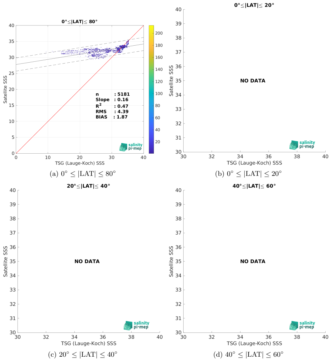
Figure 10: Contour maps of the concentration of SMOS SSS L4 v1 - Daily (CMEMS-CNR) SSS (y-axis) versus TSG (Lauge-Koch) SSS (x-axis) at match-up pairs for different latitude bands. For each plot, the red line shows x=y . The black thin and dashed lines indicate a linear fit through the data cloud and the \pm 95\% confidence levels, respectively. The number match-up pairs n , the slope and R^2 coefficient of the linear fit, the root mean square (RMS) and the mean bias between satellite and in situ data are indicated for each latitude band in each plots.
