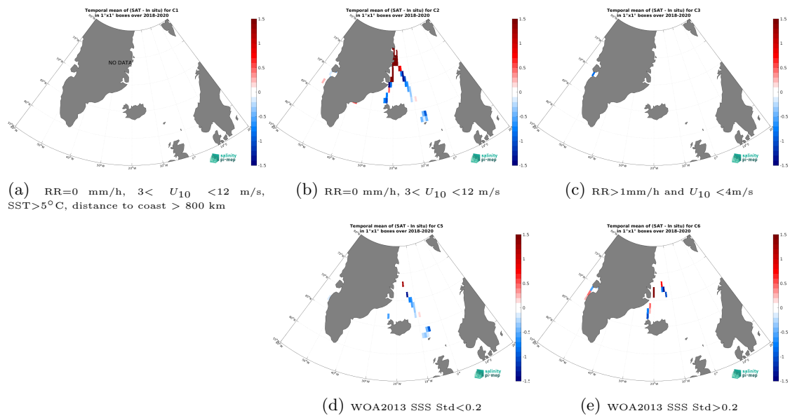
Figure 14: Temporal mean gridded over spatial boxes of size 1^\circ \times 1^\circ of \Delta SSS (SMOS SSS L4 v1 - Daily (CMEMS-CNR) - TSG (Lauge-Koch)) for 5 different subdatasets corresponding to: RR=0 mm/h, 3 < U_{10} < 12 m/s, SST > 5^\circ\text{C} , distance to coast > 800 km (a), RR=0 mm/h, 3 < U_{10} < 12 m/s (b), RR > 1 mm/h and U_{10} < 4 m/s (c), WOA2013 SSS Std < 0.2 (d), WOA2013 SSS Std > 0.2 (e).
