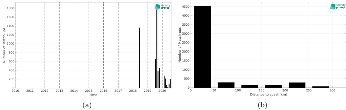
Figure 2: Number of match-ups between TSG (Lauge-Koch) and SMOS SSS L4 v1 - Daily (CMEMS-CNR) SSS as a function of time (a) and as function of the distance to coast (b) over the Arctic Ocean Pi-MEP region and for the full satellite product period.
