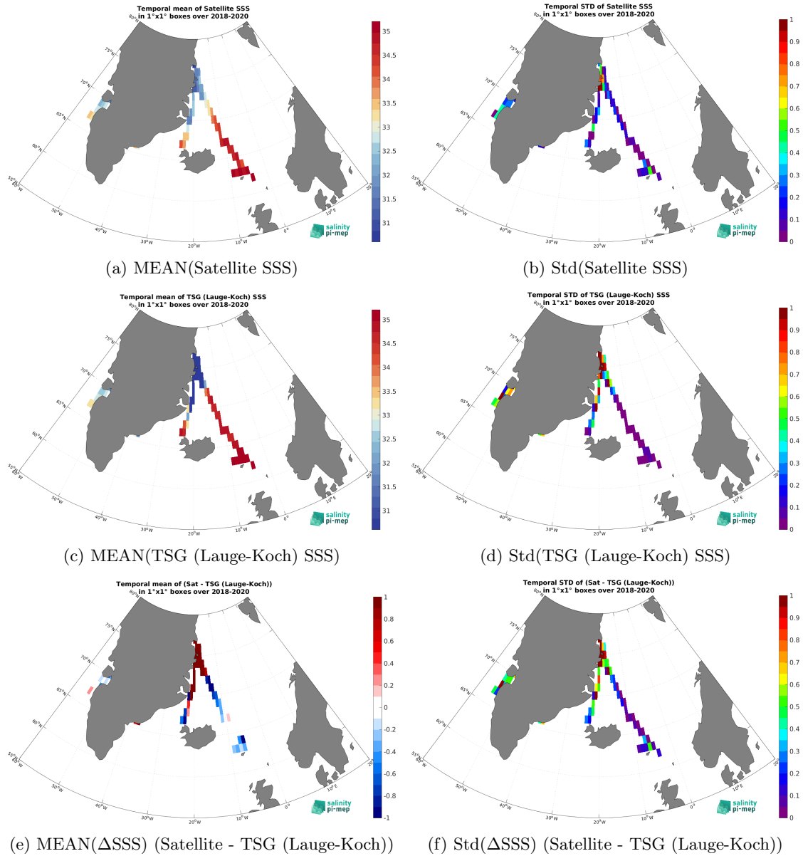
Figure 7: Temporal mean (left) and Std (right) of SSS from SMOS SSS L4 v1 - Daily (CMEMS-CNR) (top), TSG (Lauge-Koch) (middle), and of \Delta SSS (Satellite - TSG (Lauge-Koch)). Only match-up pairs are used to generate these maps.
