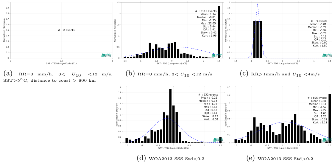
Figure 15: Normalized histogram of \Delta SSS (SMOS SSS L4 v1 - Daily (CMEMS-CNR) - TSG (Lauge-Koch)) for 5 different subdatasets corresponding to: RR=0 mm/h, 3 < U_{10} < 12 m/s, SST > 5°C, distance to coast > 800 km (a), RR=0 mm/h, 3 < U_{10} < 12 m/s (b), RR > 1mm/h and U_{10} < 4 m/s (c), WOA2013 SSS Std < 0.2 (d), WOA2013 SSS Std > 0.2 (e).
