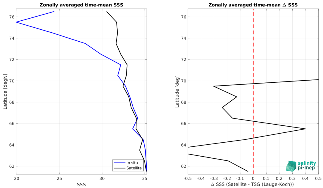
Figure 9: Left panel: Zonal mean SSS from SMOS SSS L4 v1 - Daily (CMEMS-CNR) satellite product (black) and from TSG (Lauge-Koch) (blue). Right panel: Zonal mean of \Delta SSS (Satellite - TSG (Lauge-Koch)) for all the collected Pi-MEP match-up pairs estimated over the full satellite product period.
