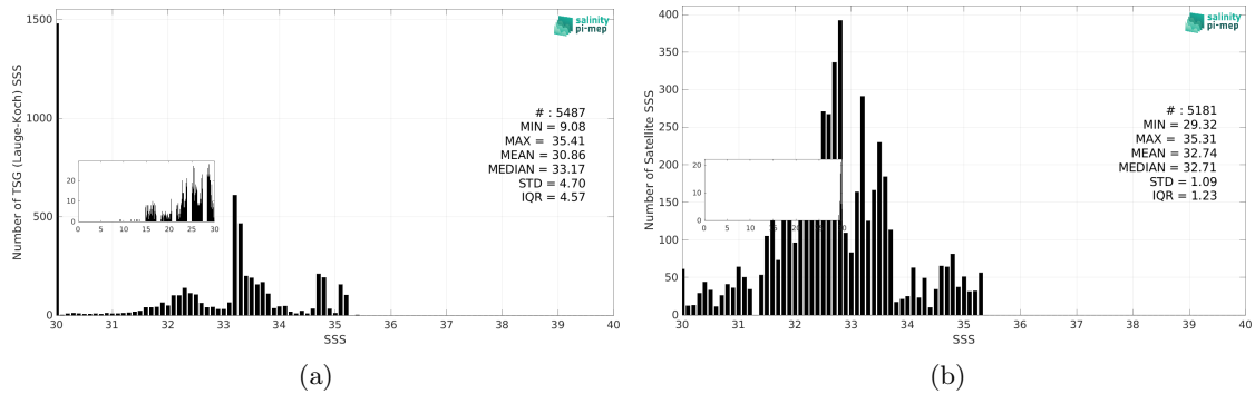
Figure 3: Histograms of SSS from TSG (Lauge-Koch) (a) and SMOS SSS L4 v1 - Daily (CMEMS-CNR) (b) considering all match-up pairs per bins of 0.1 over the Arctic Ocean Pi-MEP region and for the full satellite product period.
