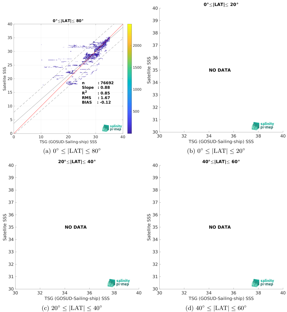
Figure 10: Contour maps of the concentration of SMOS SSS L4 v1 - Daily (CMEMS-CNR) SSS (y-axis) versus TSG (GOSUD-Sailing-ship) SSS (x-axis) at match-up pairs for different latitude bands. For each plot, the red line shows x=y . The black thin and dashed lines indicate a linear fit through the data cloud and the \pm 95\% confidence levels, respectively. The number match-up pairs n , the slope and R^2 coefficient of the linear fit, the root mean square (RMS) and the mean bias between satellite and in situ data are indicated for each latitude band in each plots.
