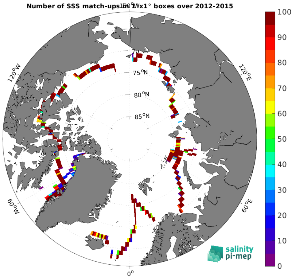
Figure 5: Number of SSS match-ups between TSG (GOSUD-Sailing-ship) SSS and the SMOS SSS L4 v1 - Daily (CMEMS-CNR) SSS product for the Arctic Ocean Pi-MEP region over 1^\circ \times 1^\circ boxes and for the full satellite product period.
