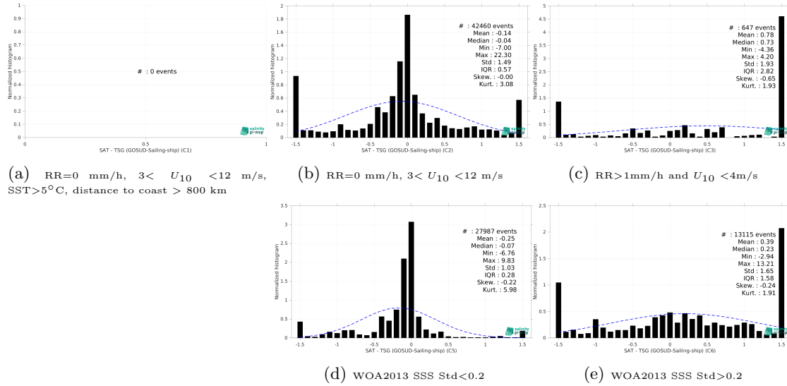
Figure 15: Normalized histogram of \Delta SSS (SMOS SSS L4 v1 - Daily (CMEMS-CNR) - TSG (GOSUD-Sailing-ship)) for 5 different subdatasets corresponding to: RR=0 mm/h, 3 < U_{10} < 12 m/s, SST > 5°C, distance to coast > 800 km (a), RR=0 mm/h, 3 < U_{10} < 12 m/s (b), RR > 1mm/h and U_{10} < 4 m/s (c), WOA2013 SSS Std < 0.2 (d), WOA2013 SSS Std > 0.2 (e).
