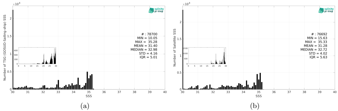
Figure 3: Histograms of SSS from TSG (GOSUD-Sailing-ship) (a) and SMOS SSS L4 v1 - Daily (CMEMS-CNR) (b) considering all match-up pairs per bins of 0.1 over the Arctic Ocean Pi-MEP region and for the full satellite product period.
