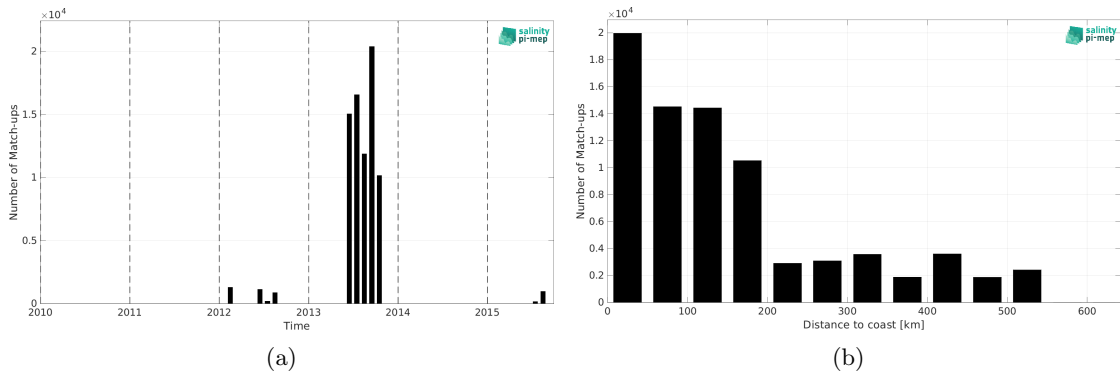
Figure 2: Number of match-ups between TSG (GOSUD-Sailing-ship) and SMOS SSS L4 v1 - Daily (CMEMS-CNR) SSS as a function of time (a) and as function of the distance to coast (b) over the Arctic Ocean Pi-MEP region and for the full satellite product period.
