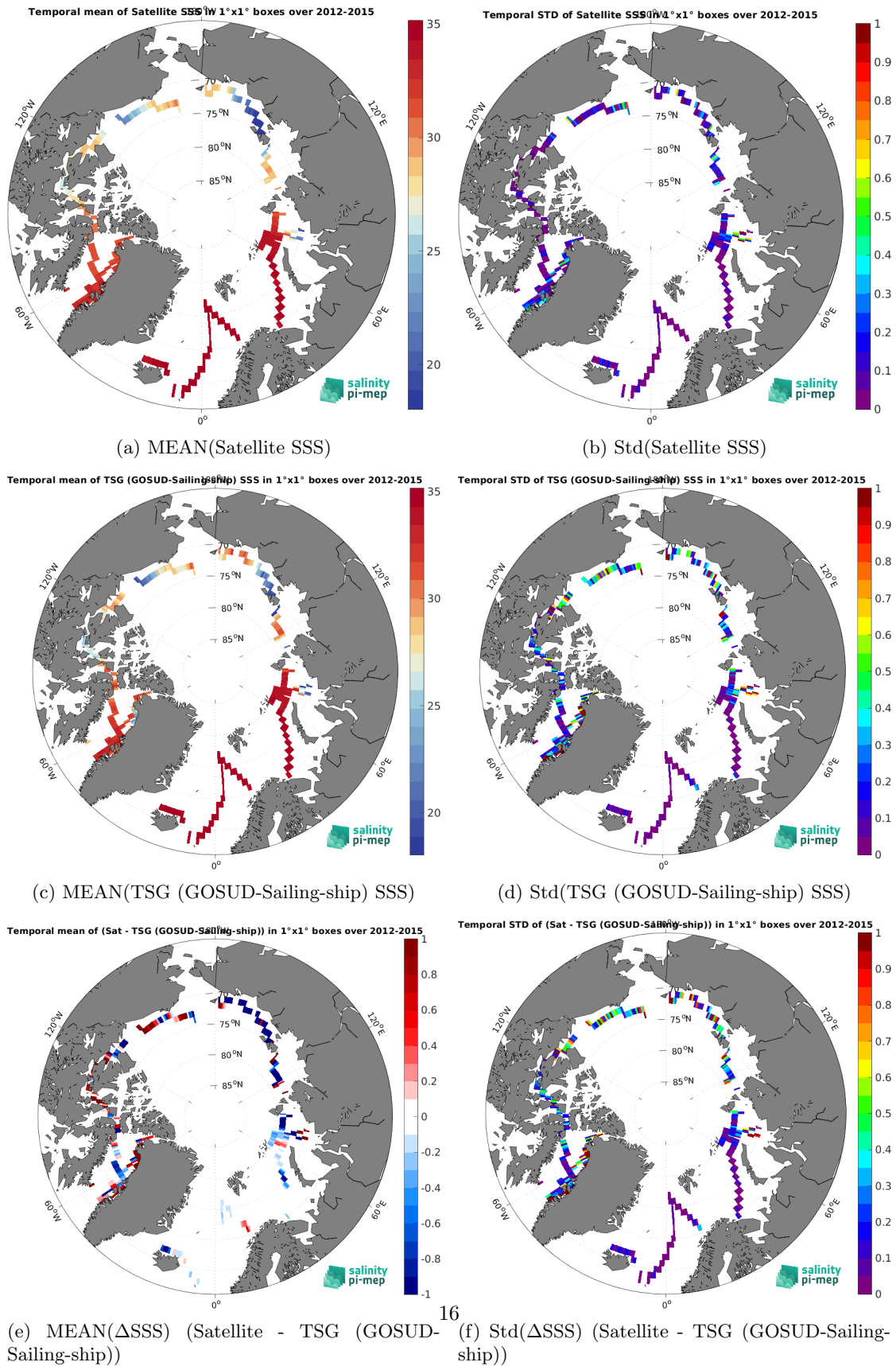
Figure 7: Temporal mean (left) and Std (right) of SSS from SMOS SSS L4 v1 - Daily (CMEMS-CNR) (top), TSG (GOSUD-Sailing-ship) (middle), and of \Delta SSS (Satellite - TSG (GOSUD-Sailing-ship)). Only match-up pairs are used to generate these maps.
