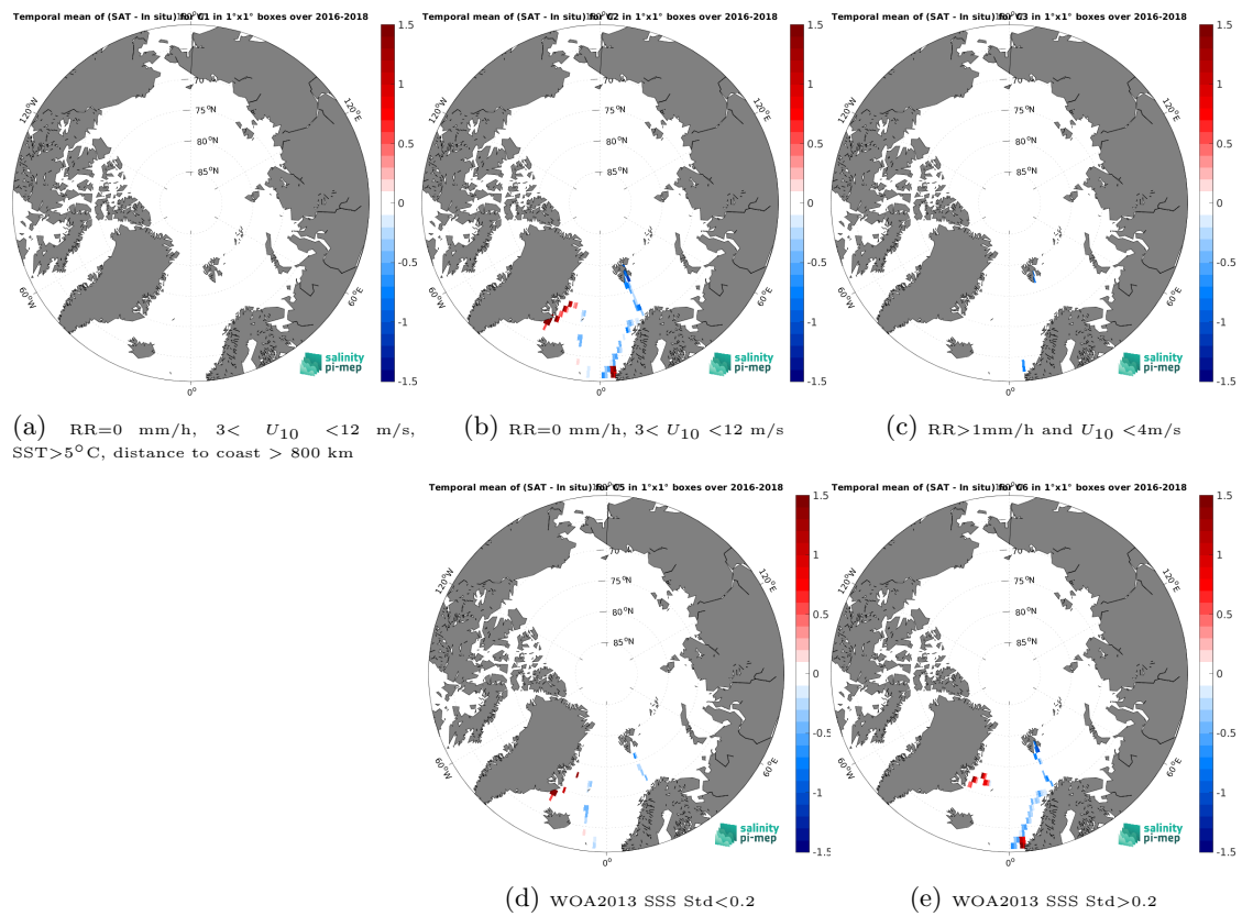
Figure 14: Temporal mean gridded over spatial boxes of size 1^\circ \times 1^\circ of \Delta SSS (SMOS SSS L4 v1 - Daily (CMEMS-CNR) - TSG (GOSUD-Research-vessel)) for 5 different subdatasets corresponding to:RR=0 mm/h, 3 < U_{10} < 12 m/s, SST >5^\circ C, distance to coast > 800 km (a), RR=0 mm/h, 3 < U_{10} < 12 m/s (b), RR >1 mm/h and U_{10} < 4 m/s (c), WOA2013 SSS Std <0.2 (d), WOA2013 SSS Std >0.2 (e).
