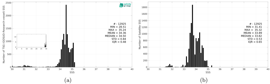
Figure 3: Histograms of SSS from TSG (GOSUD-Research-vessel) (a) and SMOS SSS L4 v1 - Daily (CMEMS-CNR) (b) considering all match-up pairs per bins of 0.1 over the Arctic Ocean Pi-MEP region and for the full satellite product period.
