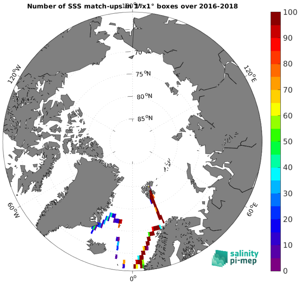
Figure 5: Number of SSS match-ups between TSG (GOSUD-Research-vessel) SSS and the SMOS SSS L4 v1 - Daily (CMEMS-CNR) SSS product for the Arctic Ocean Pi-MEP region over 1^\circ \times 1^\circ boxes and for the full satellite product period.
