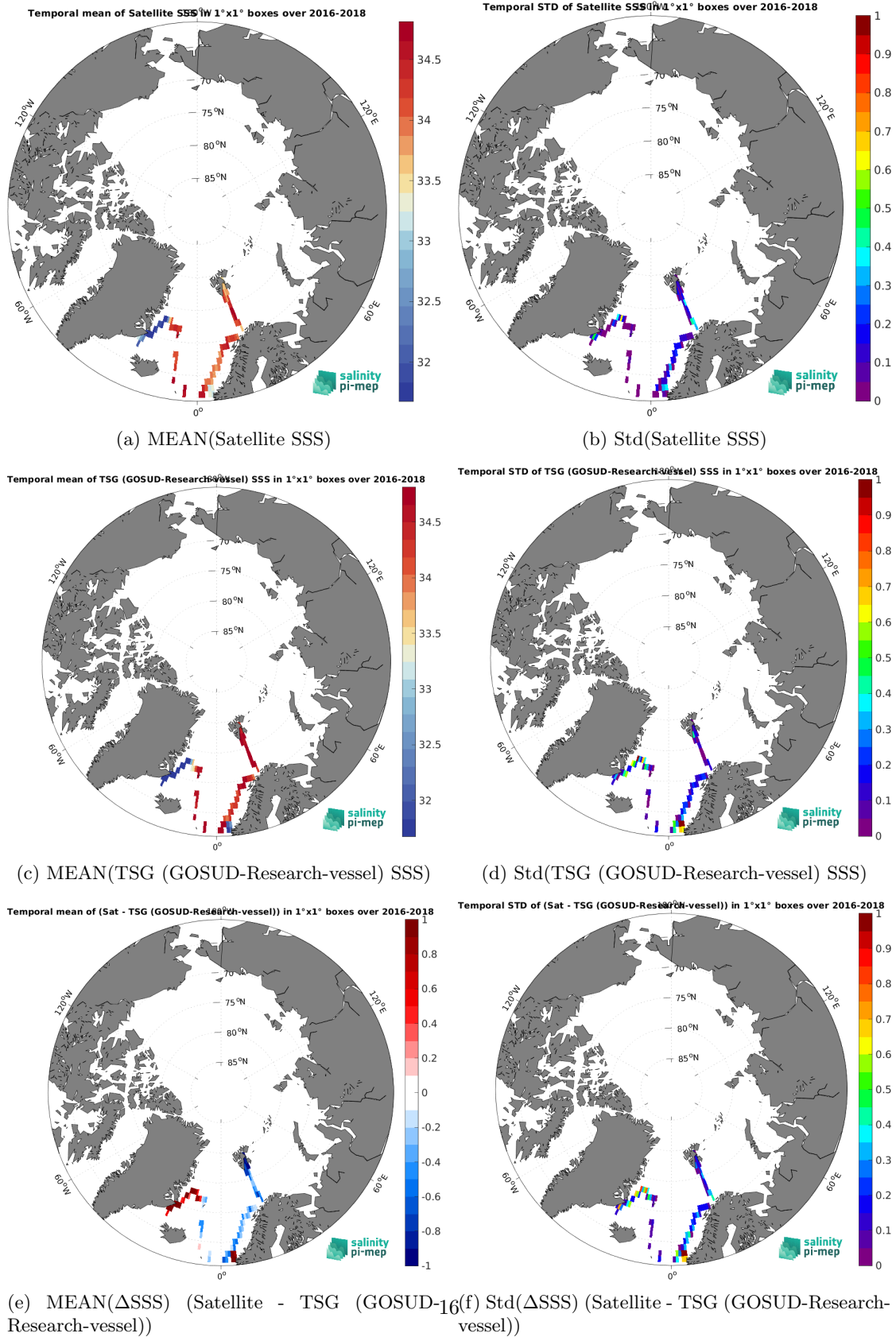
Figure 7: Temporal mean (left) and Std (right) of SSS from SMOS SSS L4 v1 - Daily (CMEMS-CNR) (top), TSG (GOSUD-Research-vessel) (middle), and of \Delta SSS (Satellite - TSG (GOSUD-Research-vessel)). Only match-up pairs are used to generate these maps.
