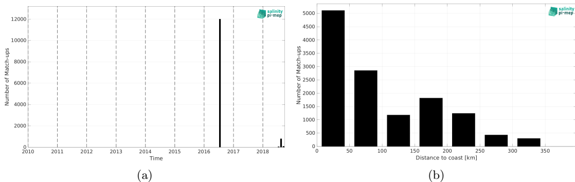
Figure 2: Number of match-ups between TSG (GOSUD-Research-vessel) and SMOS SSS L4 v1 - Daily (CMEMS-CNR) SSS as a function of time (a) and as function of the distance to coast (b) over the Arctic Ocean Pi-MEP region and for the full satellite product period.
