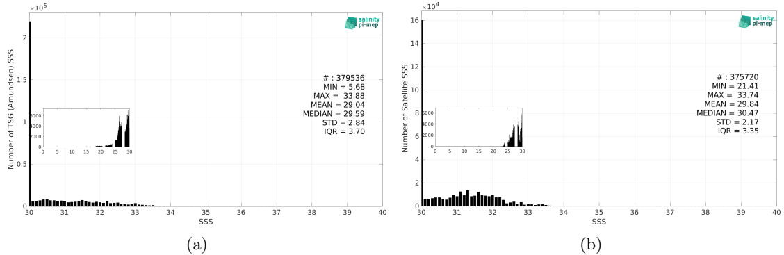
Figure 3: Histograms of SSS from TSG (Amundsen) (a) and SMOS SSS L4 v1 - Daily (CMEMS-CNR) (b) considering all match-up pairs per bins of 0.1 over the Arctic Ocean Pi-MEP region and for the full satellite product period.
