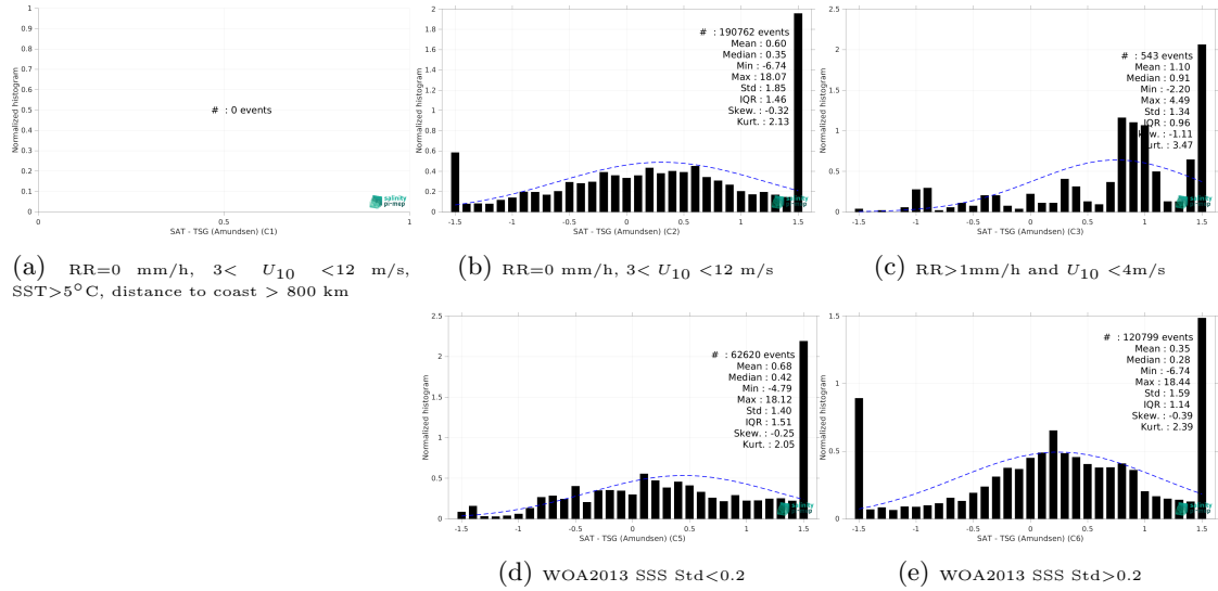
Figure 15: Normalized histogram of \Delta SSS (SMOS SSS L4 v1 - Daily (CMEMS-CNR) - TSG (Amundsen)) for 5 different subdatasets corresponding to: RR=0 mm/h, 3 < U_{10} < 12 m/s, SST > 5°C, distance to coast > 800 km (a), RR=0 mm/h, 3 < U_{10} < 12 m/s (b), RR > 1mm/h and U_{10} < 4 m/s (c), WOA2013 SSS Std < 0.2 (d), WOA2013 SSS Std > 0.2 (e).
