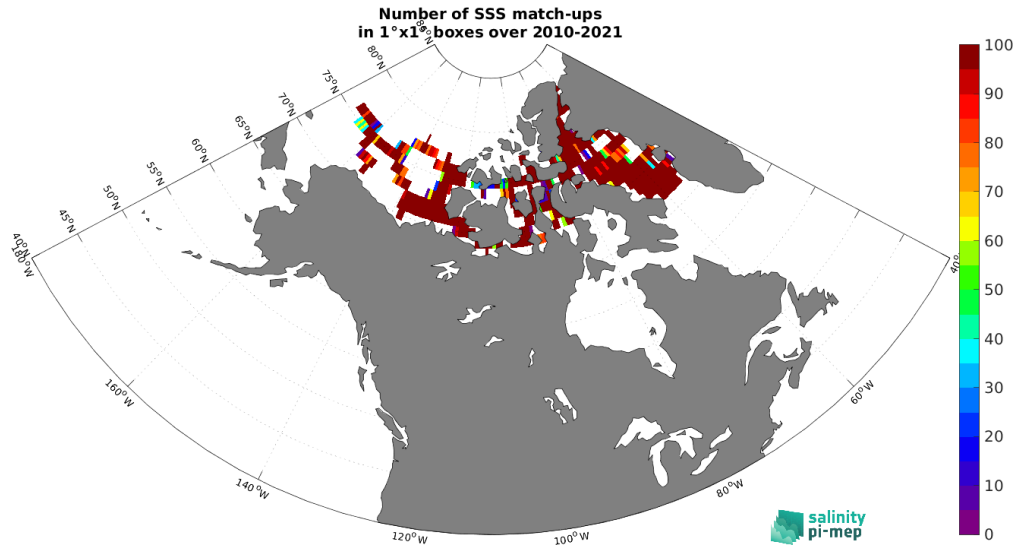
Figure 5: Number of SSS match-ups between TSG (Amundsen) SSS and the SMOS SSS L4 v1 - Daily (CMEMS-CNR) SSS product for the Arctic Ocean Pi-MEP region over 1^\circ \times 1^\circ boxes and for the full satellite product period.
