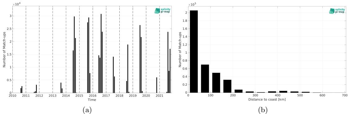
Figure 2: Number of match-ups between TSG (Amundsen) and SMOS SSS L4 v1 - Daily (CMEMS-CNR) SSS as a function of time (a) and as function of the distance to coast (b) over the Arctic Ocean Pi-MEP region and for the full satellite product period.
