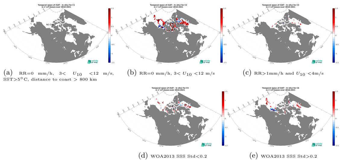
Figure 14: Temporal mean gridded over spatial boxes of size 1^\circ \times 1^\circ of \Delta SSS (SMOS SSS L4 v1 - Daily (CMEMS-CNR) - TSG (Amundsen)) for 5 different subdatasets corresponding to: RR=0 mm/h, 3 < U_{10} < 12 m/s, SST > 5°C, distance to coast > 800 km (a), RR=0 mm/h, 3 < U_{10} < 12 m/s (b), RR > 1mm/h and U_{10} < 4 m/s (c), WOA2013 SSS Std < 0.2 (d), WOA2013 SSS Std > 0.2 (e).
