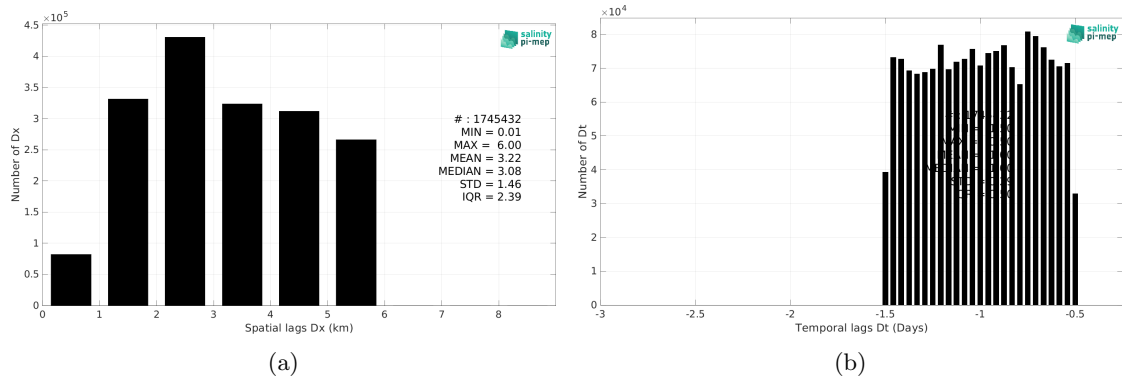
Figure 6: Histograms of the spatial (a) and temporal (b) lags between the location/time of the SASSIE measurement and the date of the corresponding SMOS SSS L4 v1 - Daily (CMEMS-CNR) SSS pixel.
