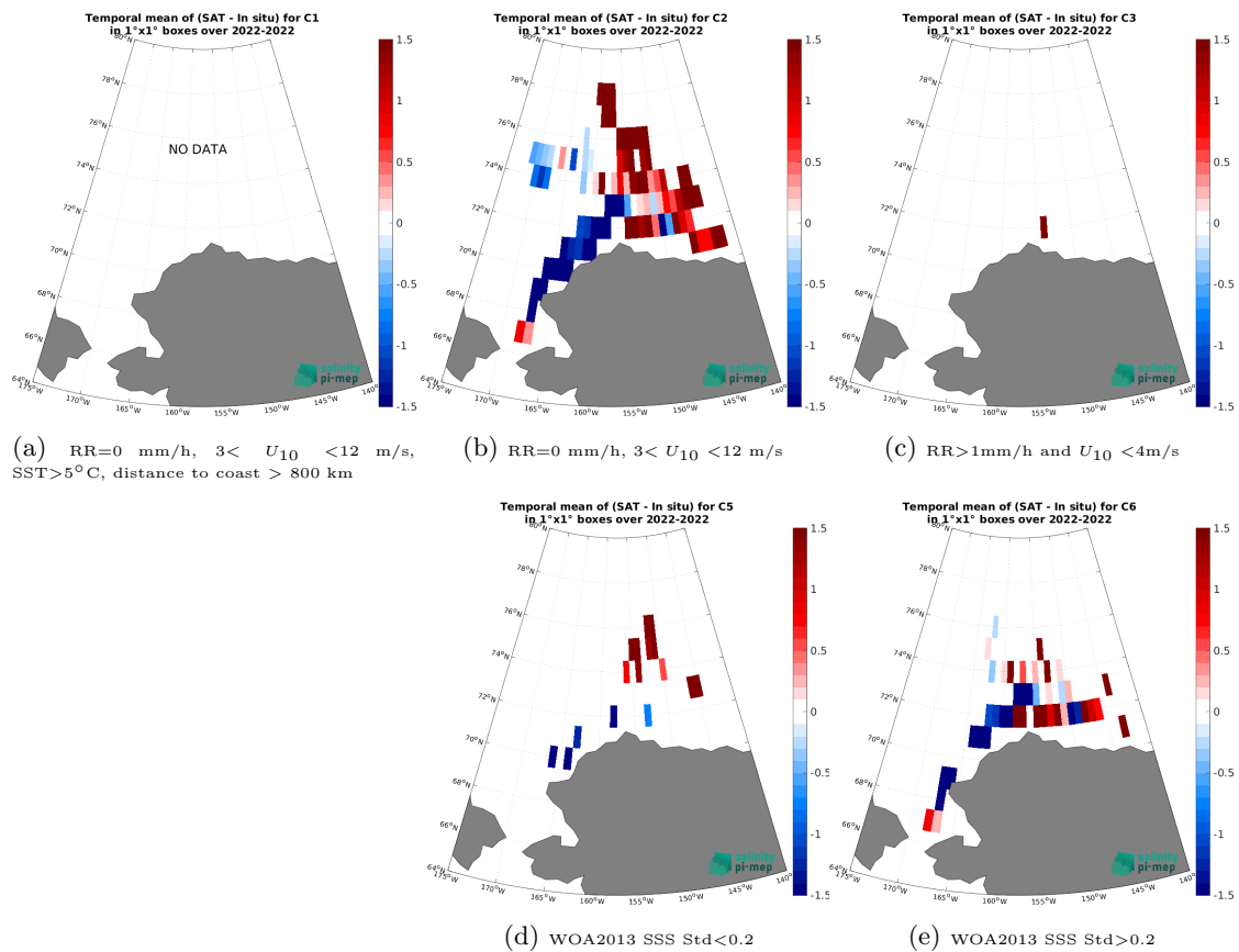
Figure 14: Temporal mean gridded over spatial boxes of size 1^\circ \times 1^\circ of \Delta\text{SSS} (SMOS SSS L4 v1 - Daily (CMEMS-CNR) - SASSIE) for 5 different subdatasets corresponding to:RR=0 mm/h, 3 < U_{10} < 12 m/s, SST>5°C, distance to coast > 800 km (a), RR=0 mm/h, 3 < U_{10} < 12 m/s (b), RR>1mm/h and U_{10} < 4 m/s (c), WOA2013 SSS Std<0.2 (d), WOA2013 SSS Std>0.2 (e).
