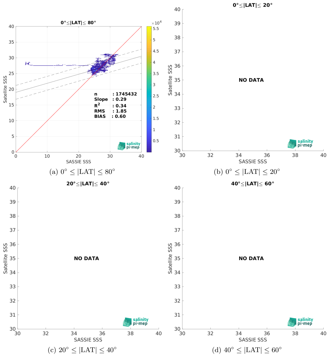
Figure 10: Contour maps of the concentration of SMOS SSS L4 v1 - Daily (CMEMS-CNR) SSS (y-axis) versus SASSIE SSS (x-axis) at match-up pairs for different latitude bands. For each plot, the red line shows x=y . The black thin and dashed lines indicate a linear fit through the data cloud and the \pm 95\% confidence levels, respectively. The number match-up pairs n , the slope and R^2 coefficient of the linear fit, the root mean square (RMS) and the mean bias between satellite and in situ data are indicated for each latitude band in each plots.
