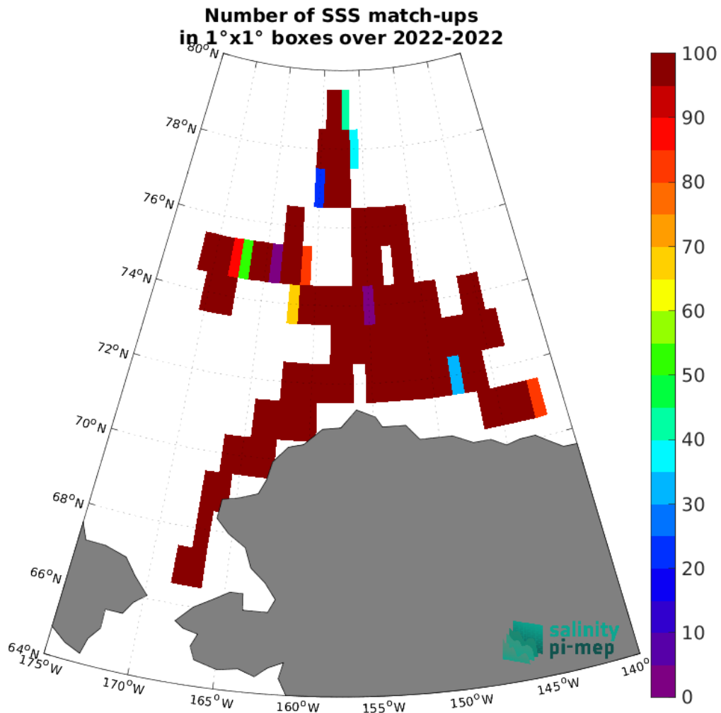
Figure 5: Number of SSS match-ups between SASSIE SSS and the SMOS SSS L4 v1 - Daily (CMEMS-CNR) SSS product for the Arctic Ocean Pi-MEP region over 1^\circ \times 1^\circ boxes and for the full satellite product period.
