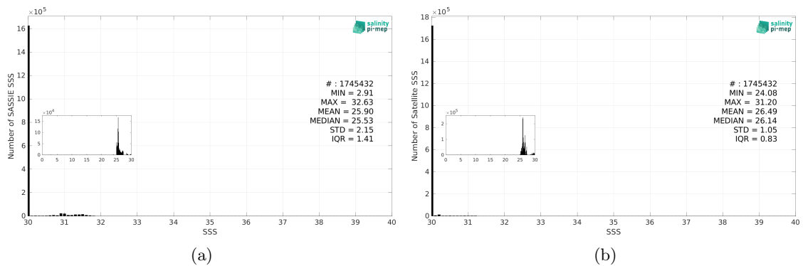
Figure 3: Histograms of SSS from SASSIE (a) and SMOS SSS L4 v1 - Daily (CMEMS-CNR) (b) considering all match-up pairs per bins of 0.1 over the Arctic Ocean Pi-MEP region and for the full satellite product period.
