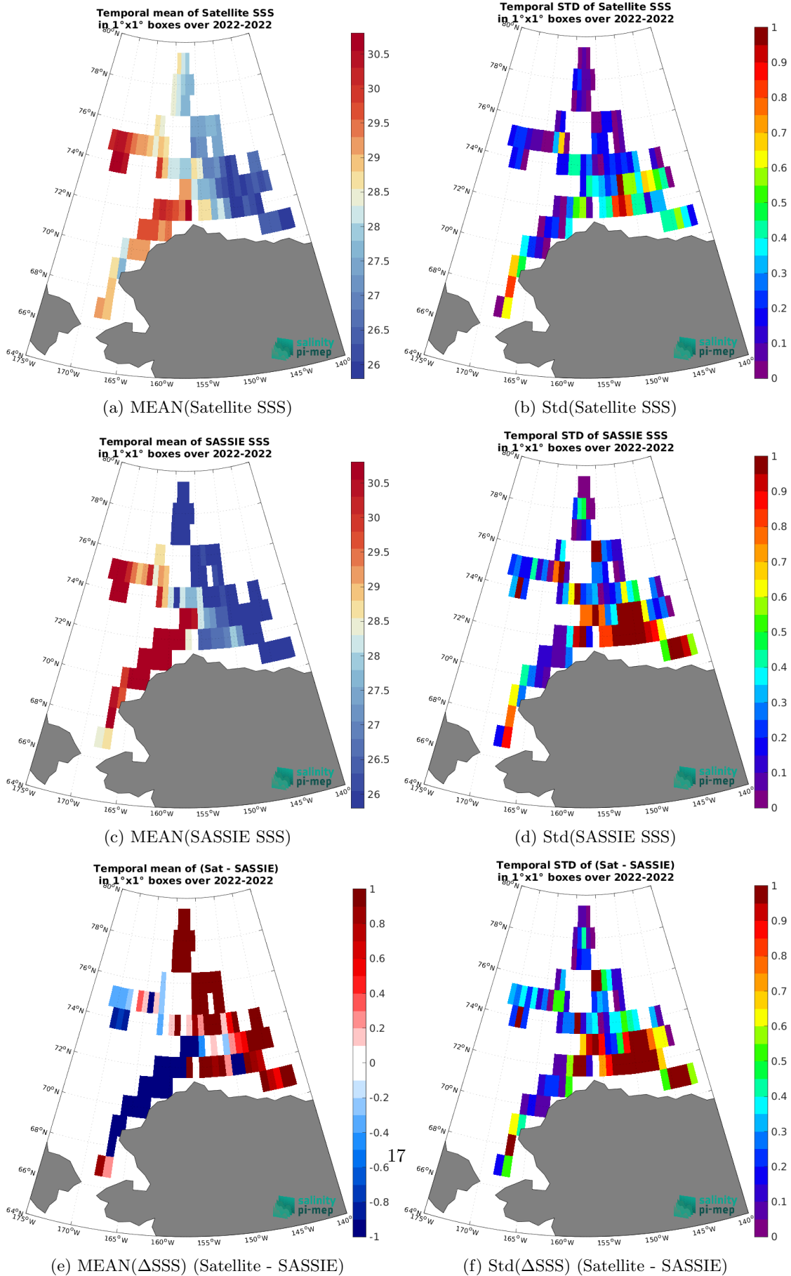
Figure 7: Temporal mean (left) and Std (right) of SSS from SMOS SSS L4 v1 - Daily (CMEMS-CNR) (top), SASSIE (middle), and of \Delta SSS (Satellite - SASSIE). Only match-up pairs are used to generate these maps.
