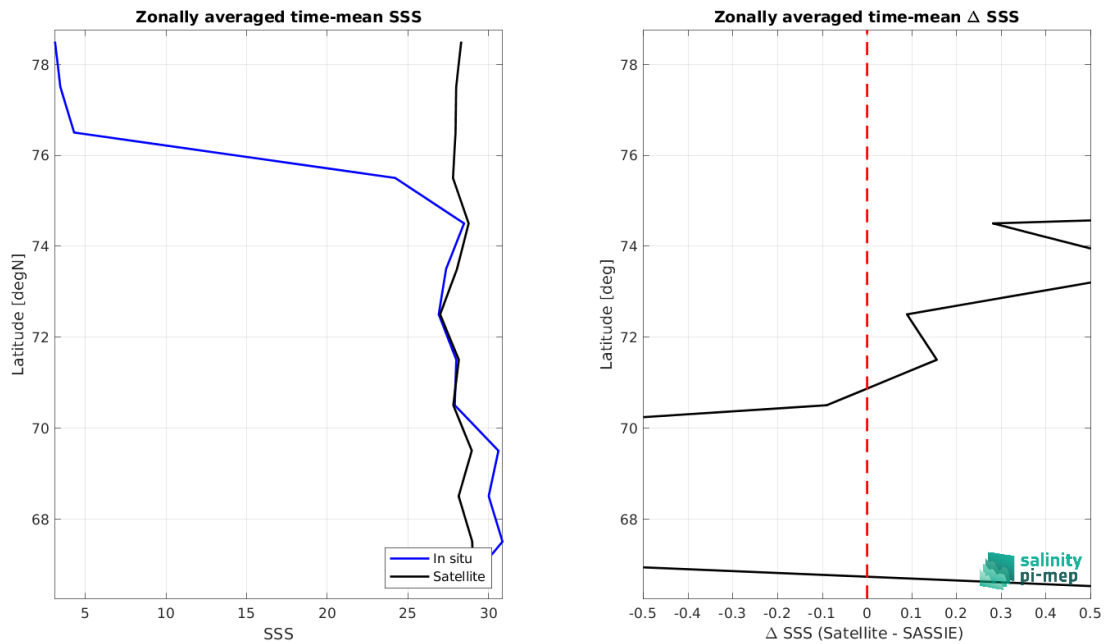
Figure 9: Left panel: Zonal mean SSS from SMOS SSS L4 v1 - Daily (CMEMS-CNR) satellite product (black) and from SASSIE (blue). Right panel: Zonal mean of \Delta SSS (Satellite - SASSIE) for all the collected Pi-MEP match-up pairs estimated over the full satellite product period.
