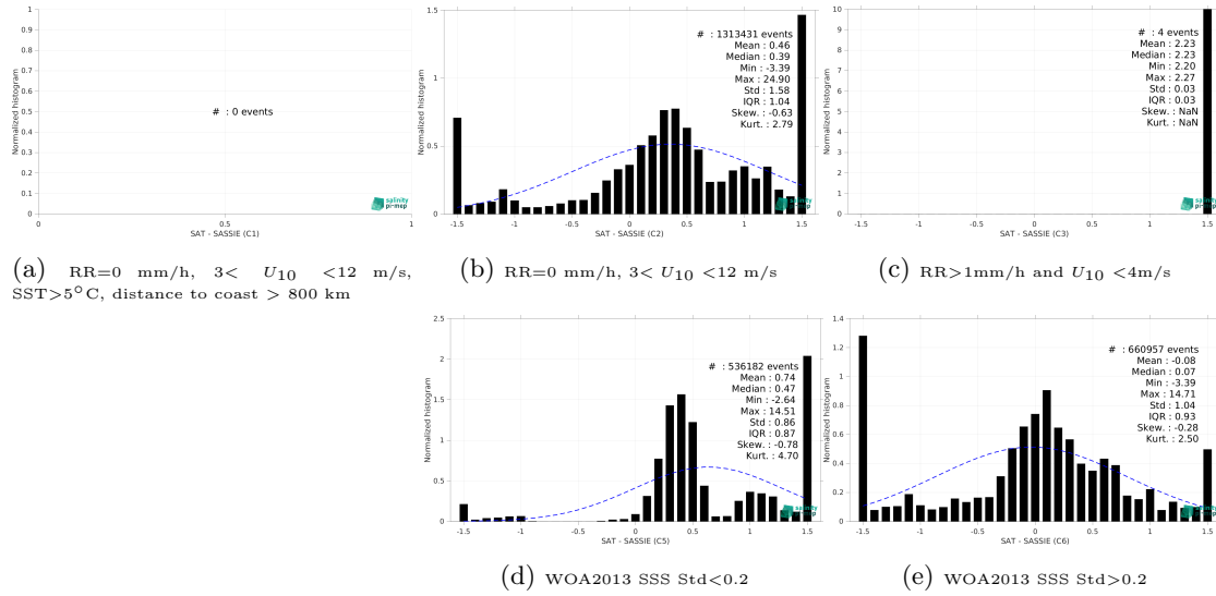
Figure 15: Normalized histogram of \Delta SSS (SMOS SSS L4 v1 - Daily (CMEMS-CNR) - SASSIE) for 5 different subdatasets corresponding to: RR=0 mm/h, 3 < U_{10} < 12 m/s, SST>5°C, distance to coast > 800 km (a), RR=0 mm/h, 3 < U_{10} < 12 m/s (b), RR>1mm/h and U_{10} < 4 m/s (c), WOA2013 SSS Std<0.2 (d), WOA2013 SSS Std>0.2 (e).
