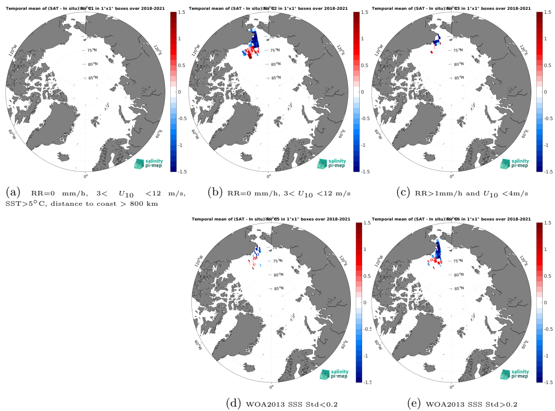
Figure 14: Temporal mean gridded over spatial boxes of size 1^\circ \times 1^\circ of \Delta SSS (SMOS SSS L4 v1 - Daily (CMEMS-CNR) - Saildrone) for 5 different subdatasets corresponding to:RR=0 mm/h, 3 < U_{10} < 12 m/s, SST > 5^\circ\text{C} , distance to coast > 800 km (a), RR=0 mm/h, 3 < U_{10} < 12 m/s (b), RR > 1 mm/h and U_{10} < 4 m/s (c), WOA2013 SSS Std < 0.2 (d), WOA2013 SSS Std > 0.2 (e).
