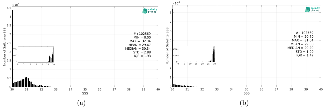
Figure 3: Histograms of SSS from Saildrone (a) and SMOS SSS L4 v1 - Daily (CMEMS-CNR) (b) considering all match-up pairs per bins of 0.1 over the Arctic Ocean Pi-MEP region and for the full satellite product period.
