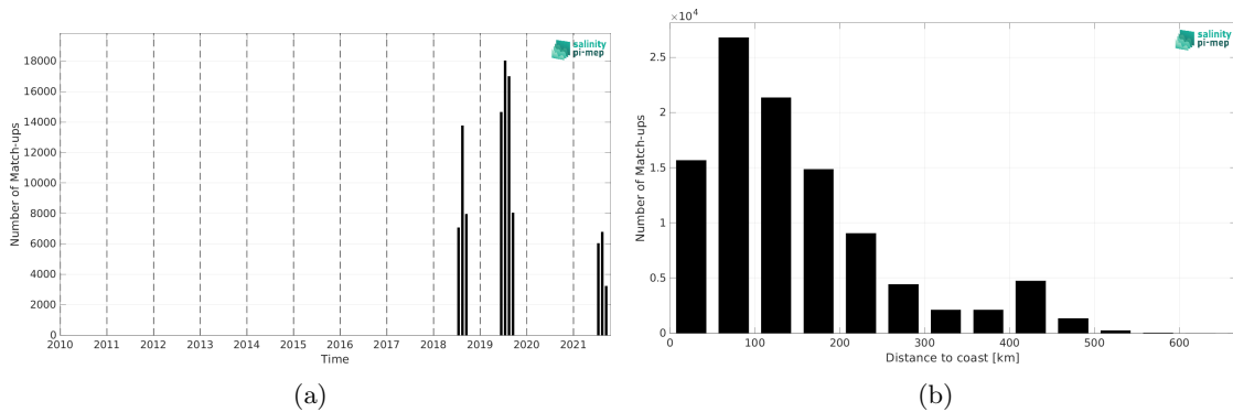
Figure 2: Number of match-ups between Saildrone and SMOS SSS L4 v1 - Daily (CMEMS-CNR) SSS as a function of time (a) and as function of the distance to coast (b) over the Arctic Ocean Pi-MEP region and for the full satellite product period.
