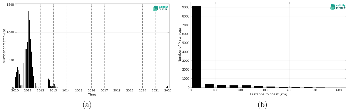
Figure 2: Number of match-ups between Marine mammals and SMOS SSS L4 v1 - Daily (CMEMS-CNR) SSS as a function of time (a) and as function of the distance to coast (b) over the Arctic Ocean Pi-MEP region and for the full satellite product period.
