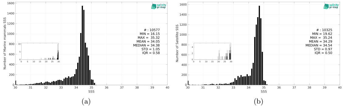
Figure 3: Histograms of SSS from Marine mammals (a) and SMOS SSS L4 v1 - Daily (CMEMS-CNR) (b) considering all match-up pairs per bins of 0.1 over the Arctic Ocean Pi-MEP region and for the full satellite product period.
