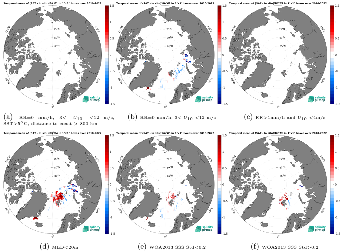
Figure 14: Temporal mean gridded over spatial boxes of size 1^\circ \times 1^\circ of \Delta SSS (SMOS SSS L4 v1 - Daily (CMEMS-CNR) - Marine mammals) for 6 different subdatasets corresponding to:RR=0 mm/h, 3 < U_{10} < 12 m/s, SST > 5°C, distance to coast > 800 km (a), RR=0 mm/h, 3 < U_{10} < 12 m/s (b), RR > 1mm/h and U_{10} < 4 m/s (c),MLD < 20m (d),WOA2013 SSS Std < 0.2 (e),WOA2013 SSS Std > 0.2 (f).
