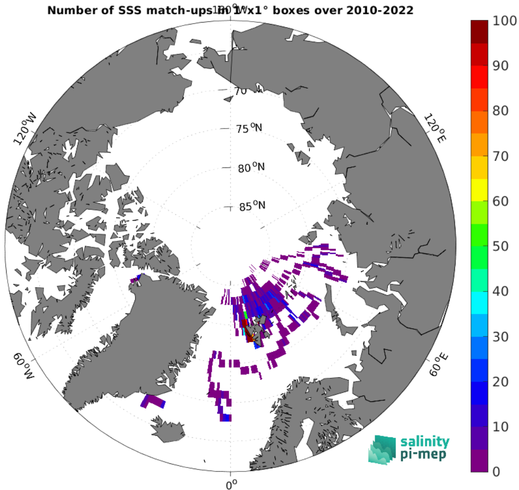
Figure 5: Number of SSS match-ups between Marine mammals SSS and the SMOS SSS L4 v1 - Daily (CMEMS-CNR) SSS product for the Arctic Ocean Pi-MEP region over 1^\circ \times 1^\circ boxes and for the full satellite product period.
