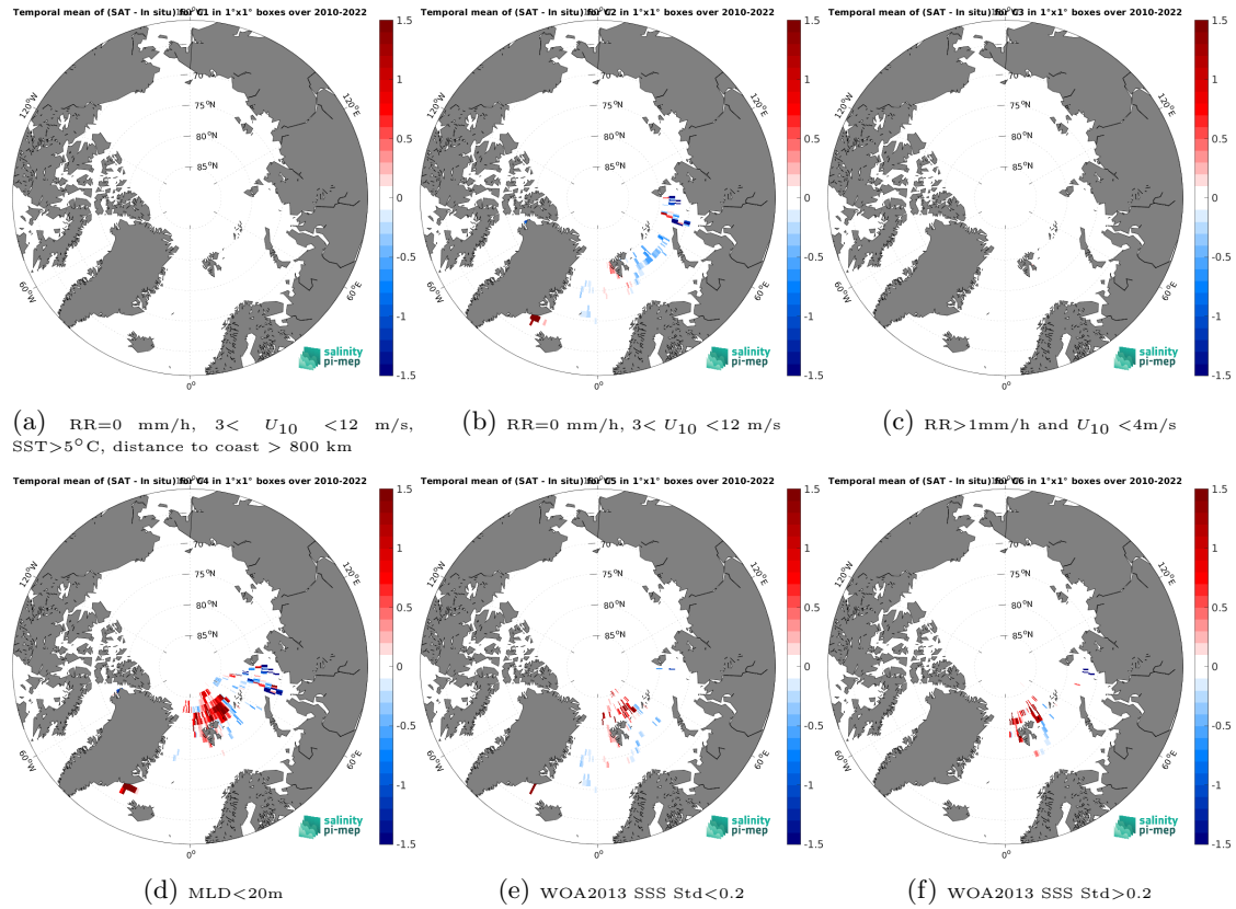
Figure 14: Temporal mean gridded over spatial boxes of size 1^\circ \times 1^\circ of \Delta\text{SSS} (SMOS SSS L4 v1 - Daily (CMEMS-CNR) - Marine mammals) for 6 different subdatasets corresponding to: RR=0 mm/h, 3 < U_{10} < 12 m/s, SST > 5°C, distance to coast > 800 km (a), RR=0 mm/h, 3 < U_{10} < 12 m/s (b), RR > 1mm/h and U_{10} < 4 m/s (c), MLD < 20m (d), WOA2013 SSS Std < 0.2 (e), WOA2013 SSS Std > 0.2 (f).
