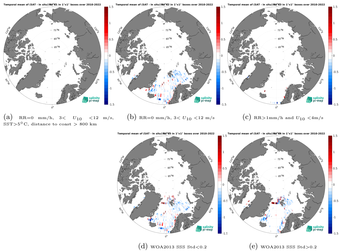
Figure 14: Temporal mean gridded over spatial boxes of size 1^\circ \times 1^\circ of \Delta SSS (SMOS SSS L4 v1 - Daily (CMEMS-CNR) - ICES) for 5 different subdatasets corresponding to:RR=0 mm/h, 3 < U_{10} < 12 m/s, SST>5°C, distance to coast > 800 km (a), RR=0 mm/h, 3 < U_{10} < 12 m/s (b), RR>1mm/h and U_{10} < 4 m/s (c), WOA2013 SSS Std<0.2 (d), WOA2013 SSS Std>0.2 (e).
