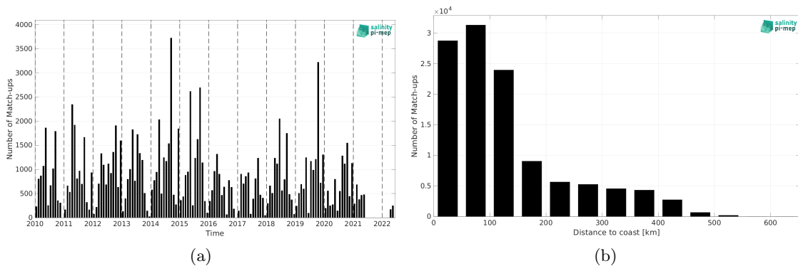
Figure 2: Number of match-ups between ICES and SMOS SSS L4 v1 - Daily (CMEMS-CNR) SSS as a function of time (a) and as function of the distance to coast (b) over the Arctic Ocean Pi-MEP region and for the full satellite product period.
