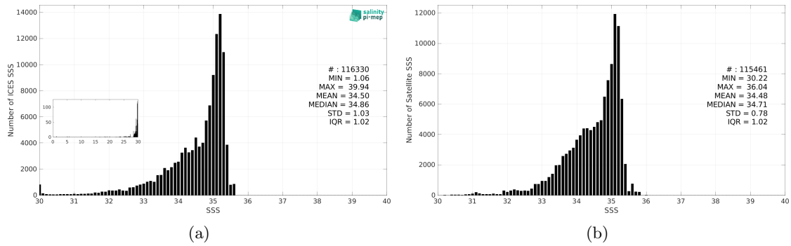
Figure 3: Histograms of SSS from ICES (a) and SMOS SSS L4 v1 - Daily (CMEMS-CNR) (b) considering all match-up pairs per bins of 0.1 over the Arctic Ocean Pi-MEP region and for the full satellite product period.
