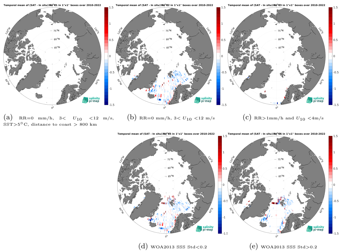
Figure 14: Temporal mean gridded over spatial boxes of size 1^\circ \times 1^\circ of \Delta\text{SSS} (SMOS SSS L4 v1 - Daily (CMEMS-CNR) - ICES) for 5 different subdatasets corresponding to: RR=0 mm/h, 3 < U_{10} < 12 m/s, SST > 5°C, distance to coast > 800 km (a), RR=0 mm/h, 3 < U_{10} < 12 m/s (b), RR > 1mm/h and U_{10} < 4 m/s (c), WOA2013 SSS Std < 0.2 (d), WOA2013 SSS Std > 0.2 (e).
