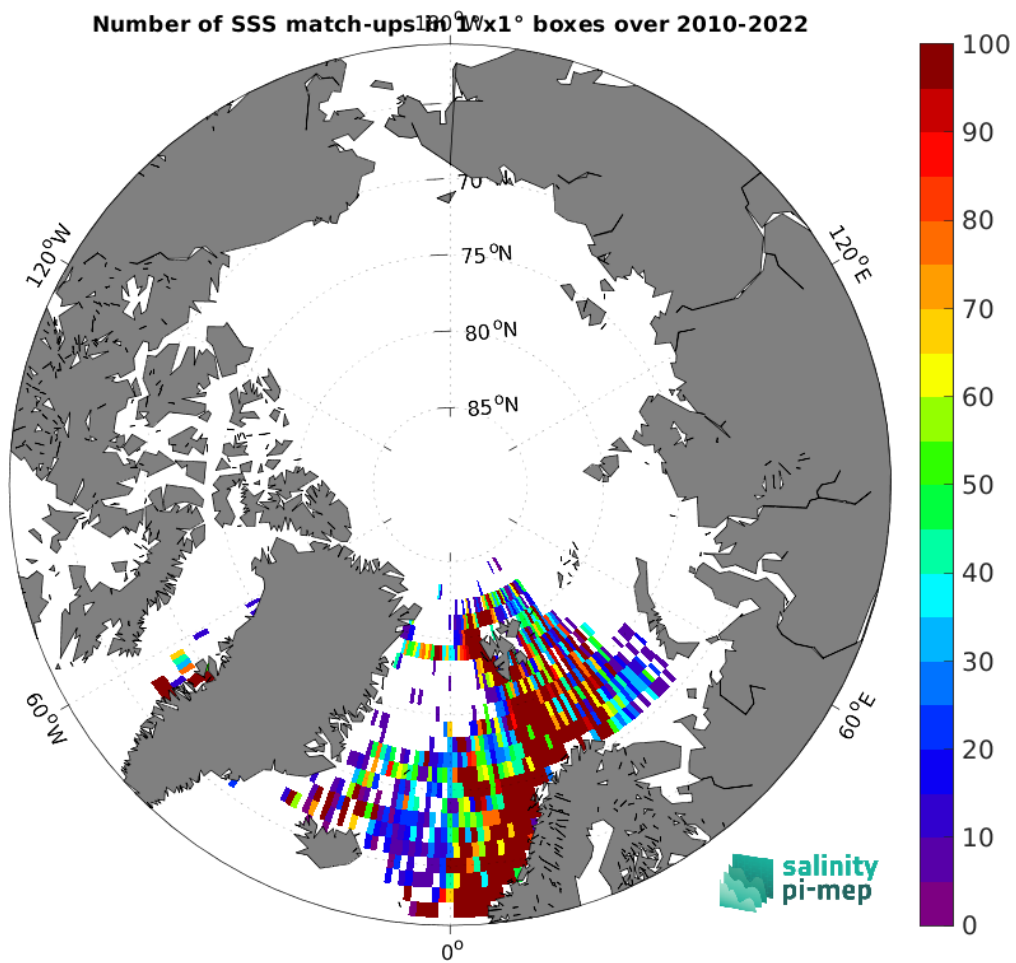
Figure 5: Number of SSS match-ups between ICES SSS and the SMOS SSS L4 v1 - Daily (CMEMS-CNR) SSS product for the Arctic Ocean Pi-MEP region over 1^\circ \times 1^\circ boxes and for the full satellite product period.
