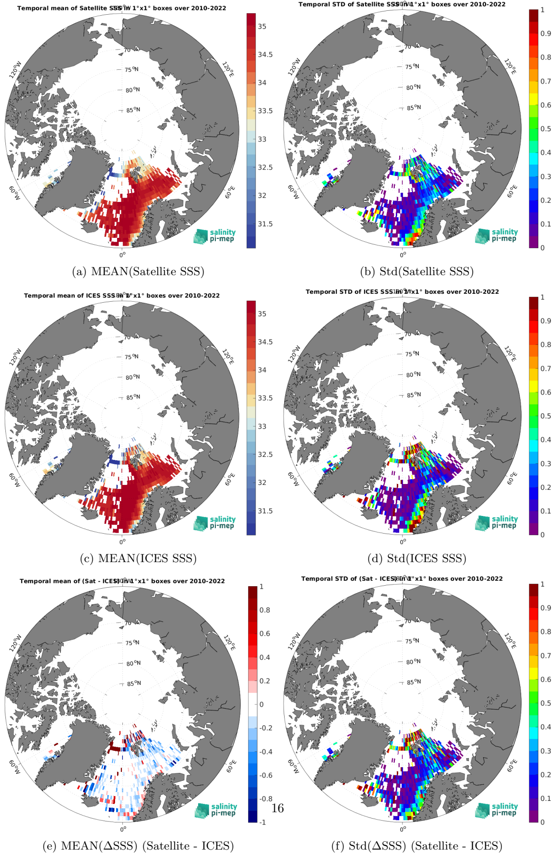
Figure 7: Temporal mean (left) and Std (right) of SSS from SMOS SSS L4 v1 - Daily (CMEMS-CNR) (top), ICES (middle), and of \Delta SSS (Satellite - ICES). Only match-up pairs are used to generate these maps.
