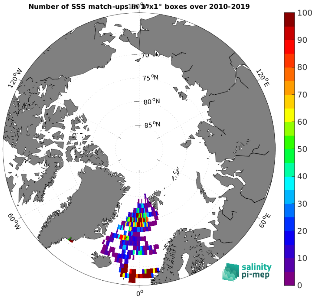
Figure 4: Number of SSS match-ups between Surface drifters SSS and the SMOS SSS L4 v1 - Daily (CMEMS-CNR) SSS product for the Arctic Ocean Pi-MEP region over 1^{\circ} \times 1^{\circ} boxes and for the full satellite product period.
